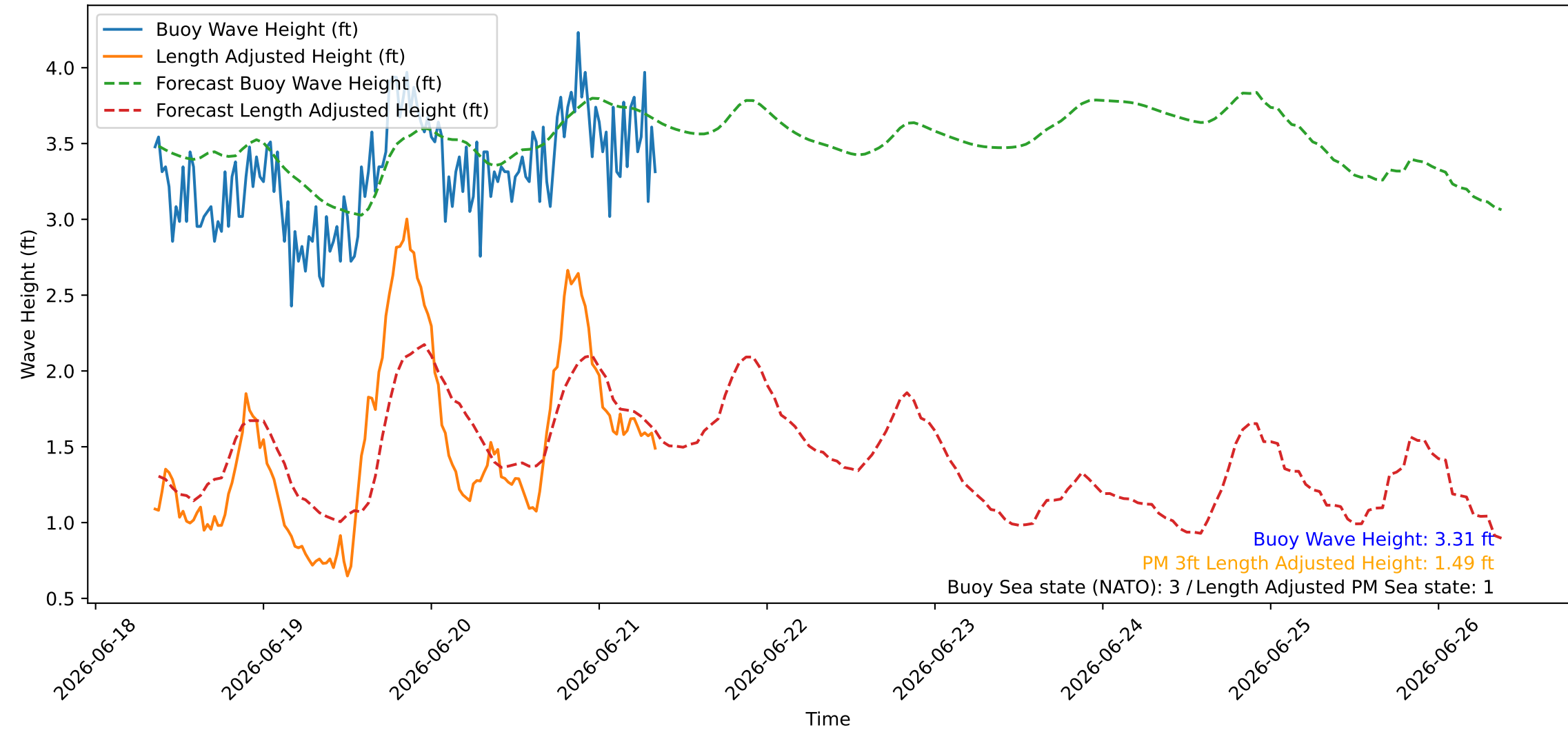
Wave Heights over Time for Green Beach at 2026-06-21 08:41:07
