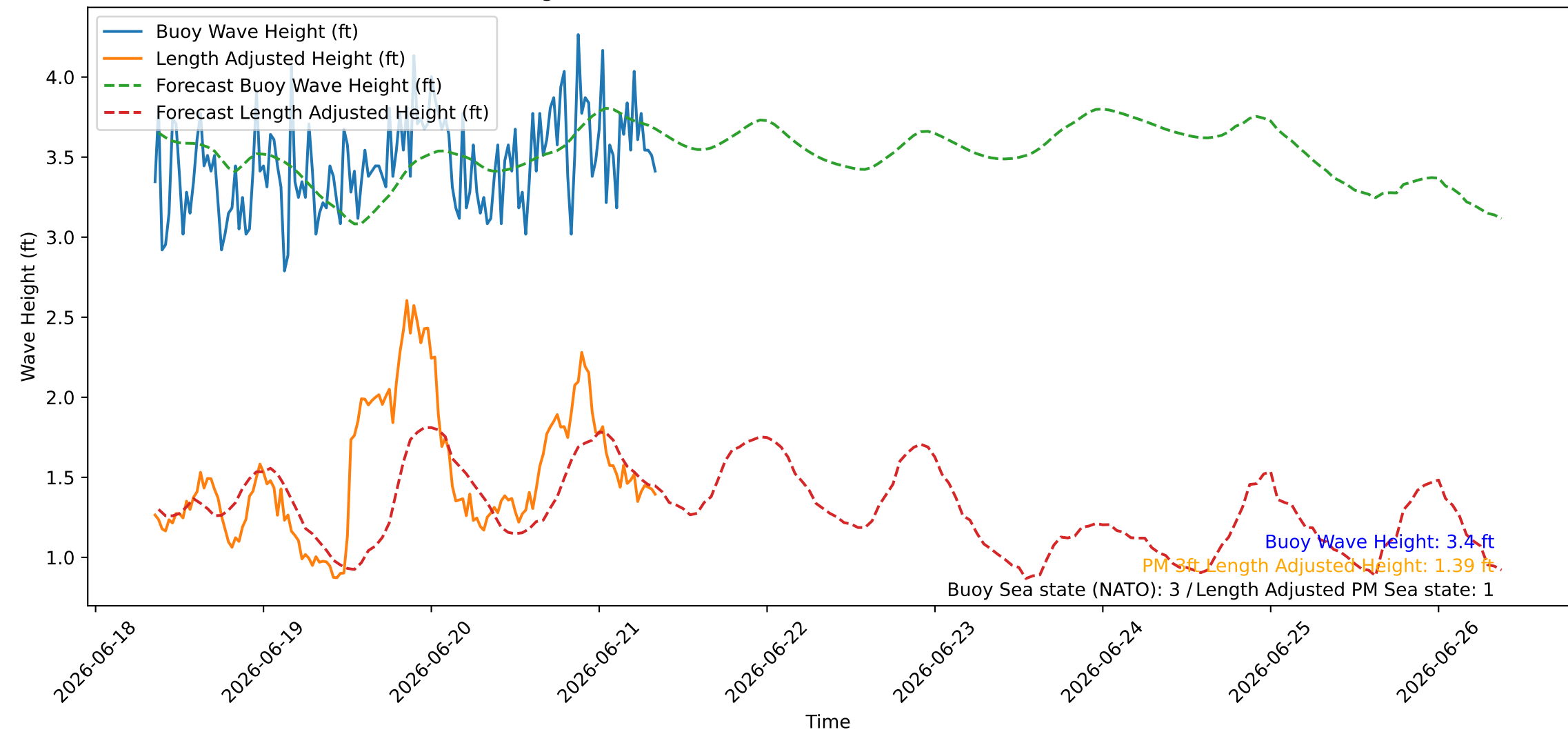
Wave Heights over Time for Oceanside Harbor at 2026-06-21 08:40:26
