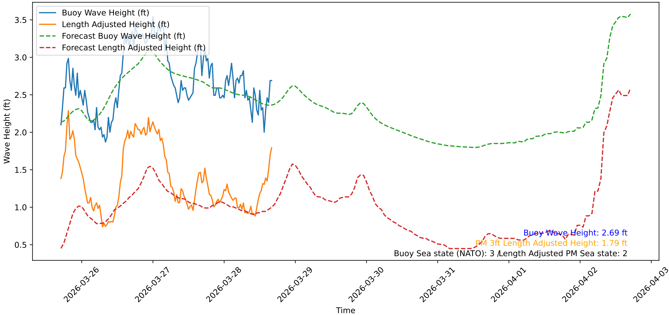
Wave Heights over Time for Green Beach at 2026-03-28 16:51:09
