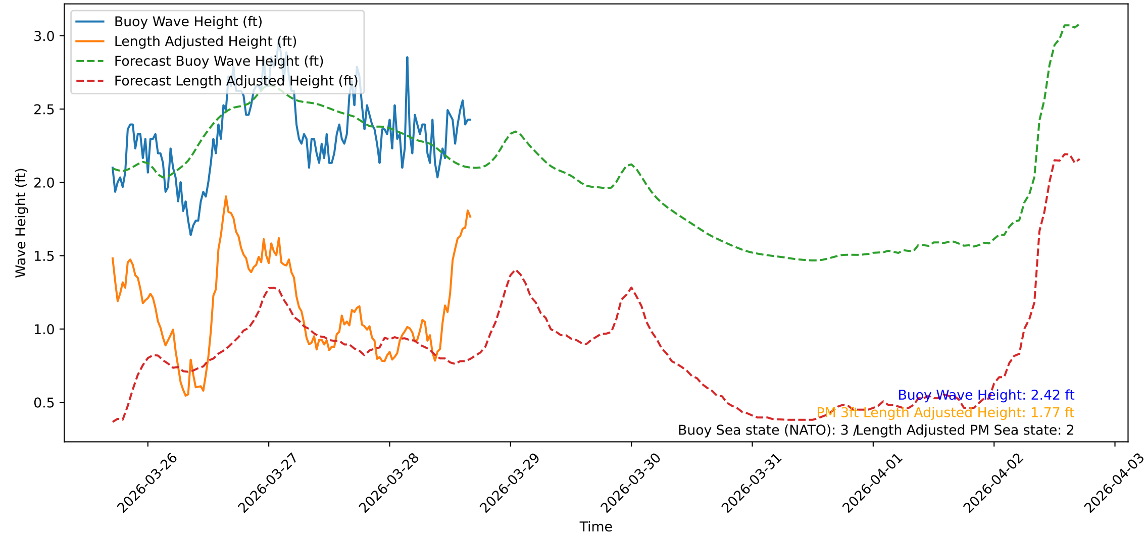
Wave Heights over Time for Red Beach at 2026-03-28 16:50:47
