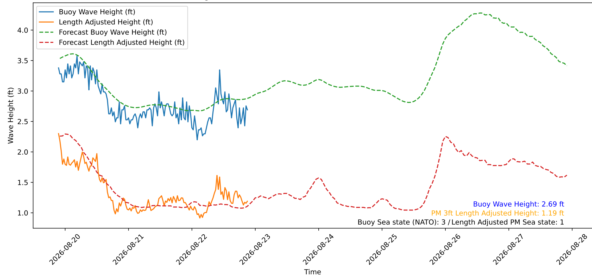
Wave Heights over Time for Oceanside Harbor at 2026-08-22 21:40:29
