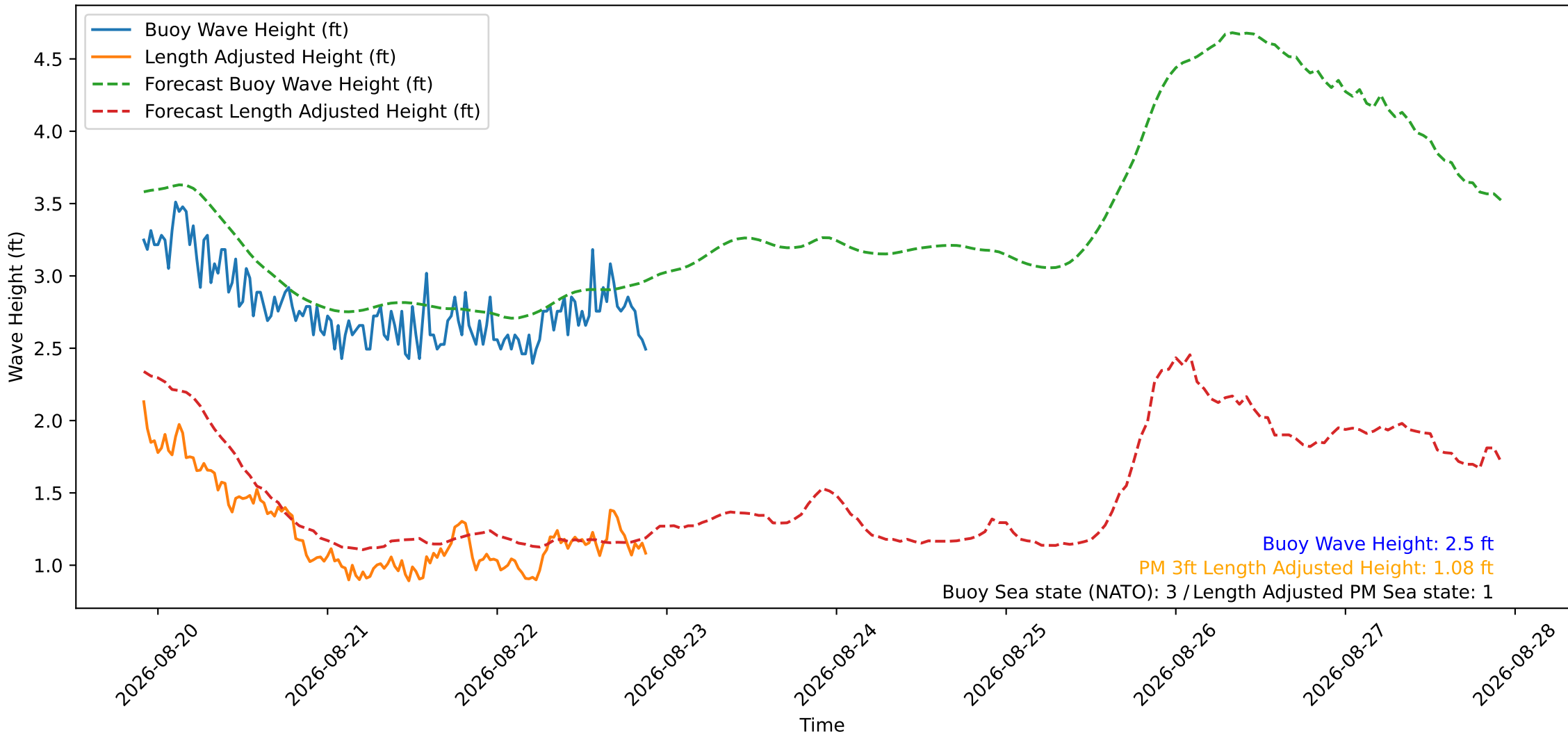
Wave Heights over Time for Green Beach at 2026-08-22 21:41:11
