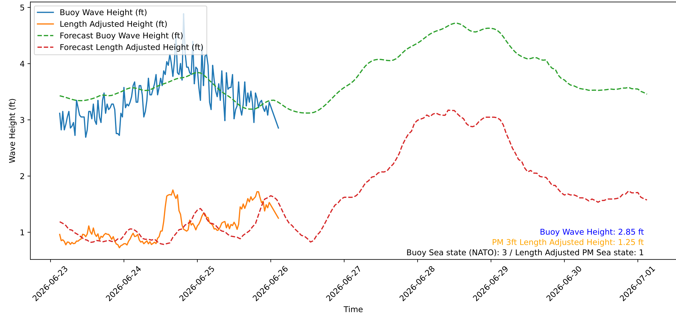
Wave Heights over Time for Oceanside Harbor at 2026-06-26 03:10:26
