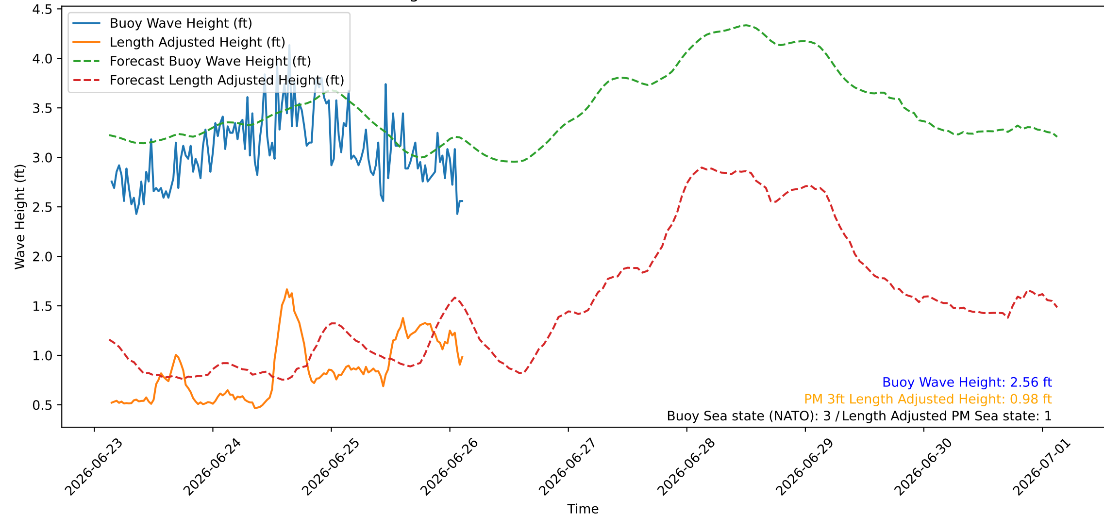
Wave Heights over Time for Red Beach at 2026-06-26 03:10:45
