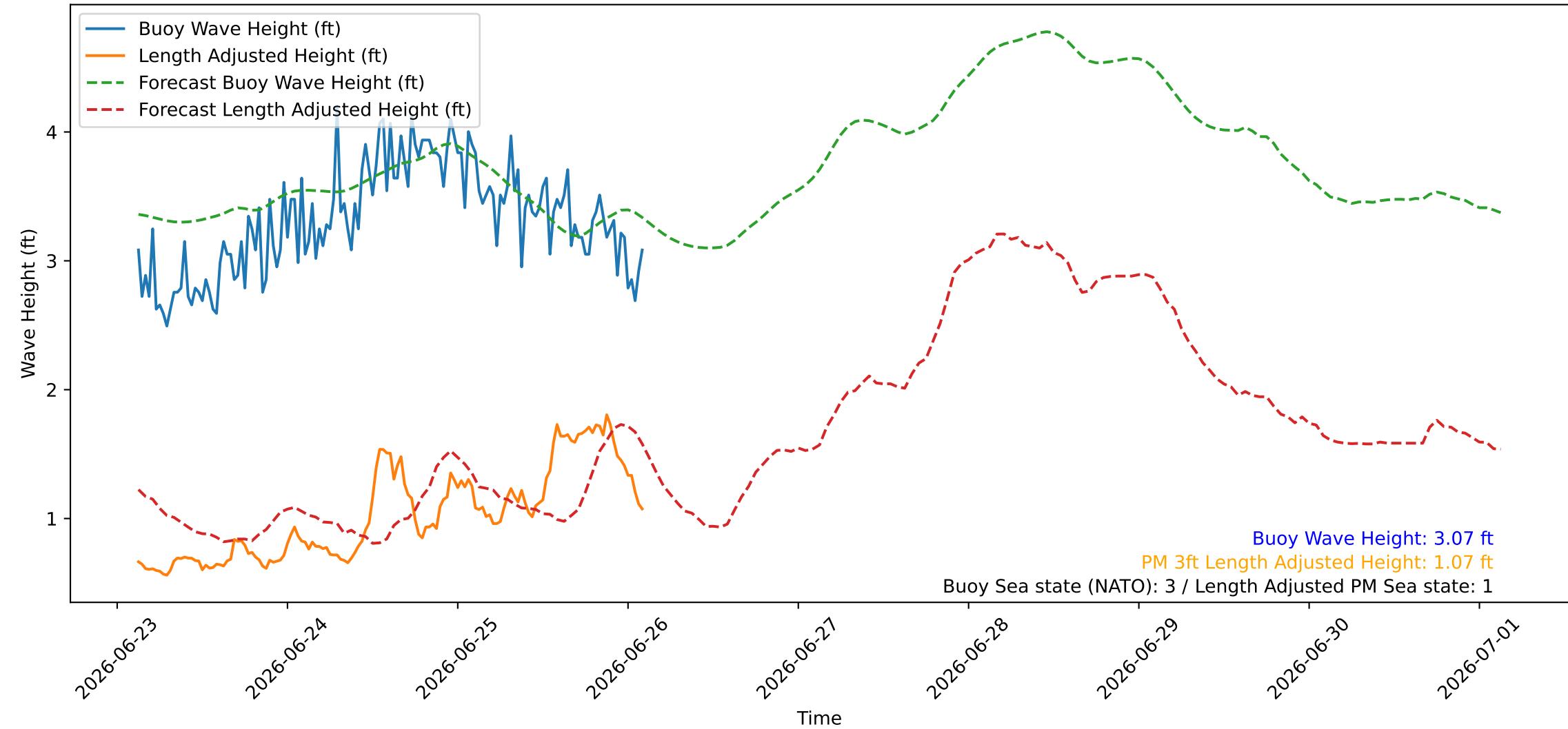
Wave Heights over Time for Green Beach at 2026-06-26 03:11:08
