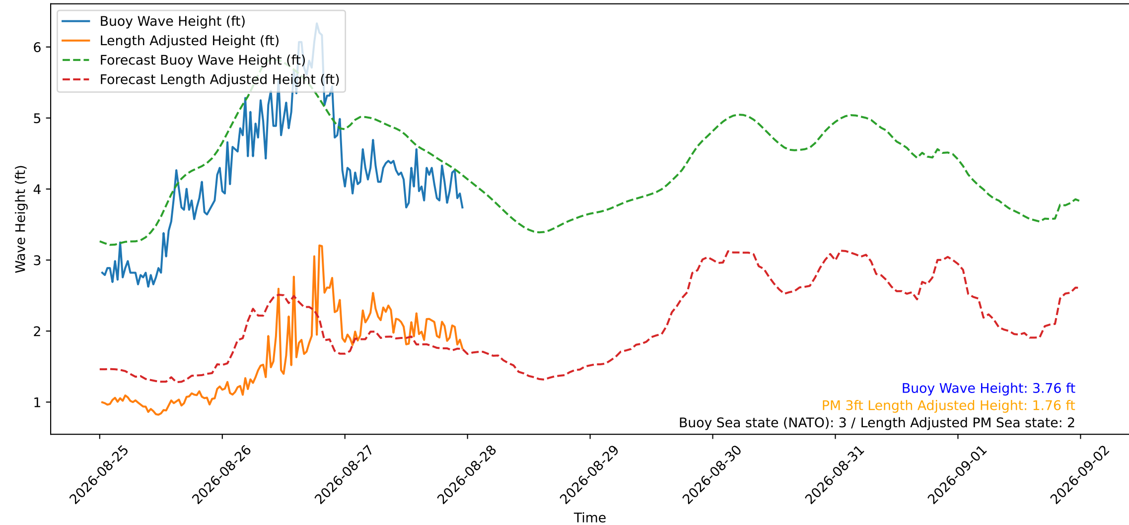
Wave Heights over Time for Green Beach at 2026-08-28 00:21:14
