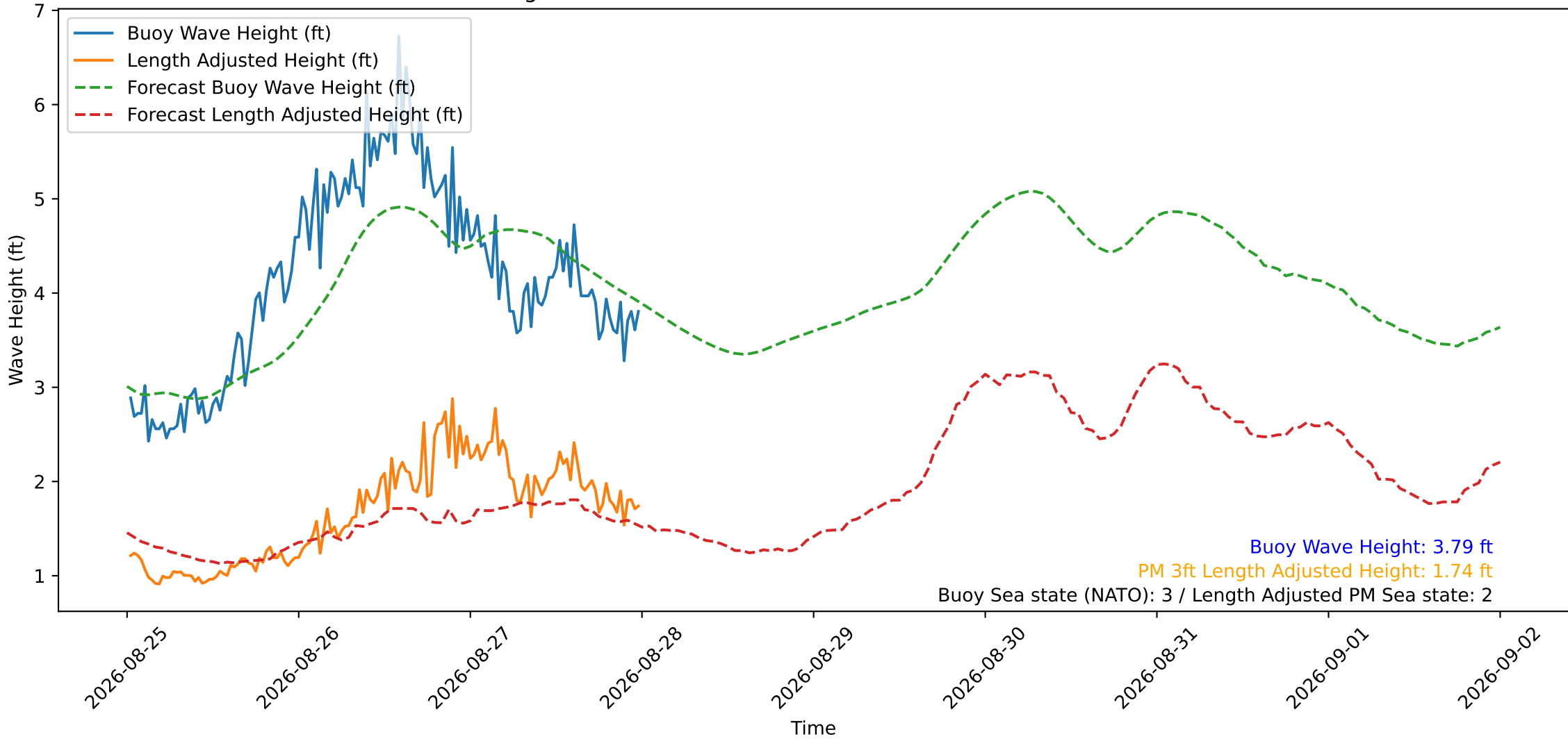
Wave Heights over Time for Oceanside Harbor at 2026-08-28 00:20:29
