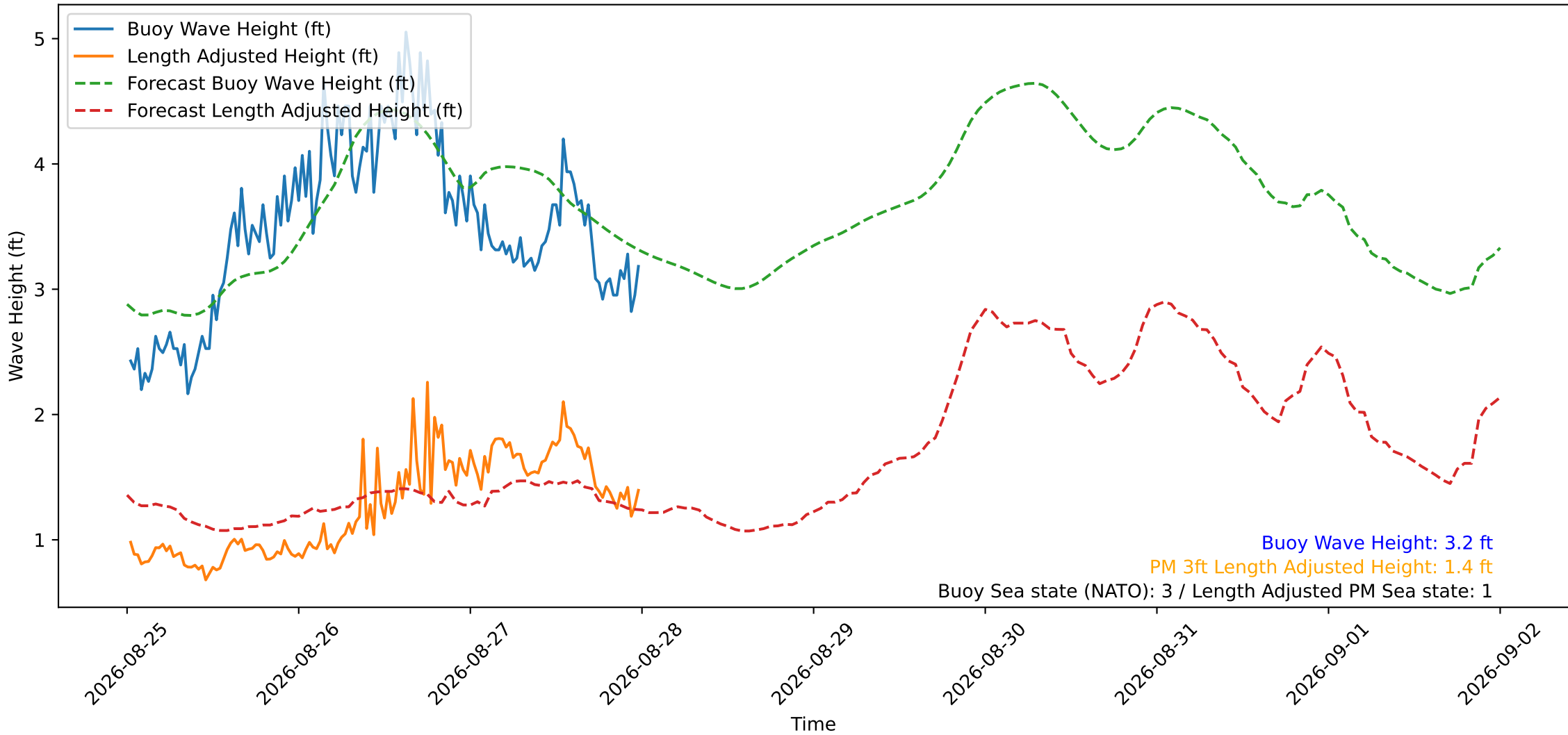
Wave Heights over Time for Red Beach at 2026-08-28 00:20:50
