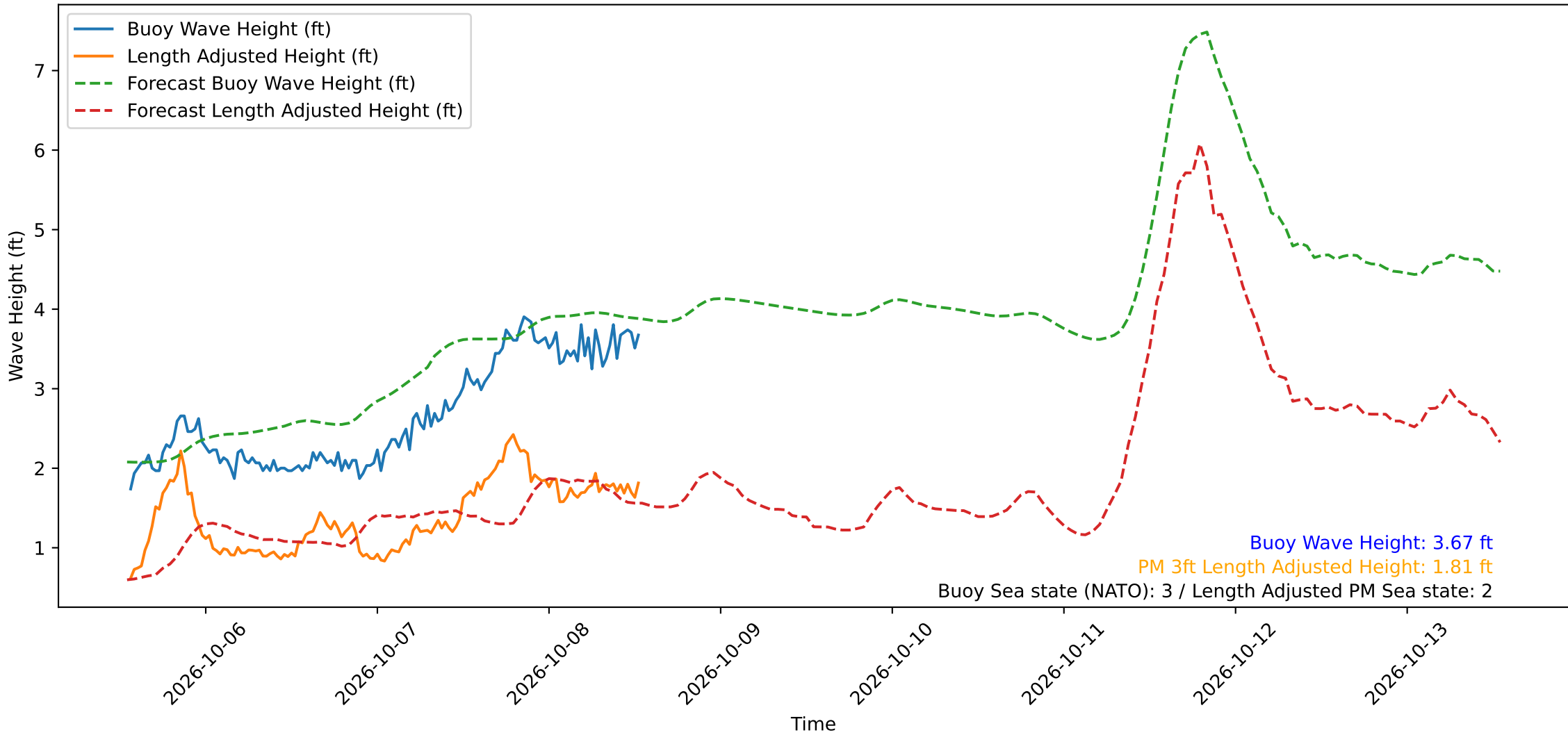
Wave Heights over Time for Red Beach at 2026-10-08 13:10:51
