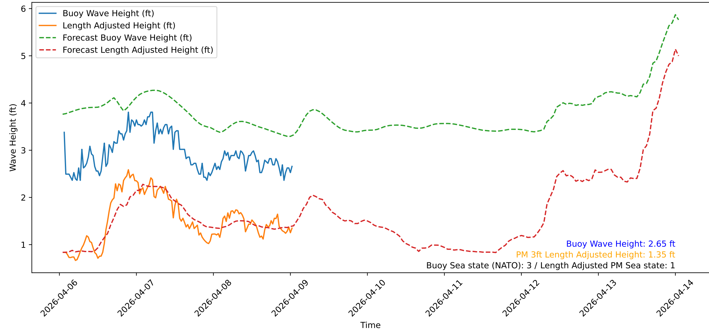
Wave Heights over Time for Green Beach at 2026-04-09 01:21:09
