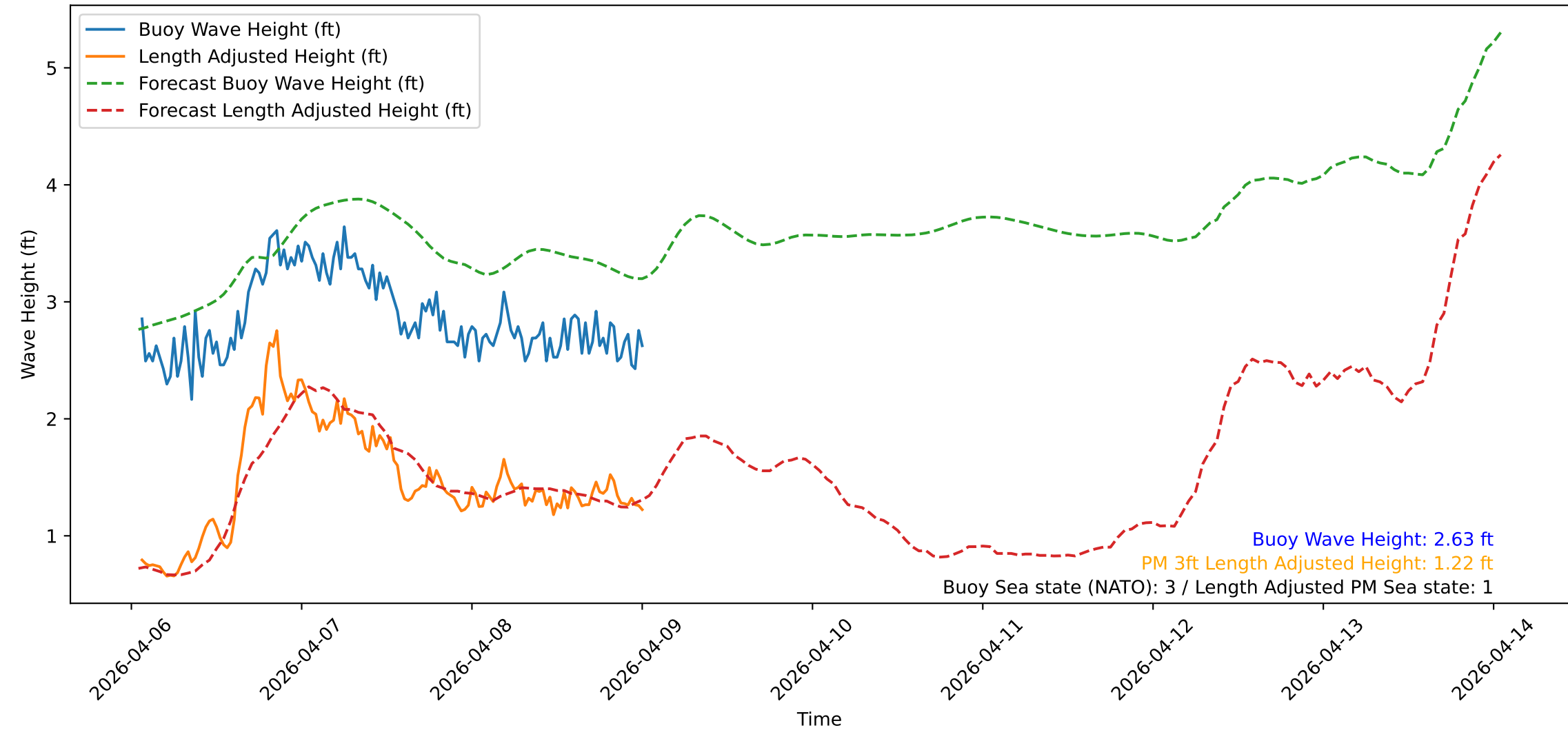
Wave Heights over Time for Oceanside Harbor at 2026-04-09 01:20:31
