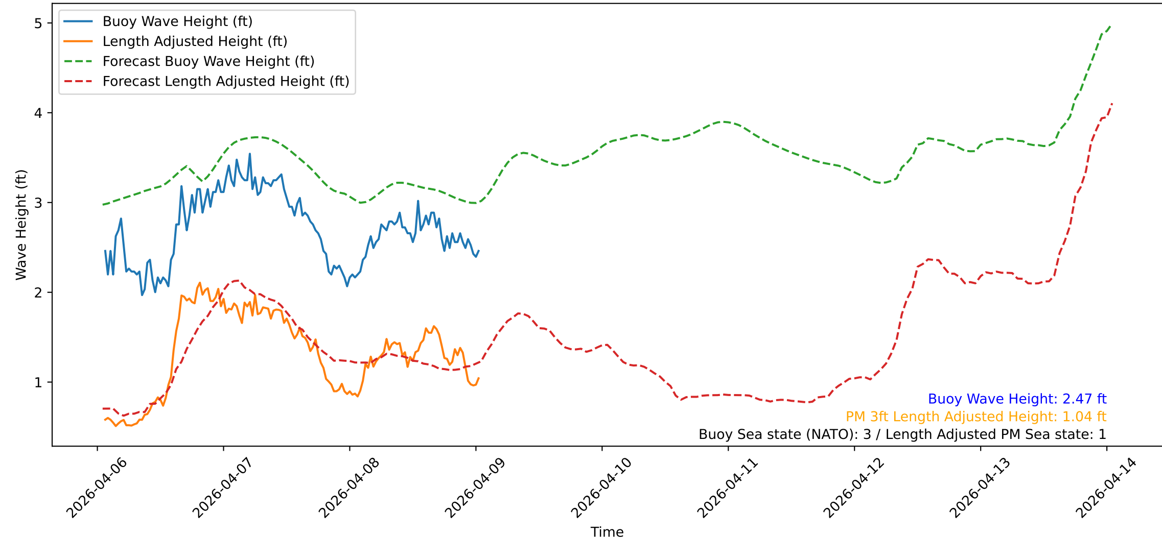
Wave Heights over Time for Red Beach at 2026-04-09 01:20:48
