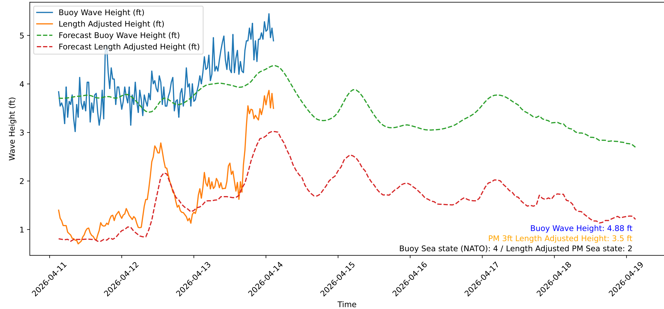
Wave Heights over Time for Oceanside Harbor at 2026-04-14 03:10:32
