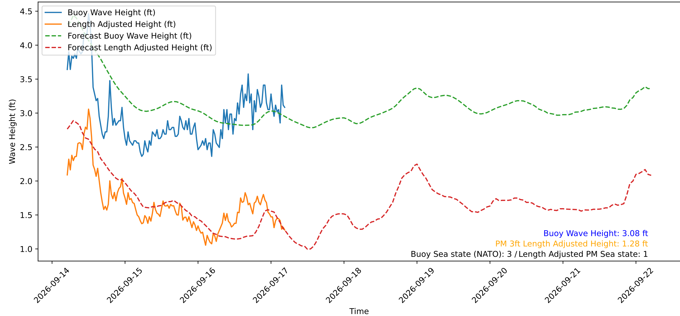
Wave Heights over Time for Oceanside Harbor at 2026-09-17 05:10:29
