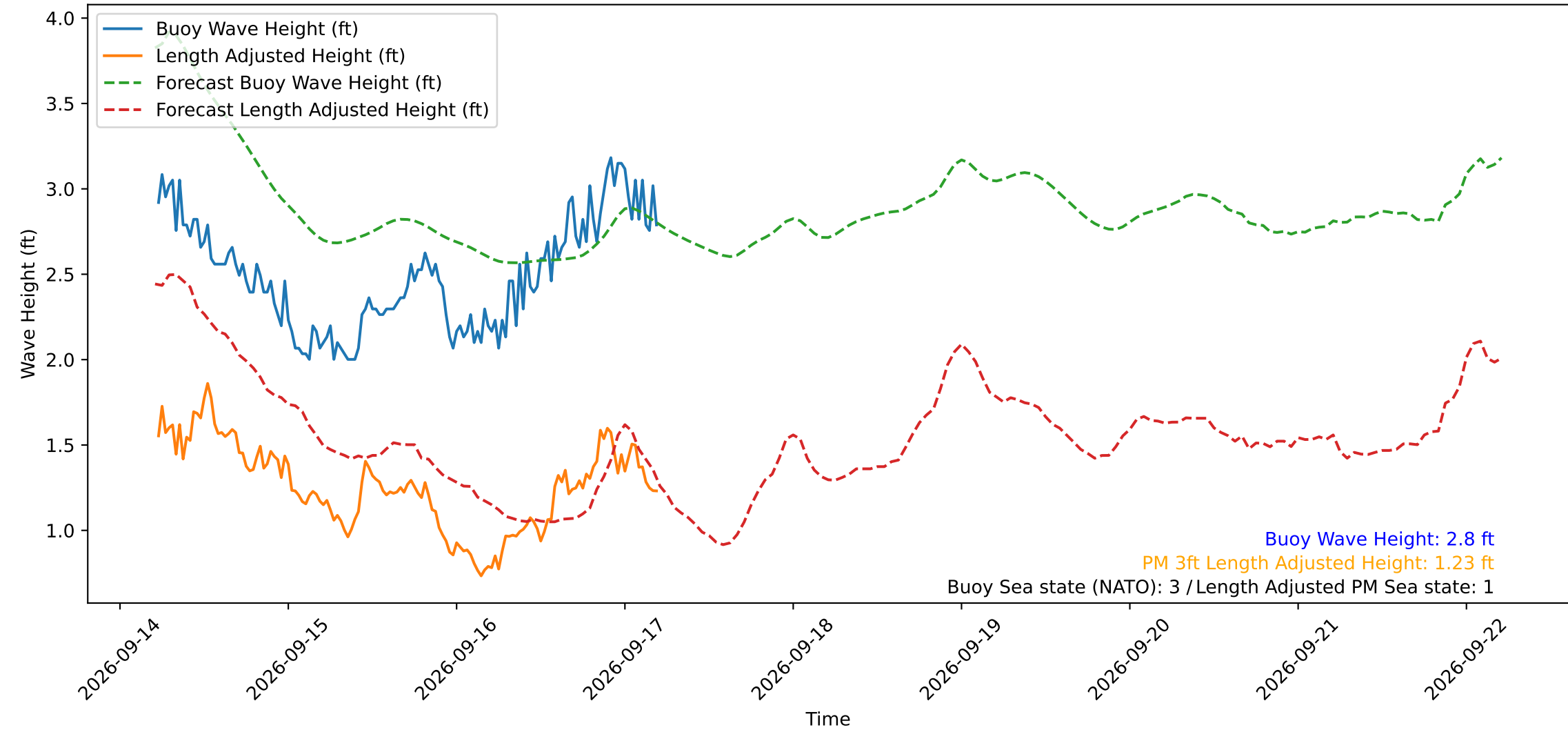
Wave Heights over Time for Red Beach at 2026-09-17 05:10:49
