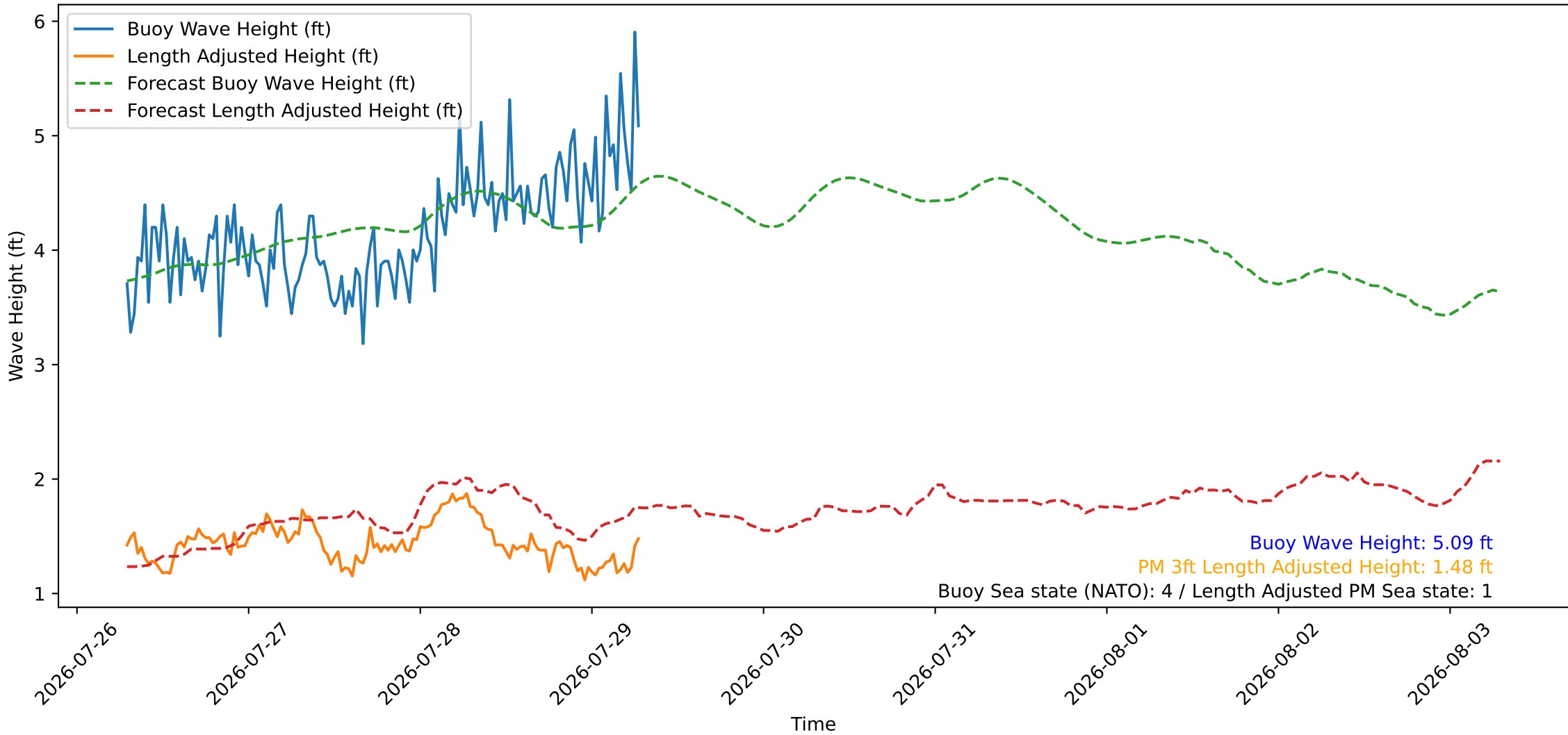
Wave Heights over Time for Oceanside Harbor at 2026-07-29 07:10:26
