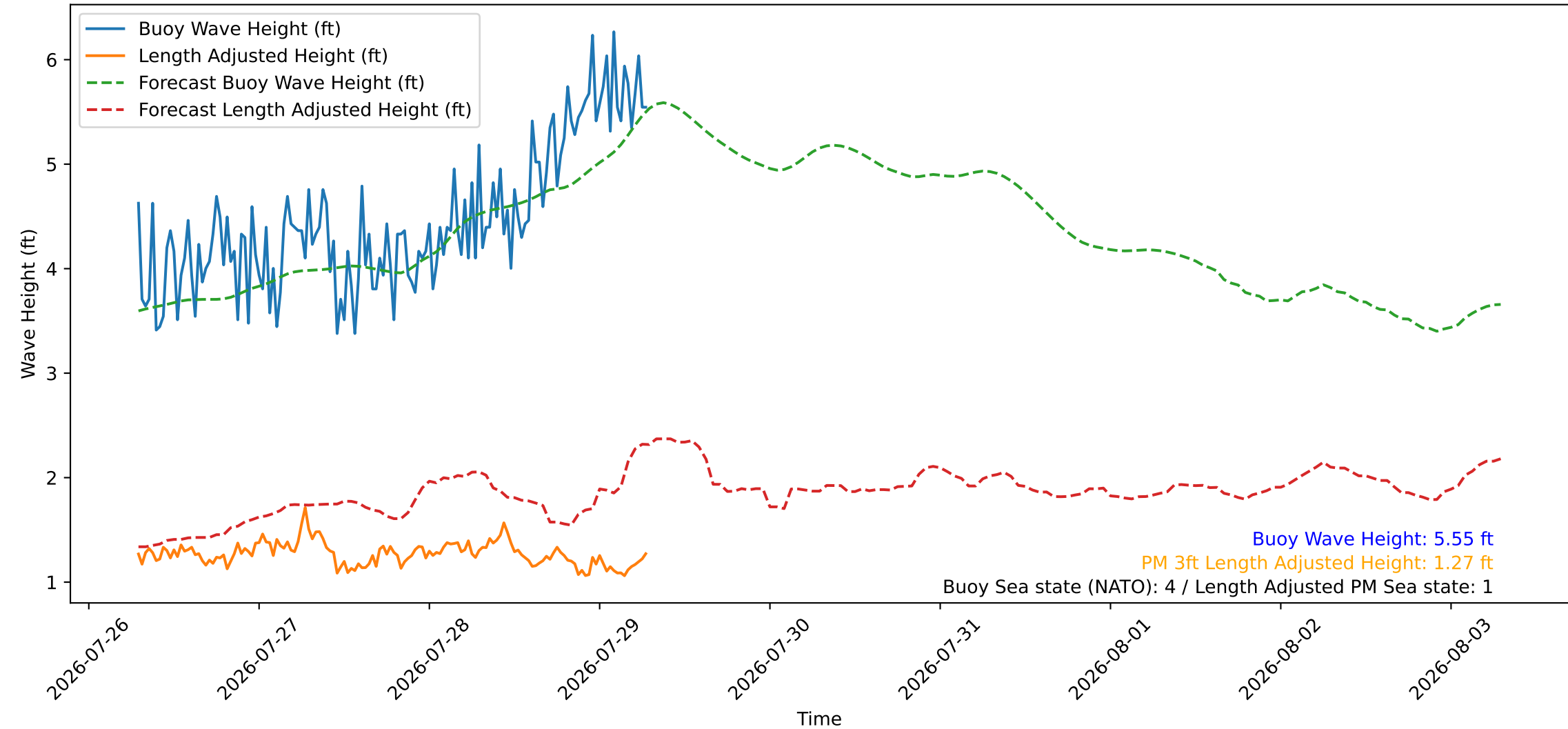
Wave Heights over Time for Green Beach at 2026-07-29 07:11:09
