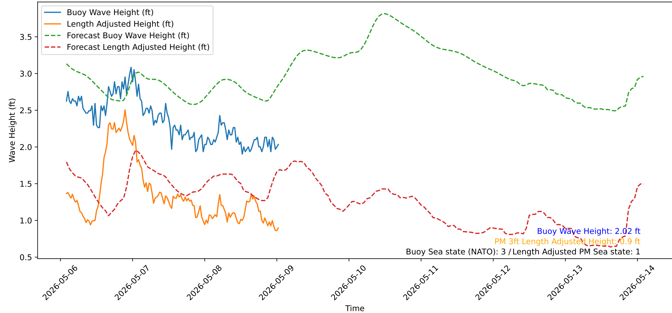
Wave Heights over Time for Red Beach at 2026-05-09 01:30:51
