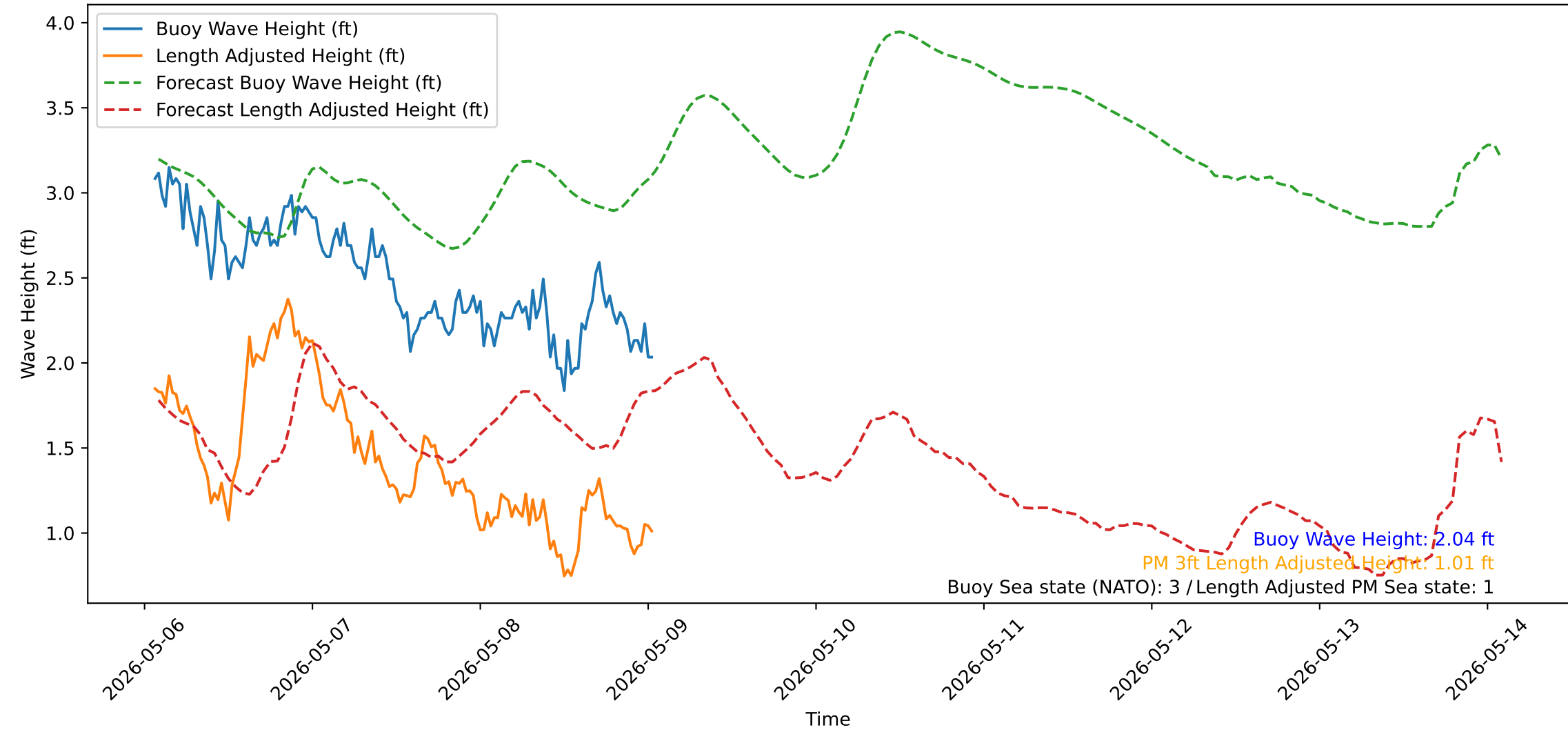
Wave Heights over Time for Green Beach at 2026-05-09 01:31:13
