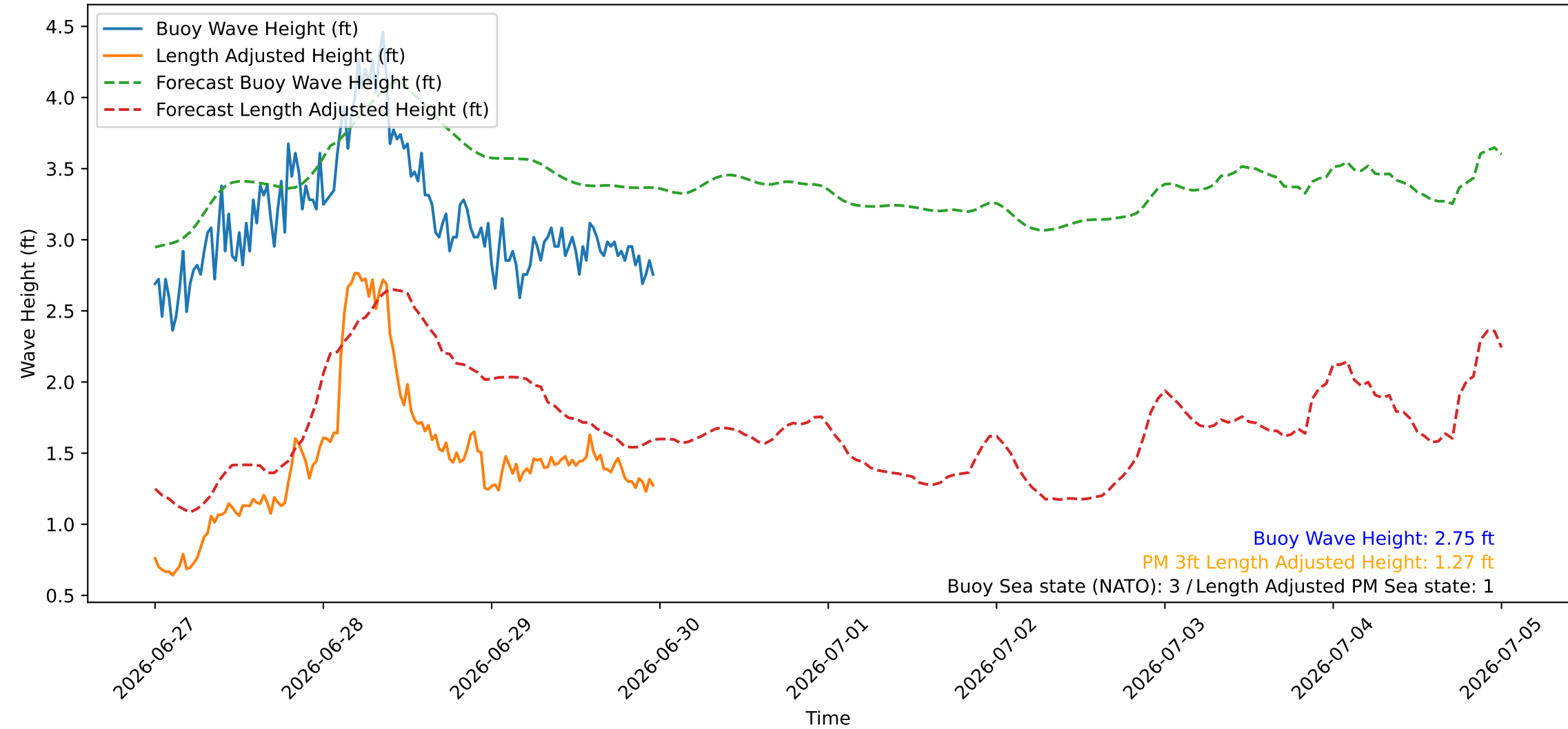
Wave Heights over Time for Red Beach at 2026-06-29 23:50:47
