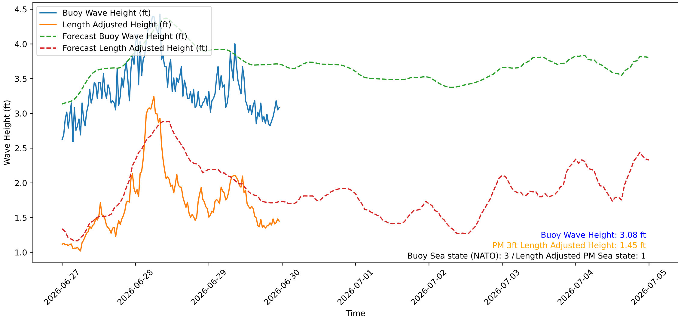
Wave Heights over Time for Oceanside Harbor at 2026-06-29 23:50:26
