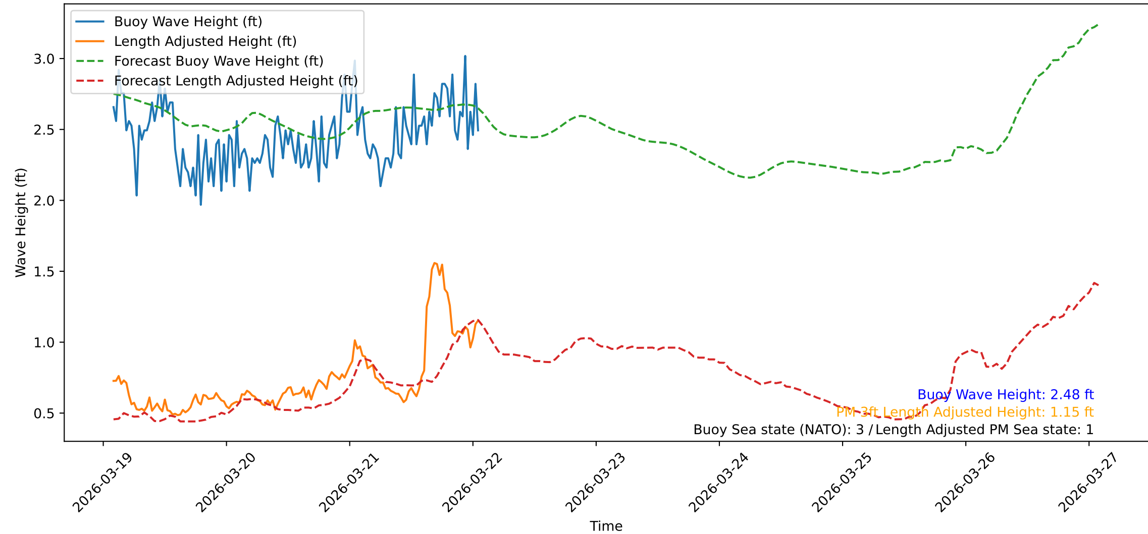
Wave Heights over Time for Oceanside Harbor at 2026-03-22 02:00:32
