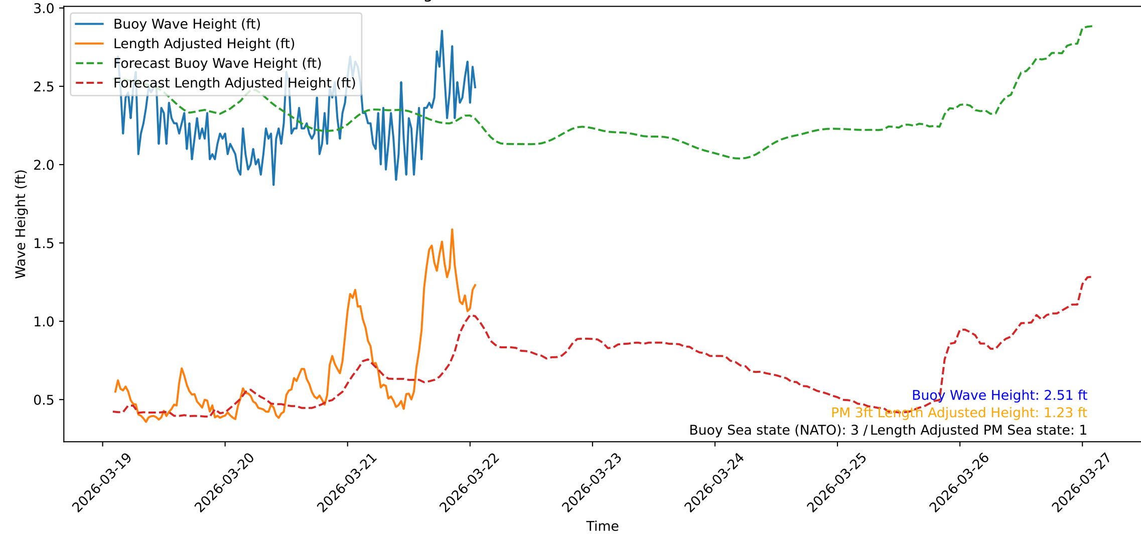
Wave Heights over Time for Red Beach at 2026-03-22 02:00:48
