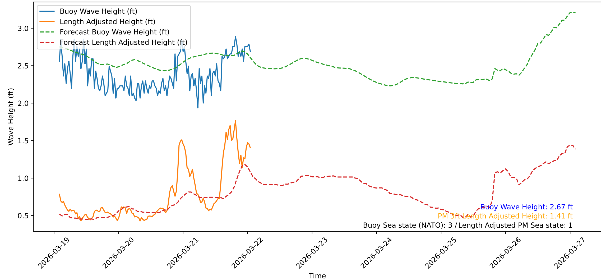
Wave Heights over Time for Green Beach at 2026-03-22 02:01:10
