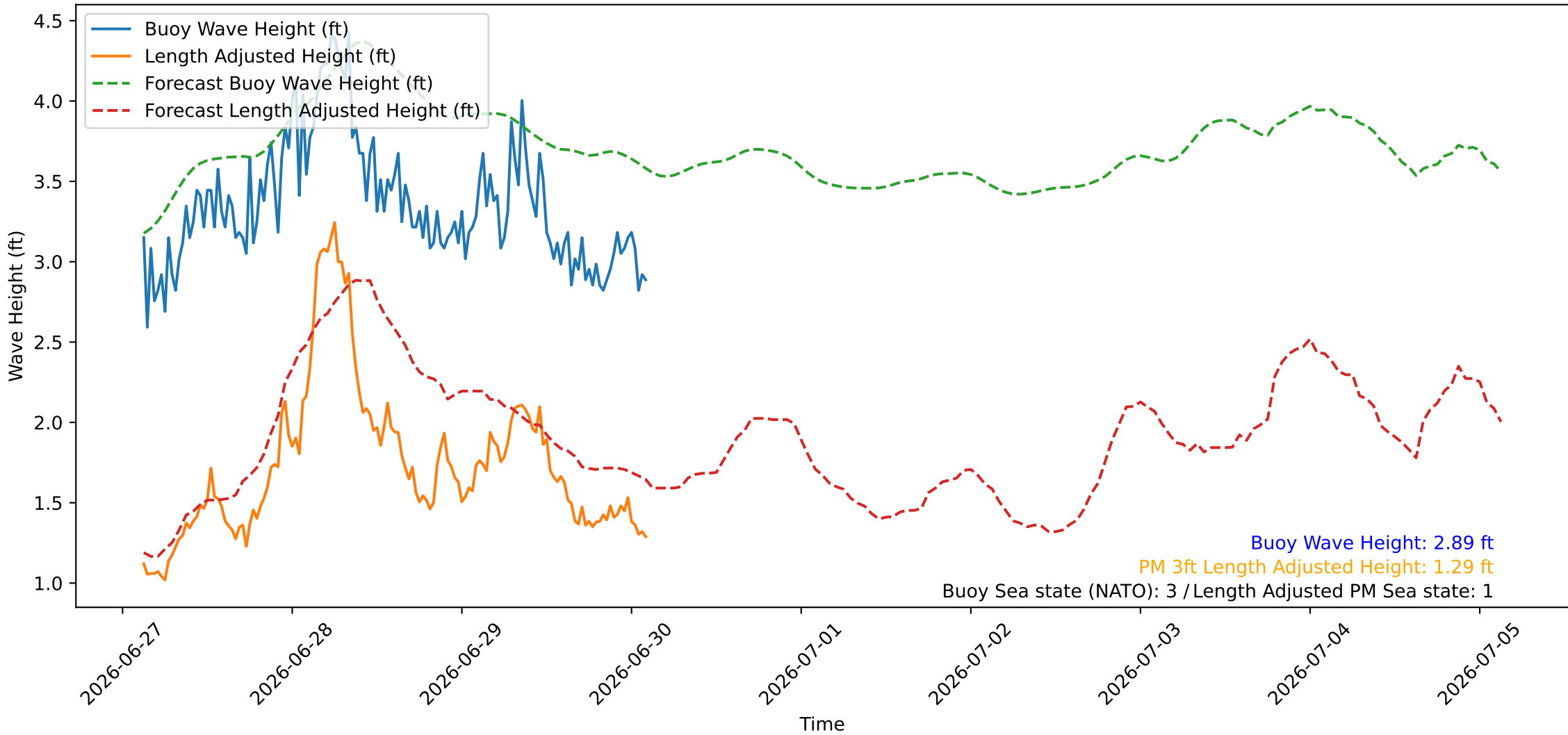
Wave Heights over Time for Oceanside Harbor at 2026-06-30 02:50:26
