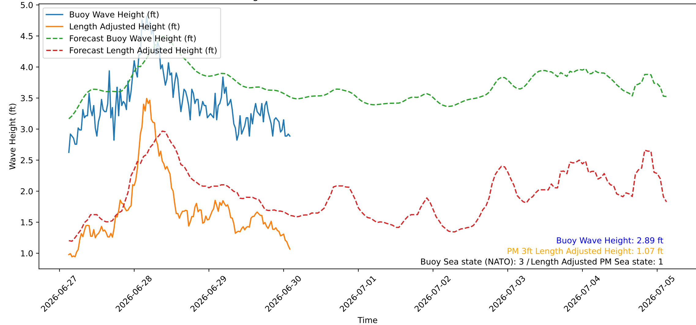
Wave Heights over Time for Green Beach at 2026-06-30 02:51:09
