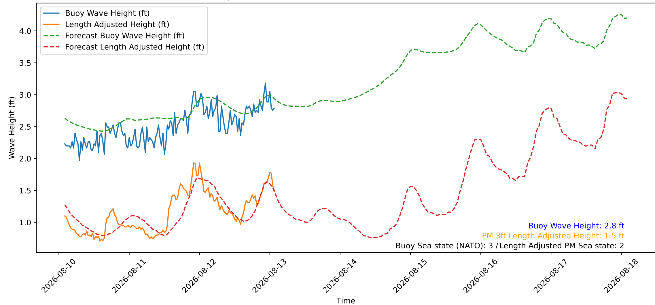
Wave Heights over Time for Oceanside Harbor at 2026-08-13 02:10:26
