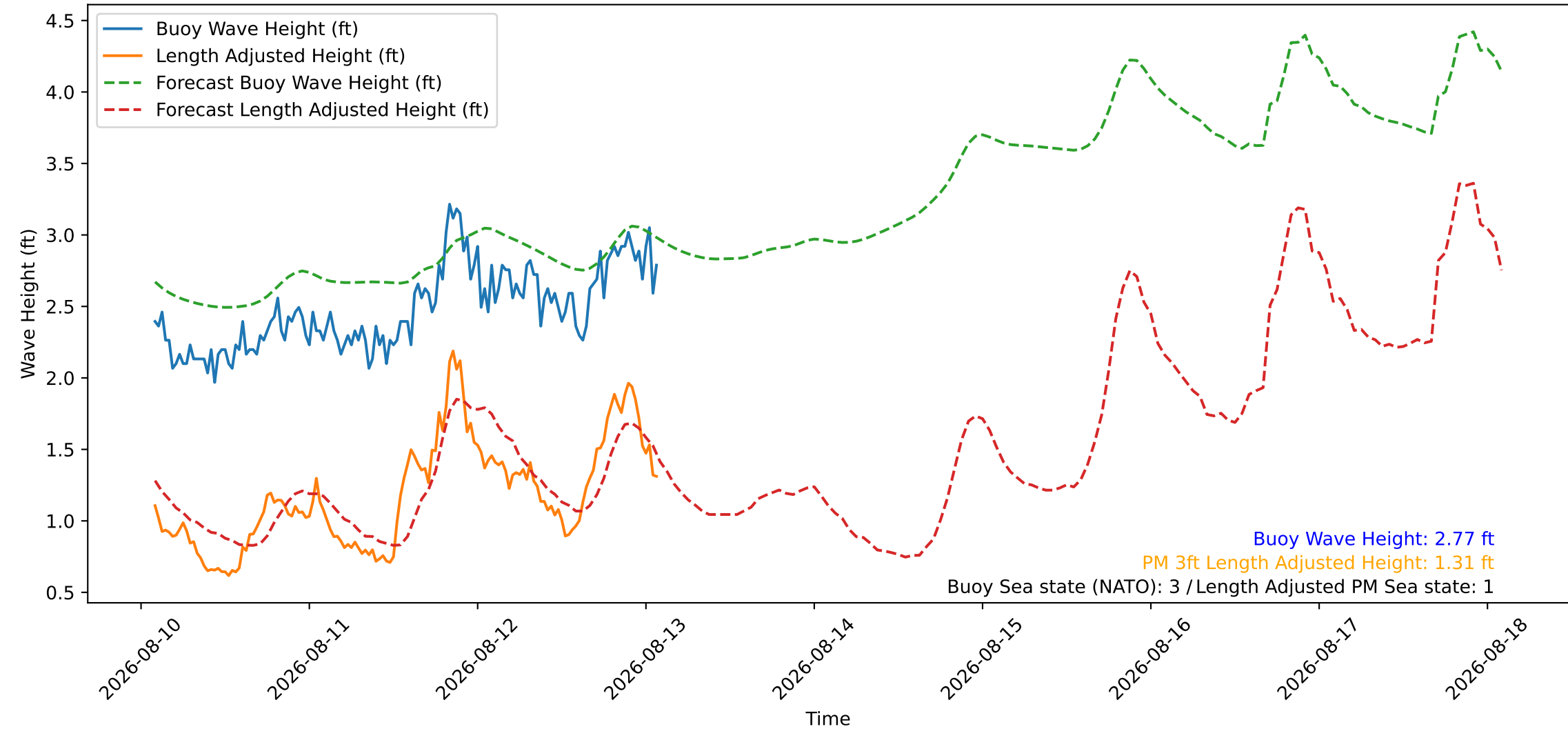
Wave Heights over Time for Green Beach at 2026-08-13 02:11:08
