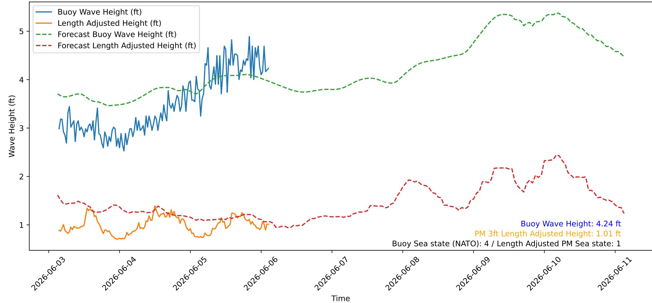
Wave Heights over Time for Red Beach at 2026-06-06 03:20:47
