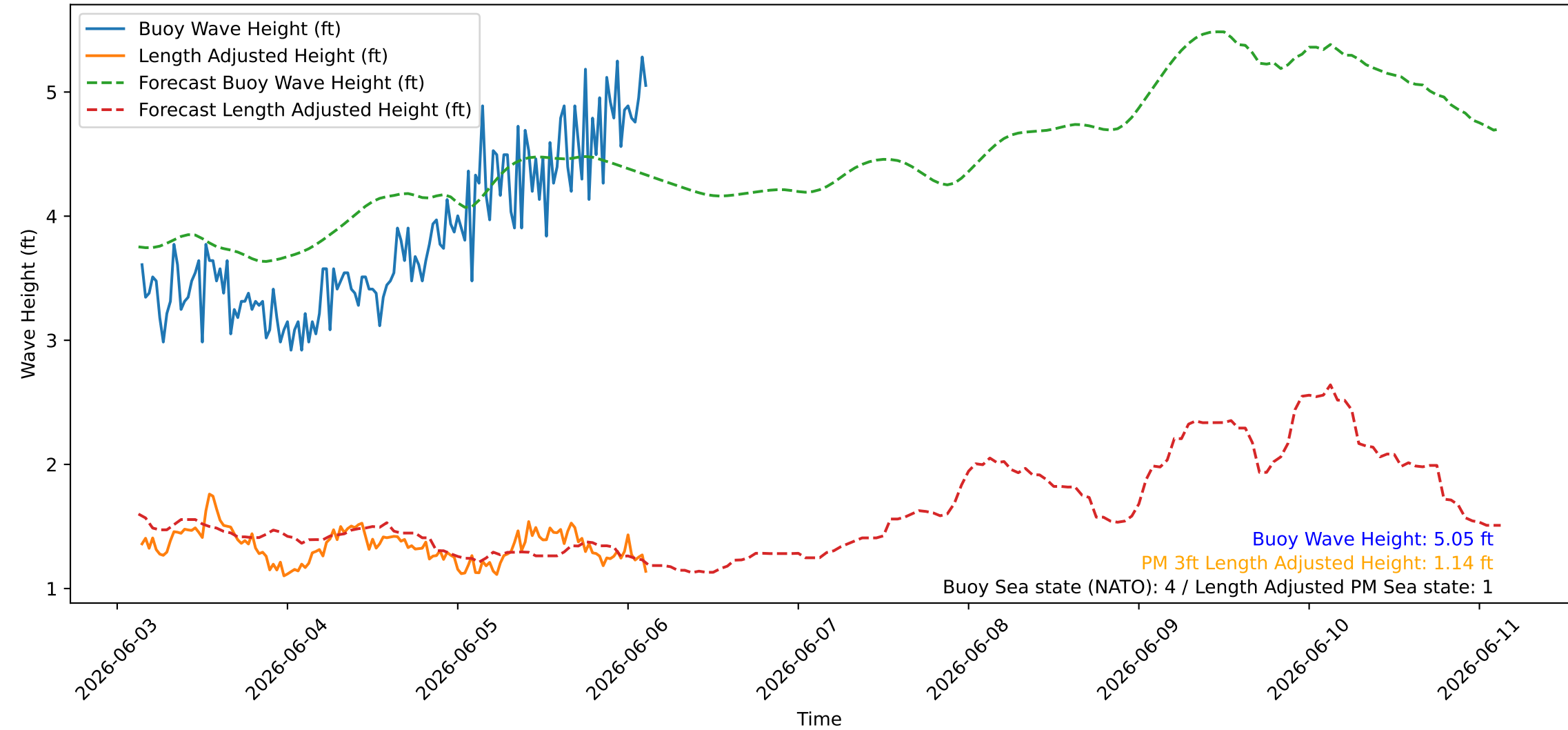
Wave Heights over Time for Oceanside Harbor at 2026-06-06 03:20:26
