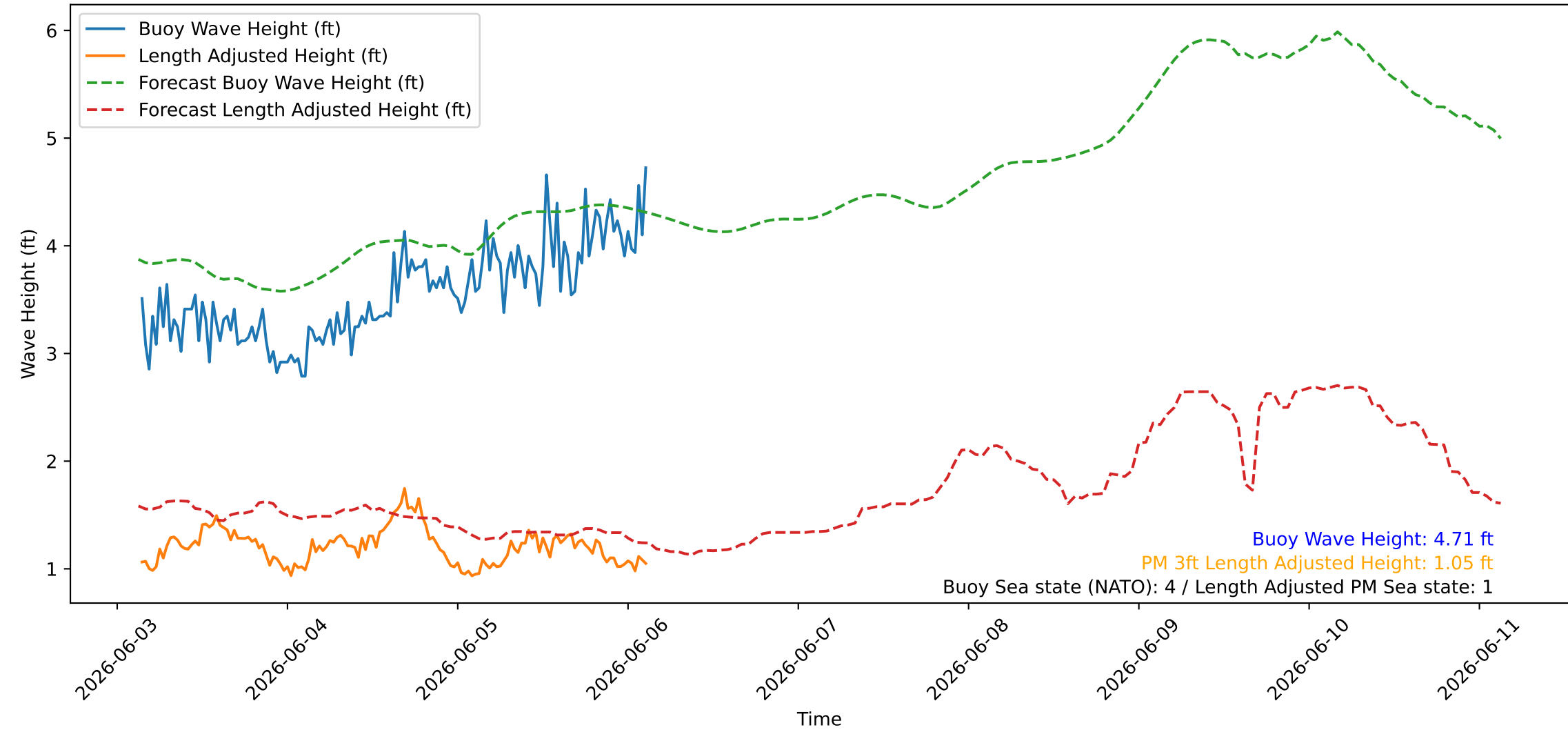
Wave Heights over Time for Green Beach at 2026-06-06 03:21:09
