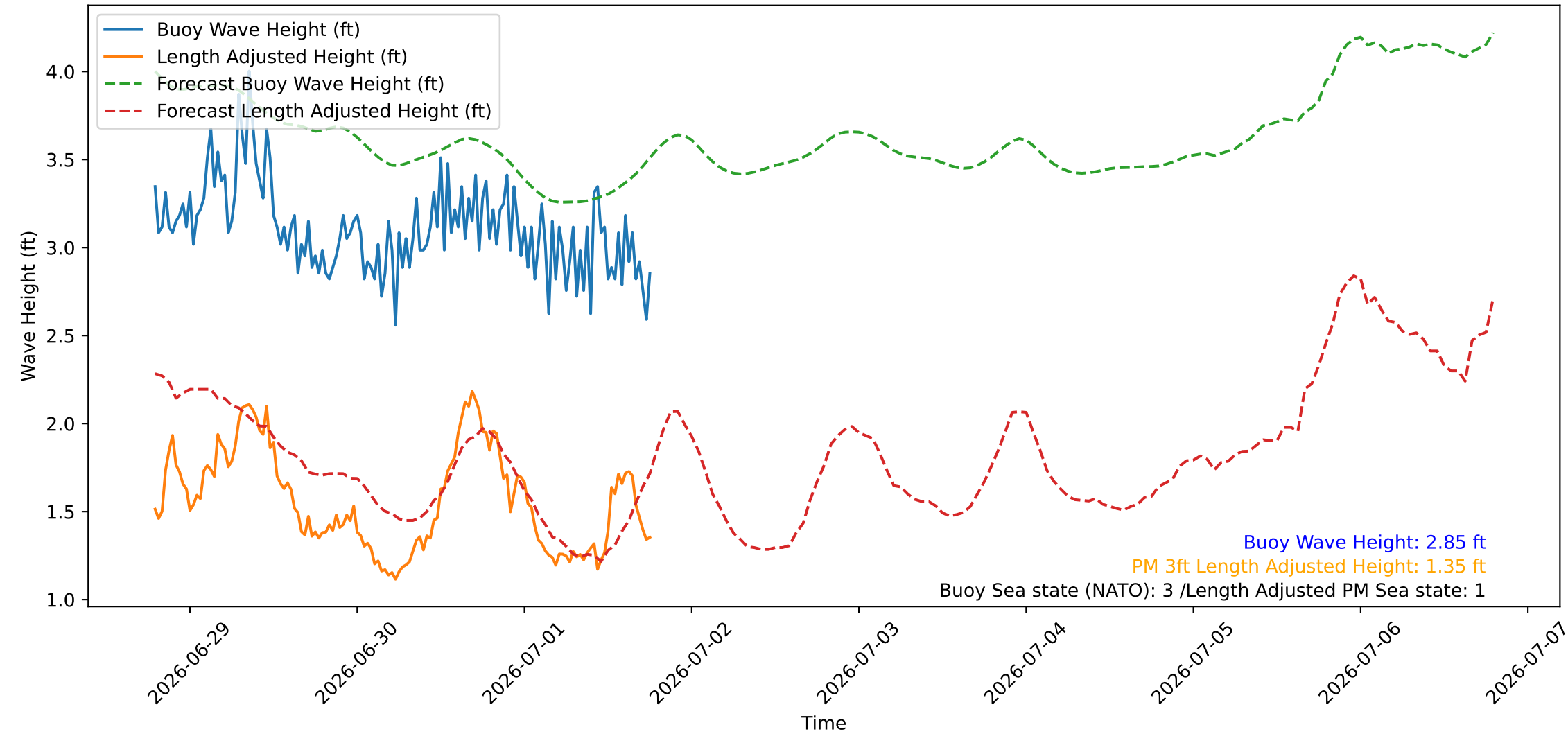
Wave Heights over Time for Oceanside Harbor at 2026-07-01 19:00:26
