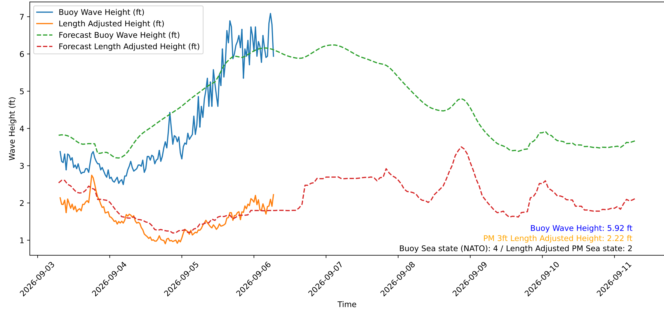
Wave Heights over Time for Green Beach at 2026-09-06 07:21:15
