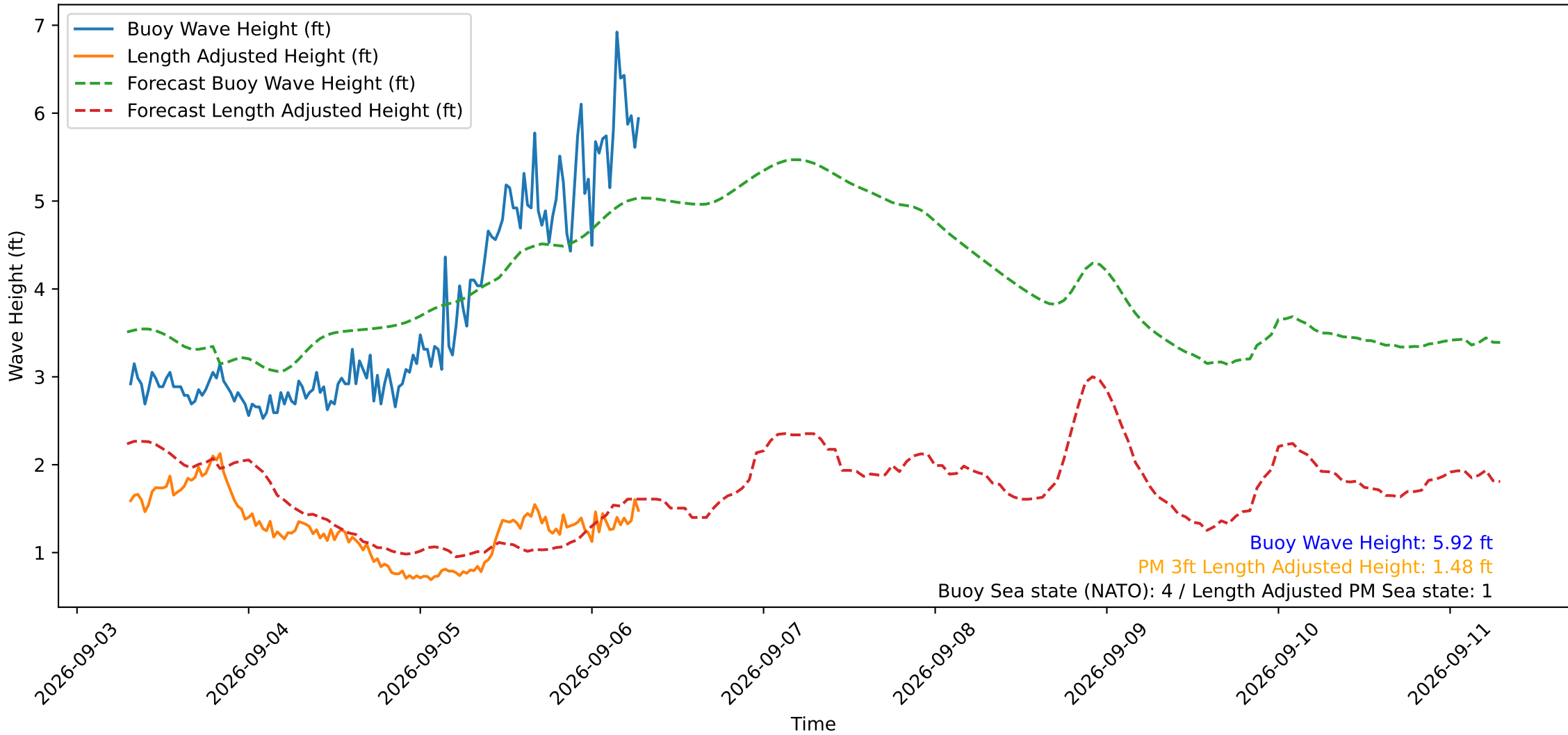
Wave Heights over Time for Red Beach at 2026-09-06 07:20:51
