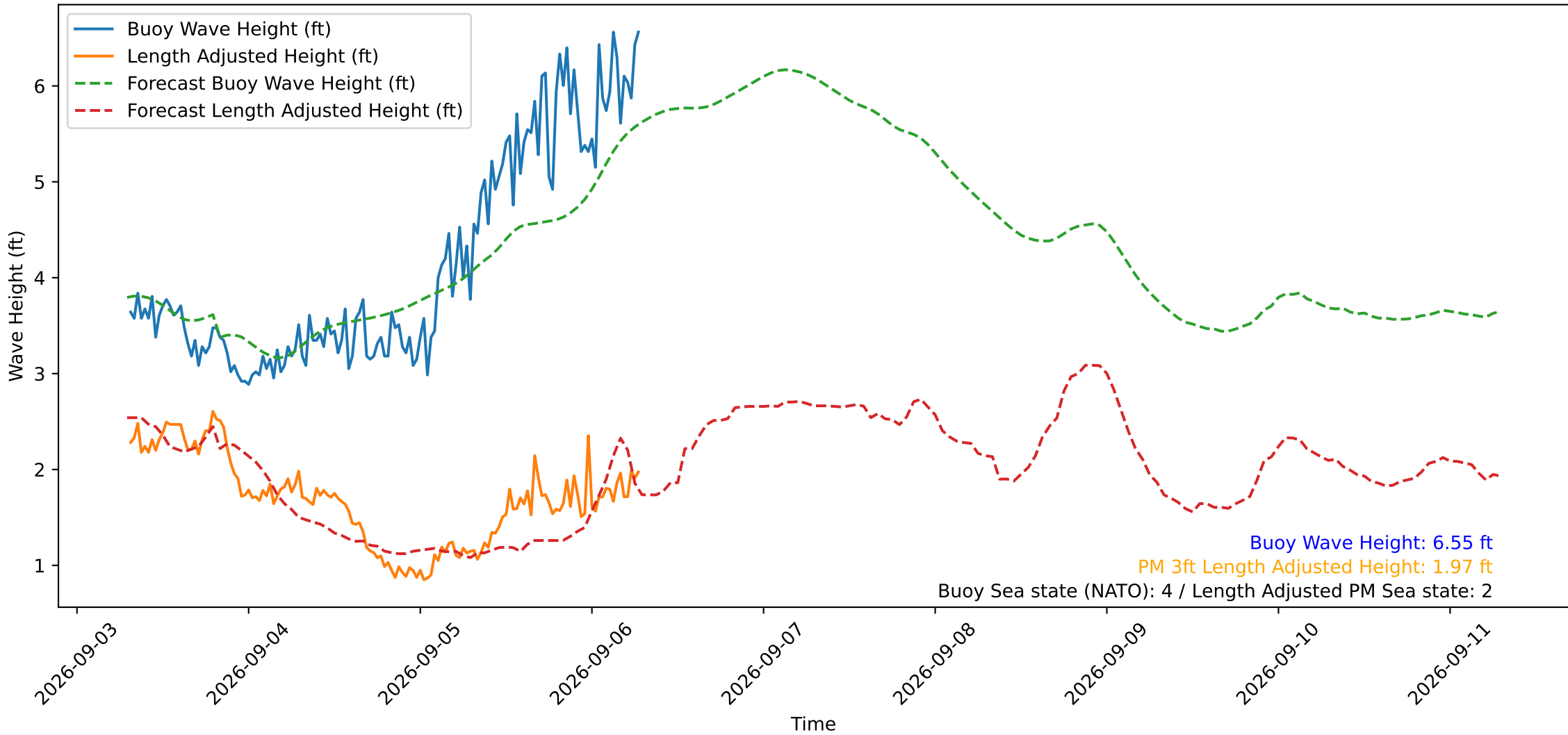
Wave Heights over Time for Oceanside Harbor at 2026-09-06 07:20:30
