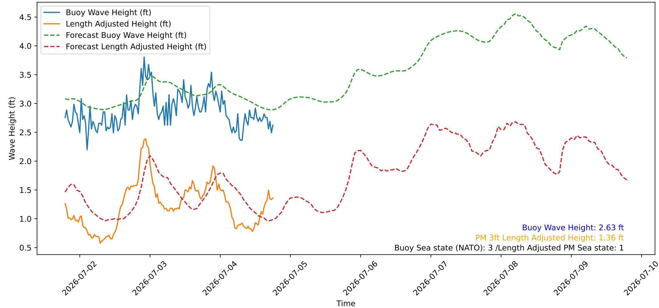
Wave Heights over Time for Red Beach at 2026-07-04 18:40:45
