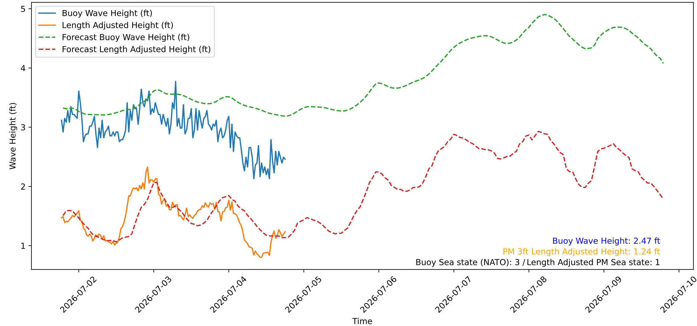
Wave Heights over Time for Oceanside Harbor at 2026-07-04 18:40:26
