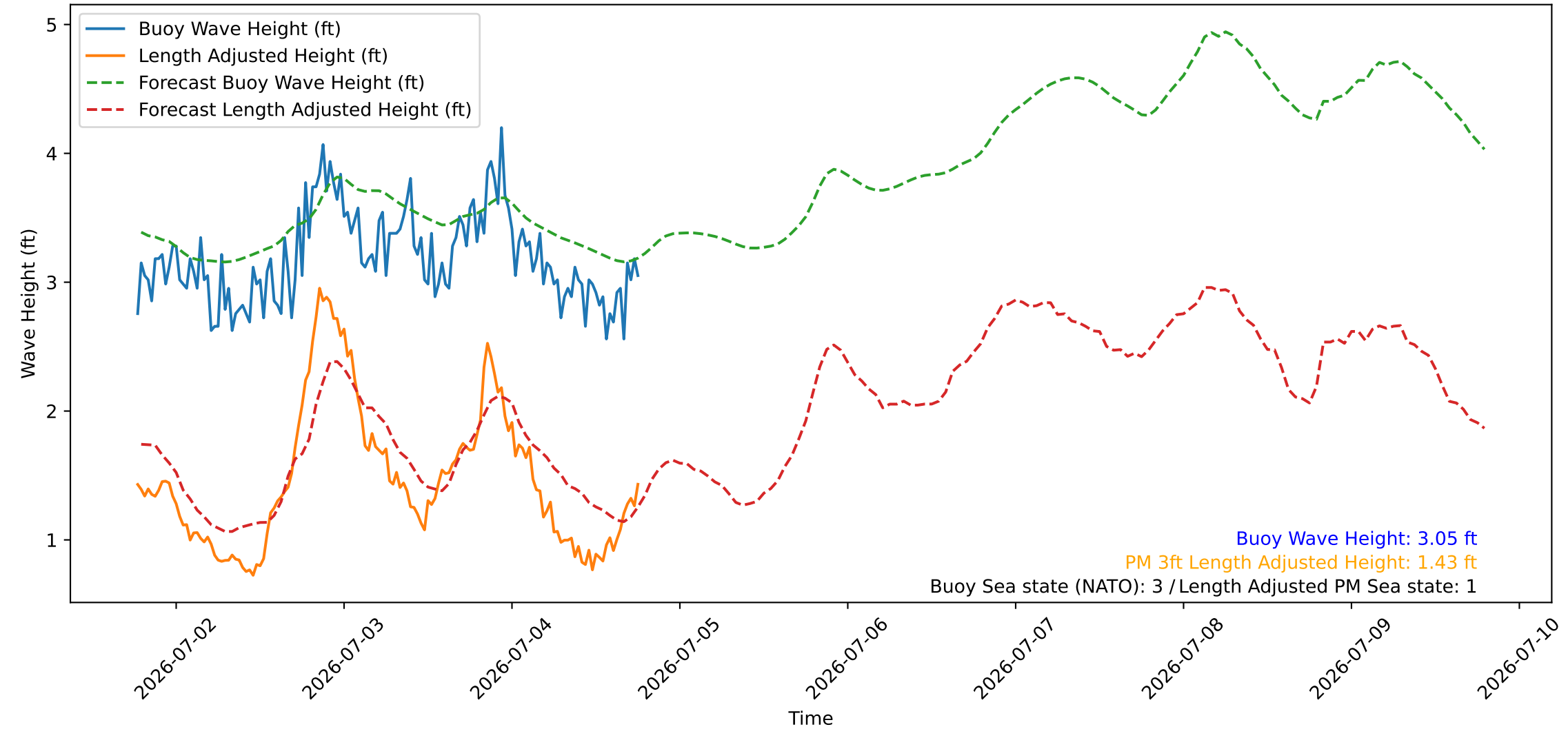
Wave Heights over Time for Green Beach at 2026-07-04 18:41:08
