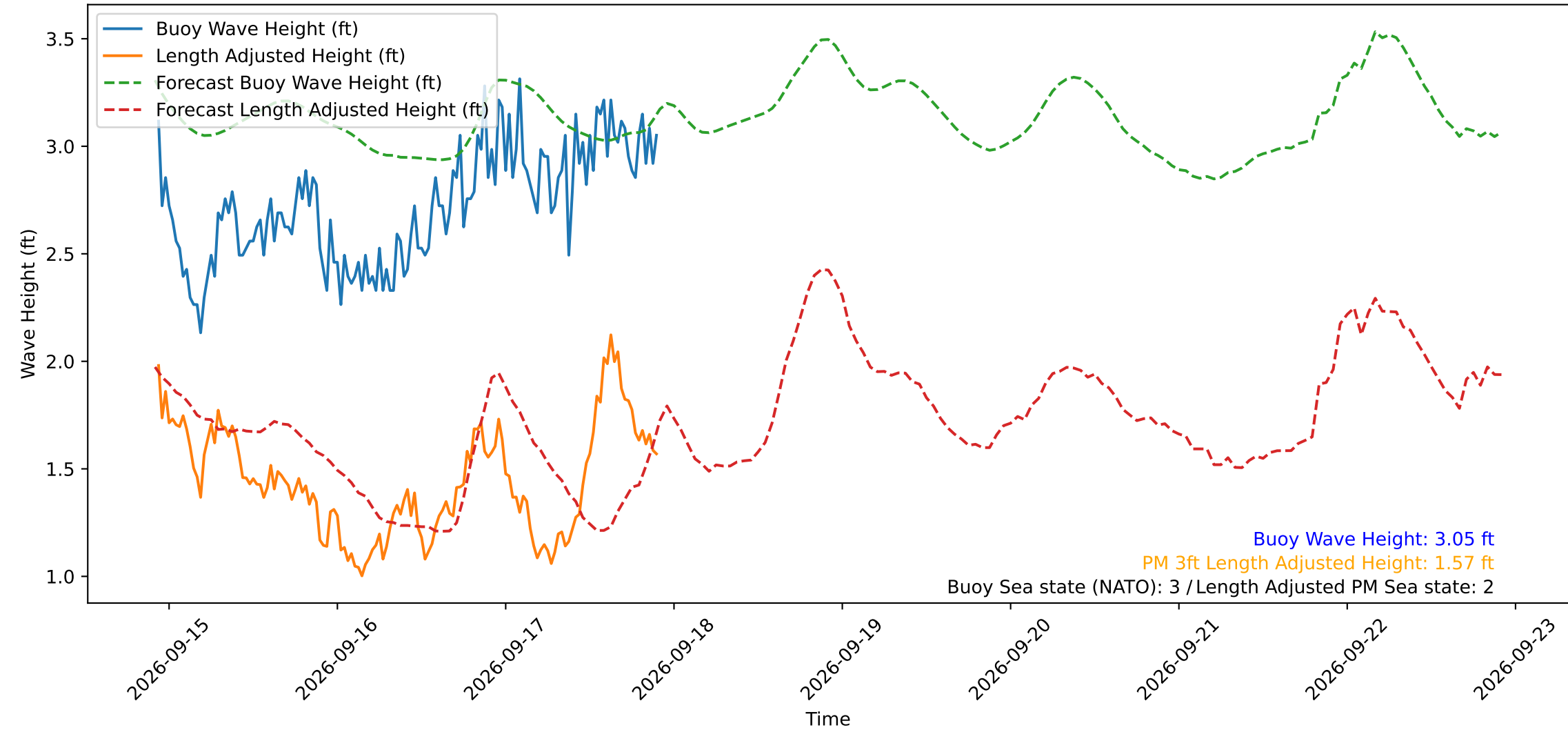
Wave Heights over Time for Green Beach at 2026-09-17 22:21:14
