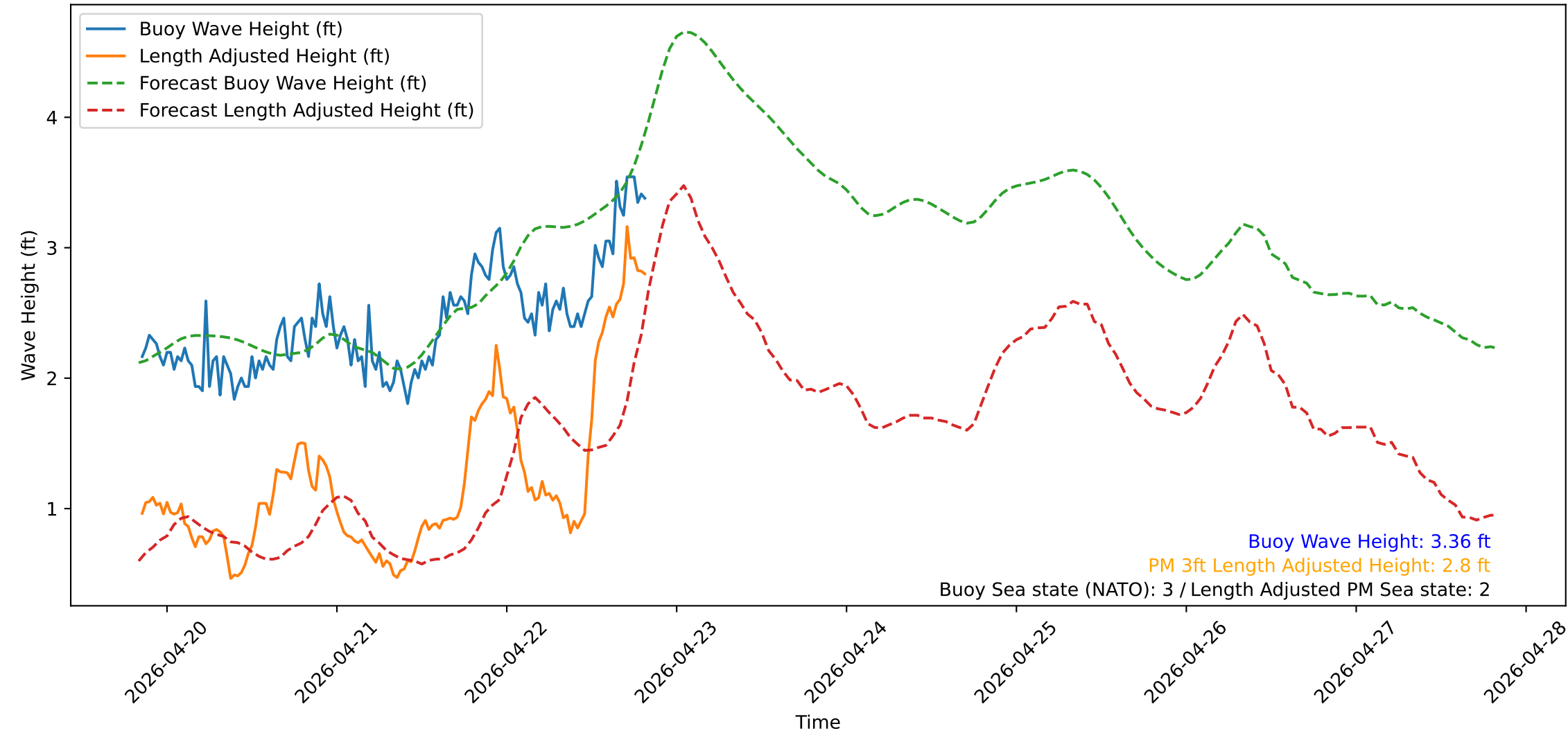
Wave Heights over Time for Red Beach at 2026-04-22 20:10:50
