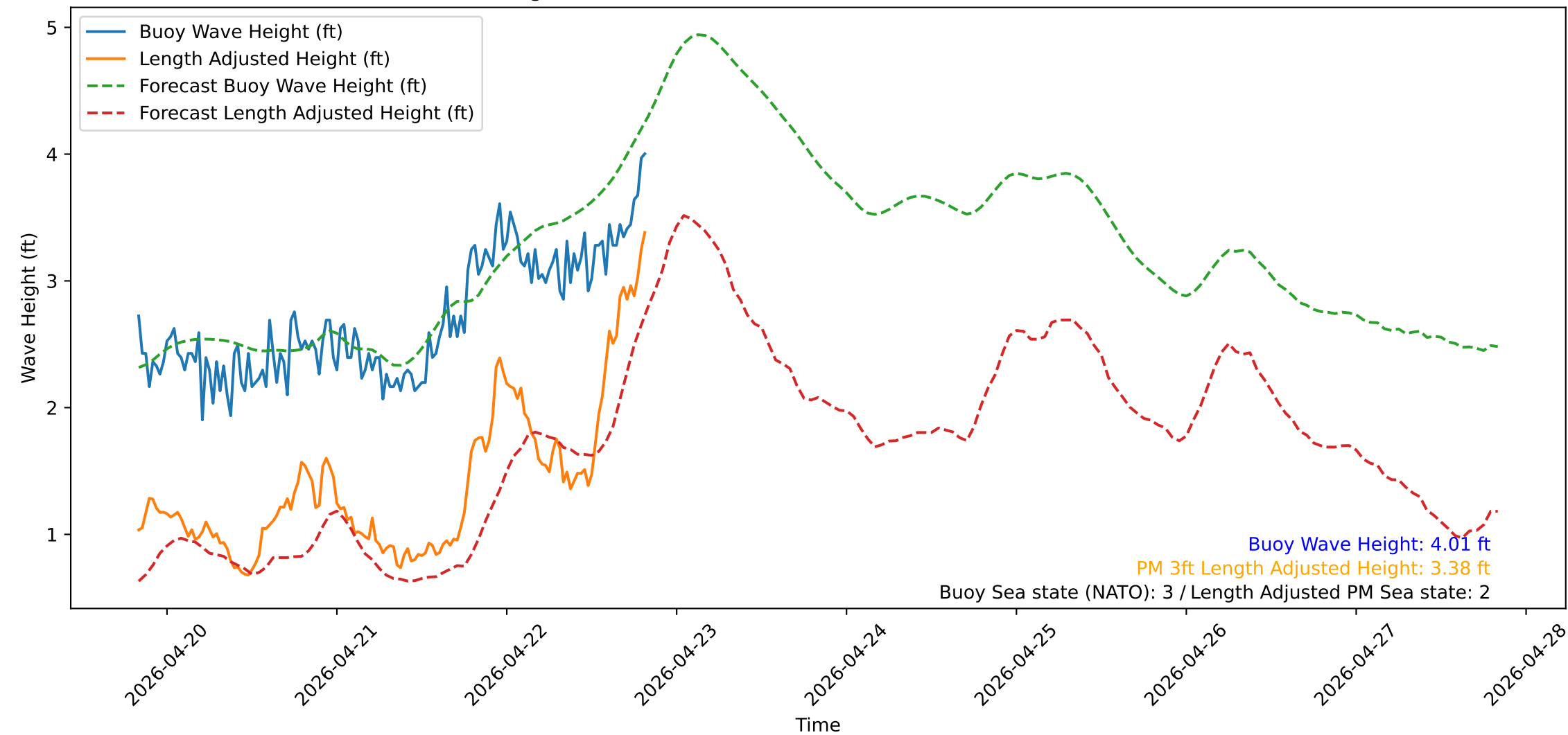
Wave Heights over Time for Oceanside Harbor at 2026-04-22 20:10:31
