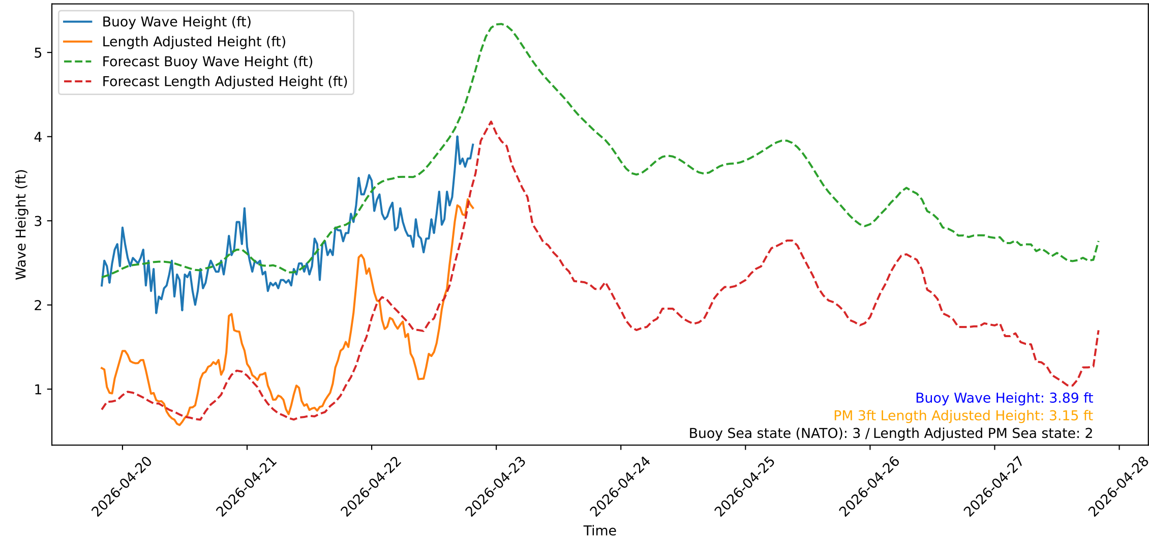
Wave Heights over Time for Green Beach at 2026-04-22 20:11:12
