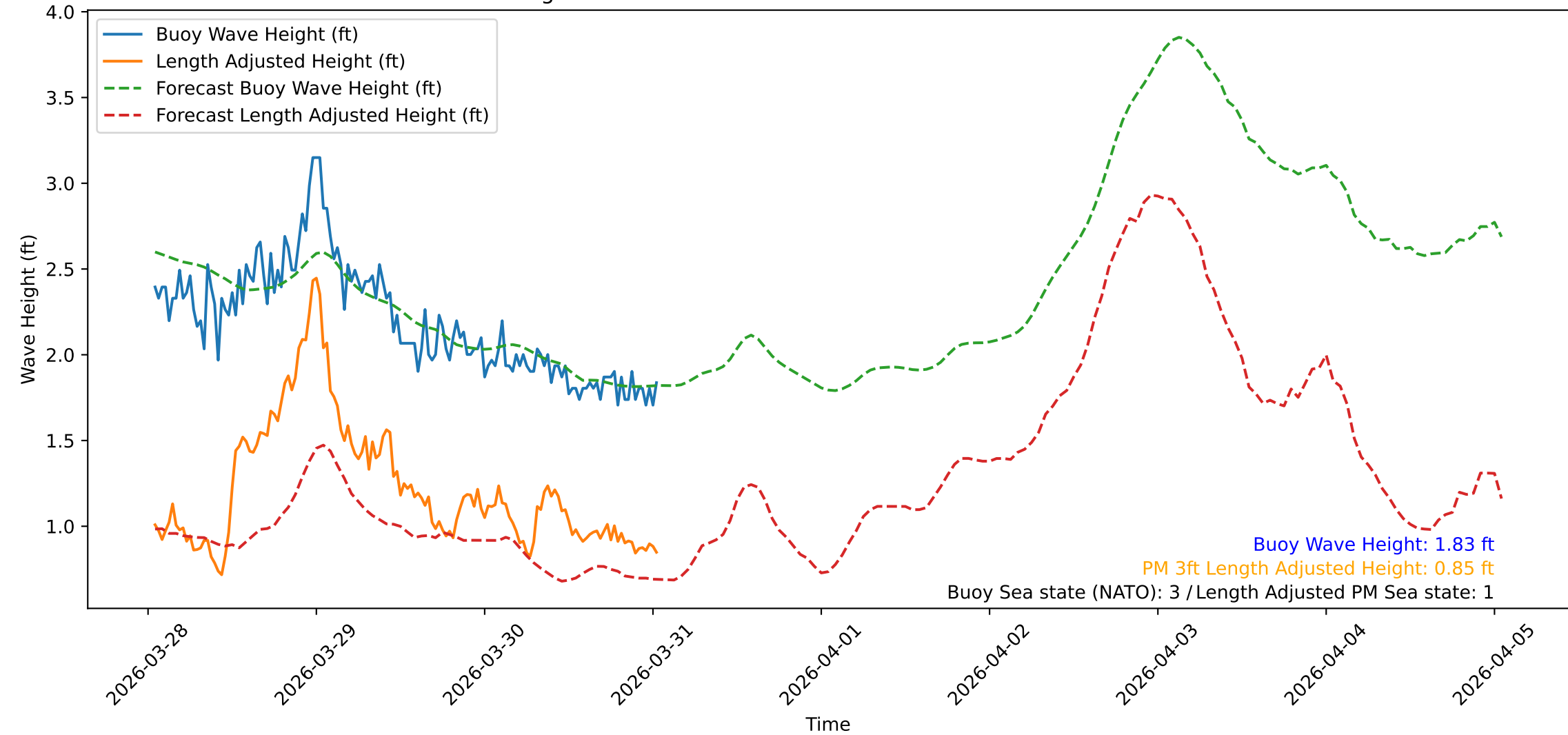
Wave Heights over Time for Oceanside Harbor at 2026-03-31 01:00:32
