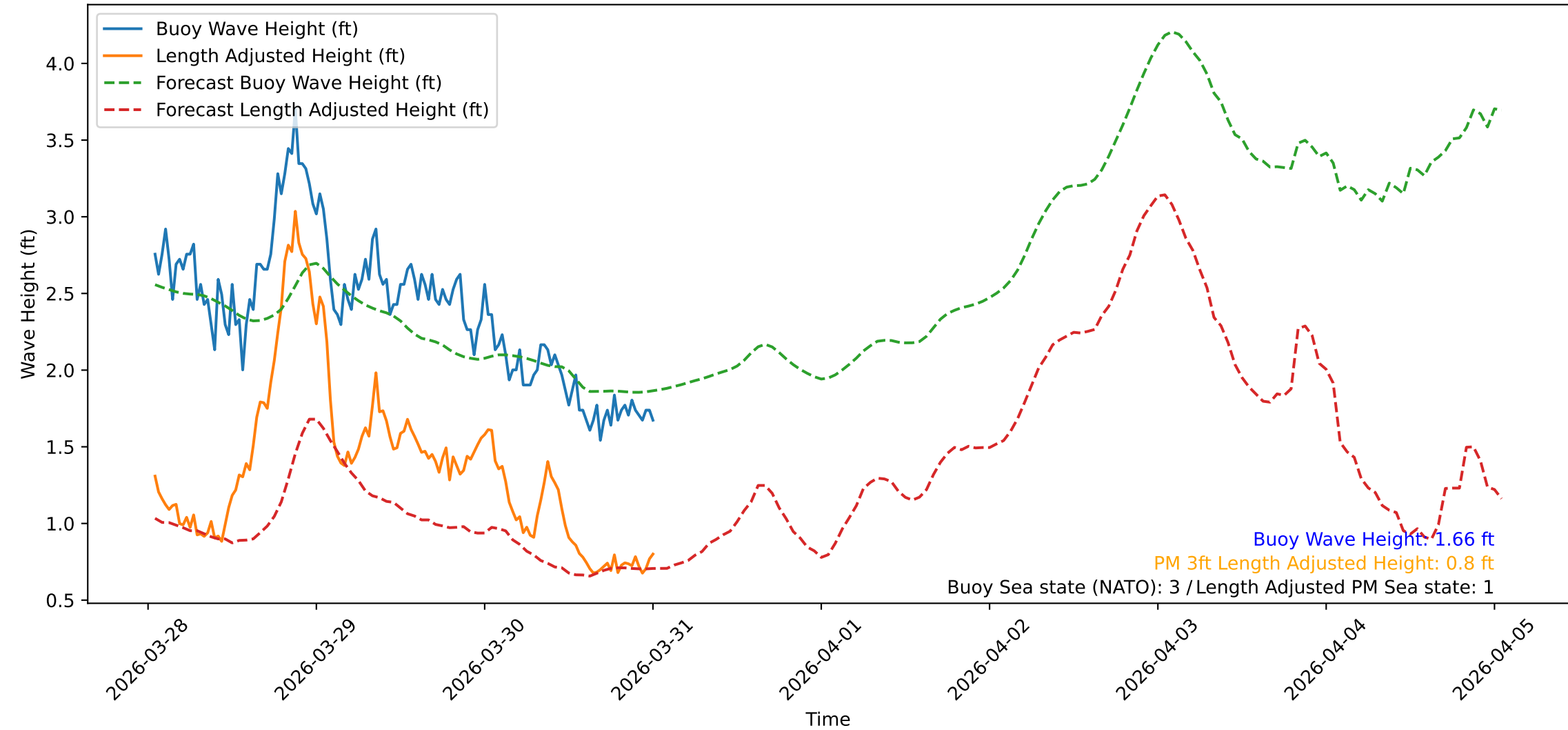
Wave Heights over Time for Green Beach at 2026-03-31 01:01:10
