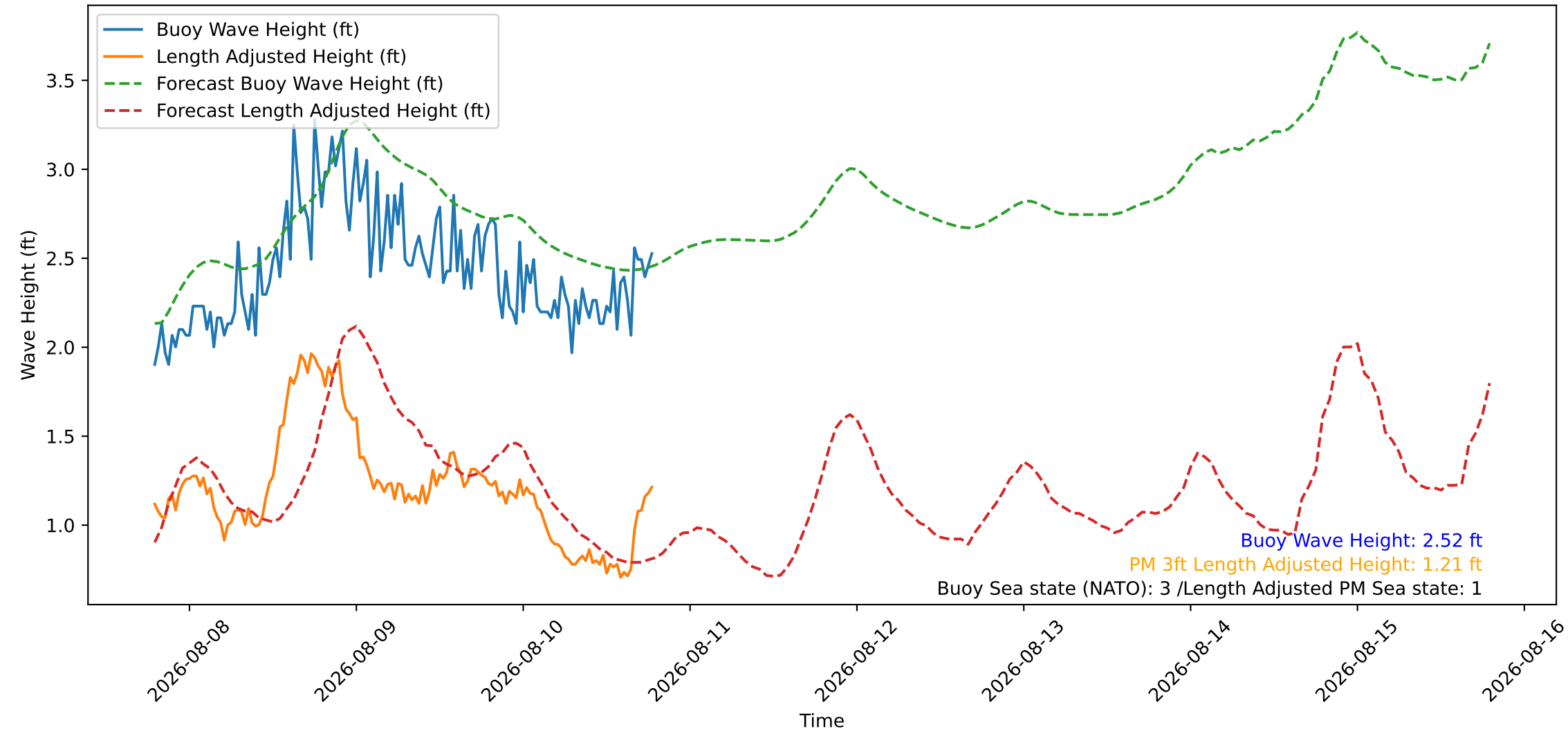
Wave Heights over Time for Oceanside Harbor at 2026-08-10 19:10:27
