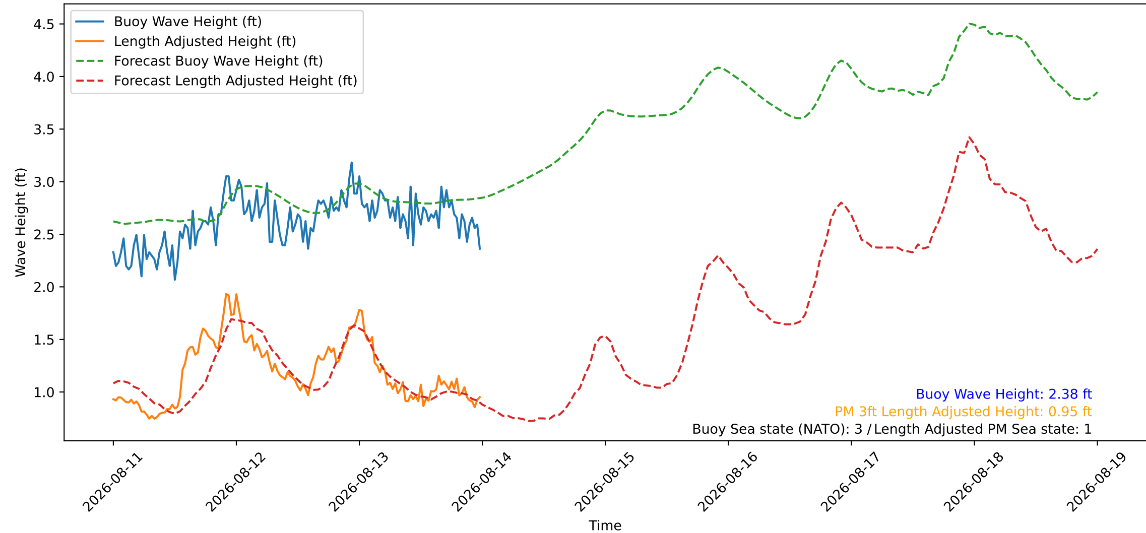
Wave Heights over Time for Oceanside Harbor at 2026-08-14 00:10:26
