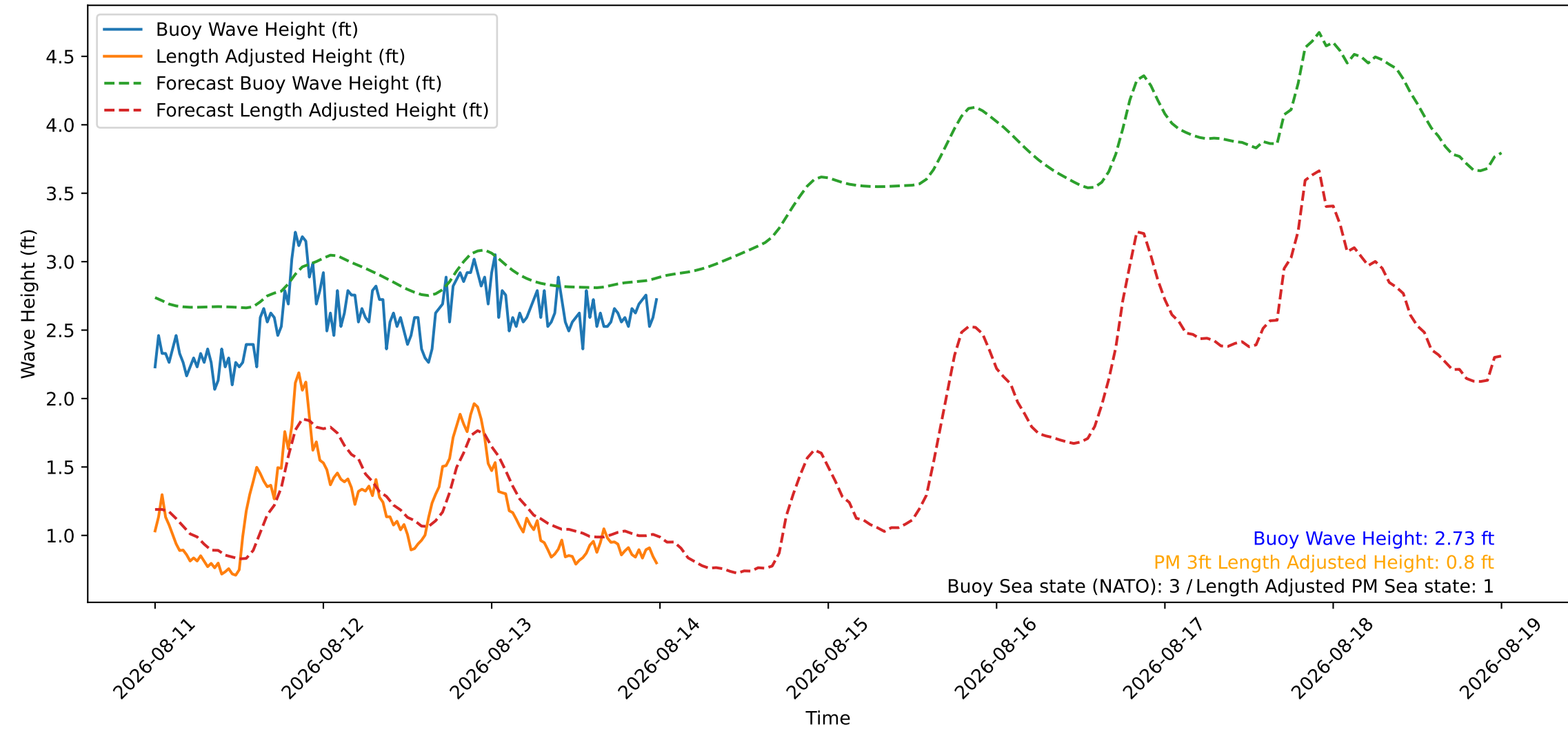
Wave Heights over Time for Green Beach at 2026-08-14 00:11:08
