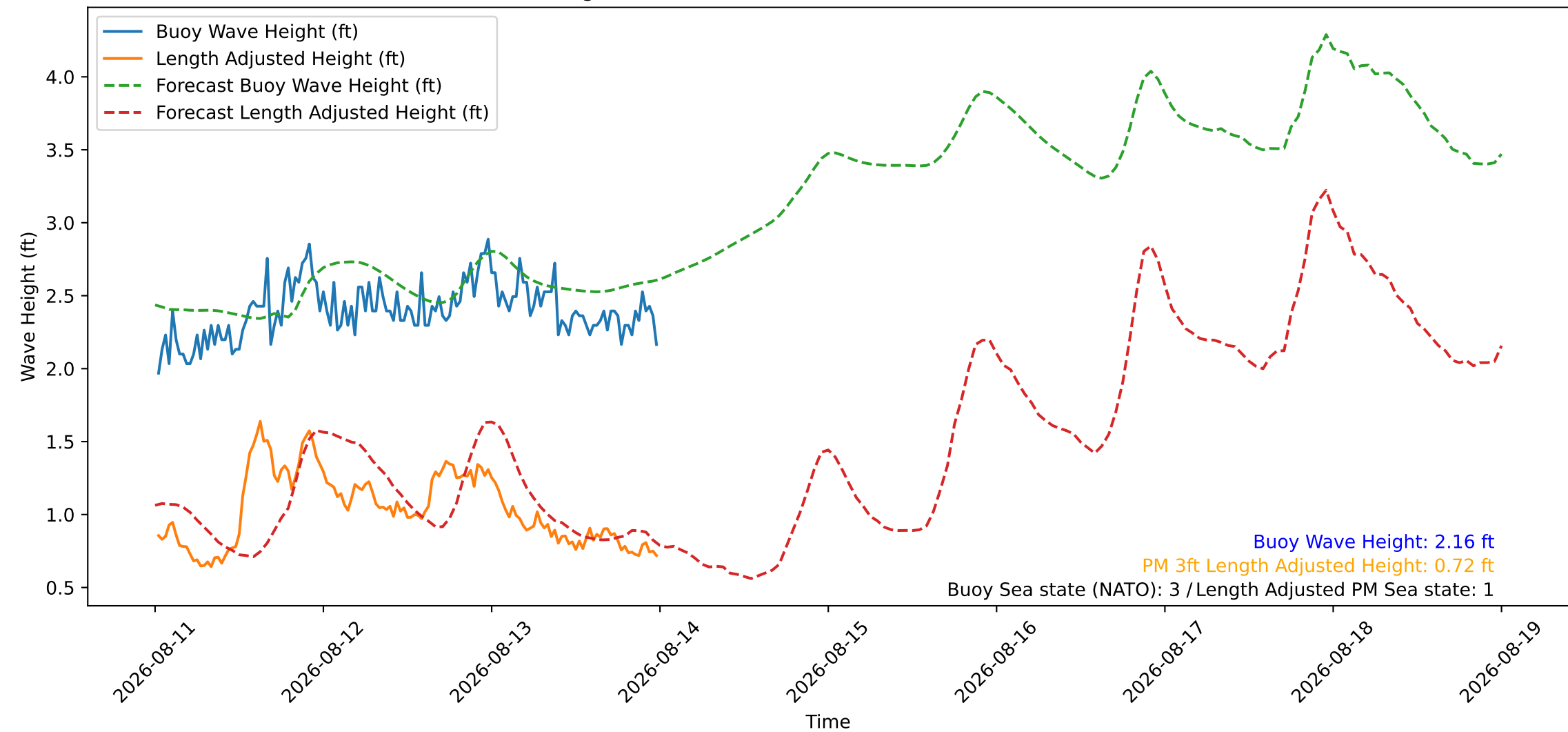
Wave Heights over Time for Red Beach at 2026-08-14 00:10:45
