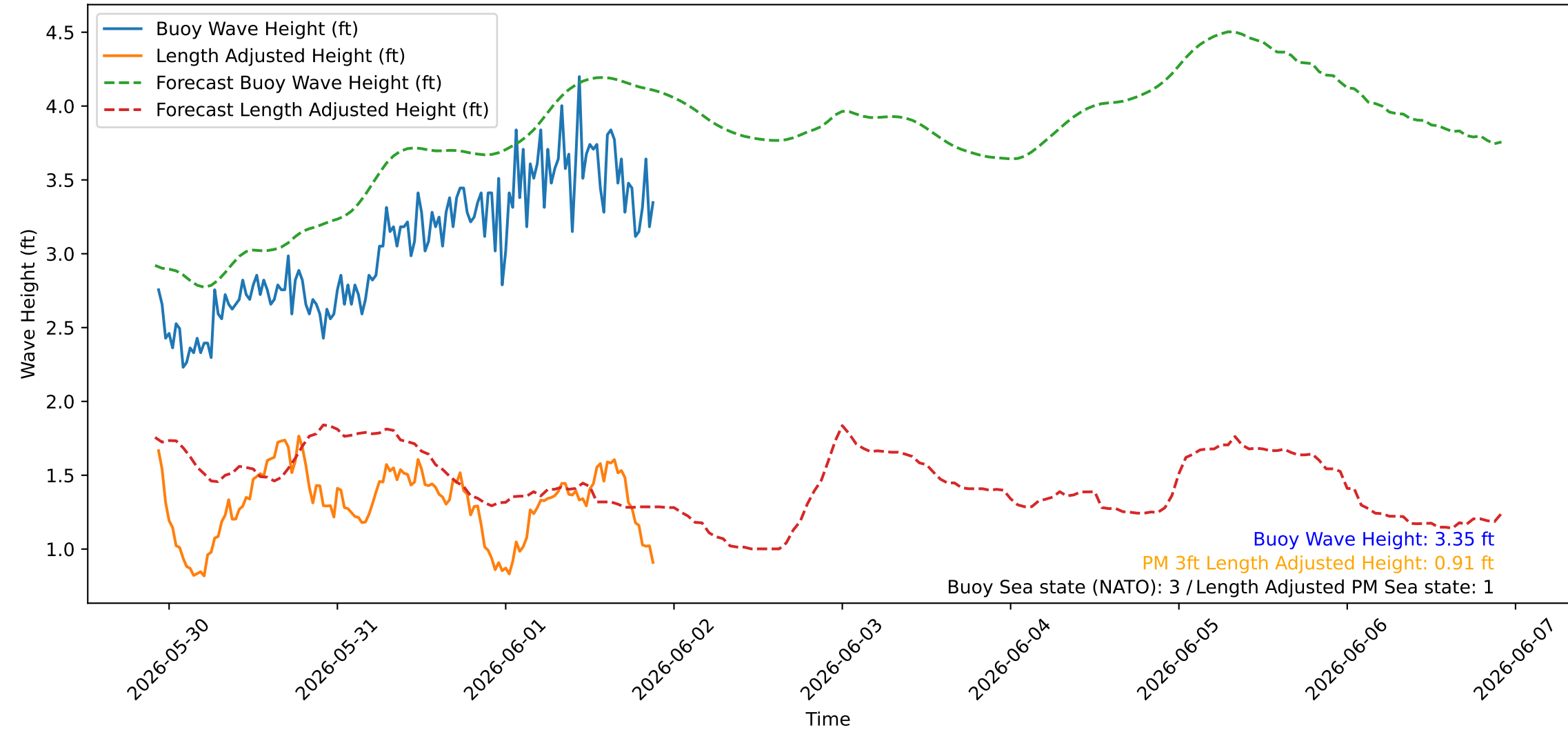
Wave Heights over Time for Red Beach at 2026-06-01 22:00:45
