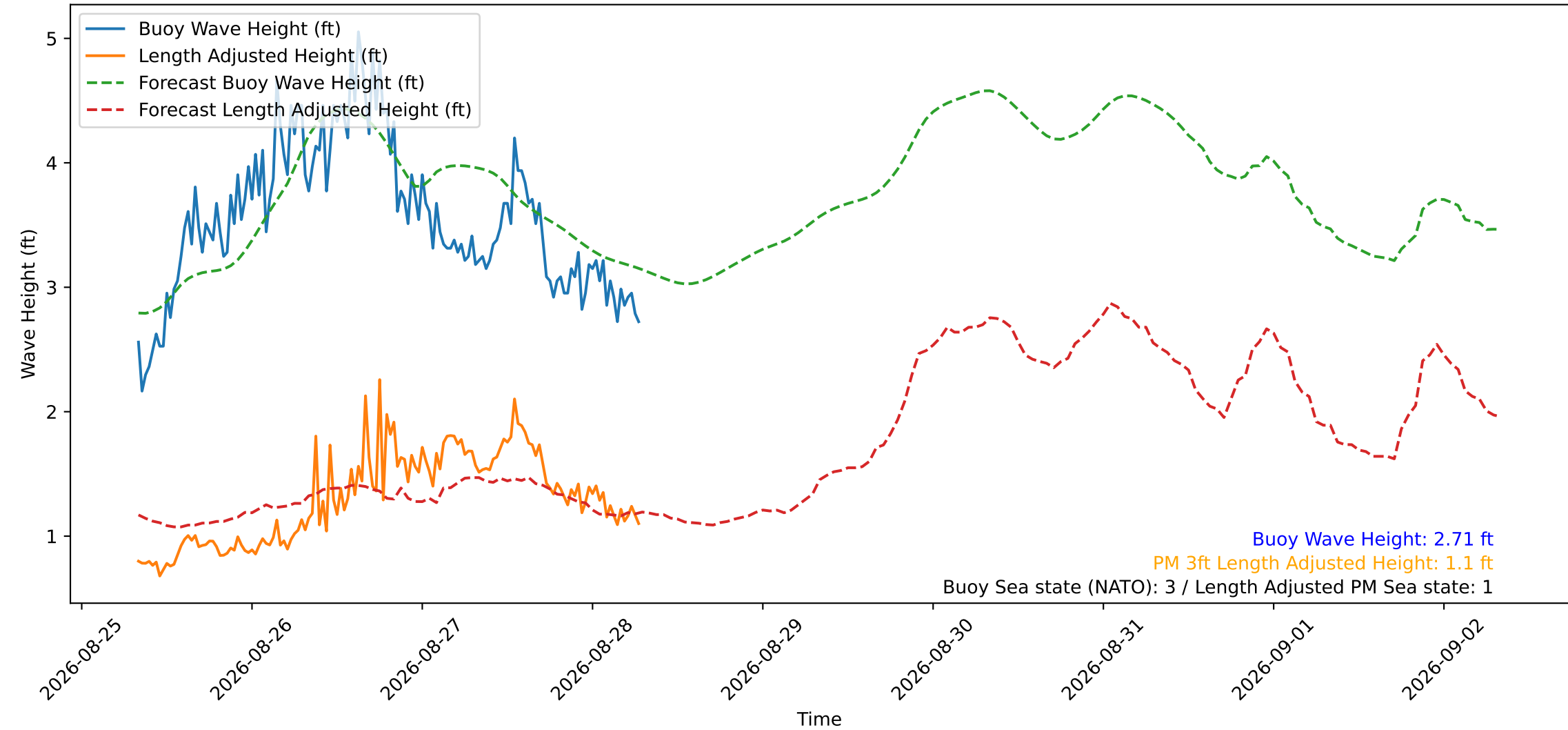
Wave Heights over Time for Red Beach at 2026-08-28 07:30:49
