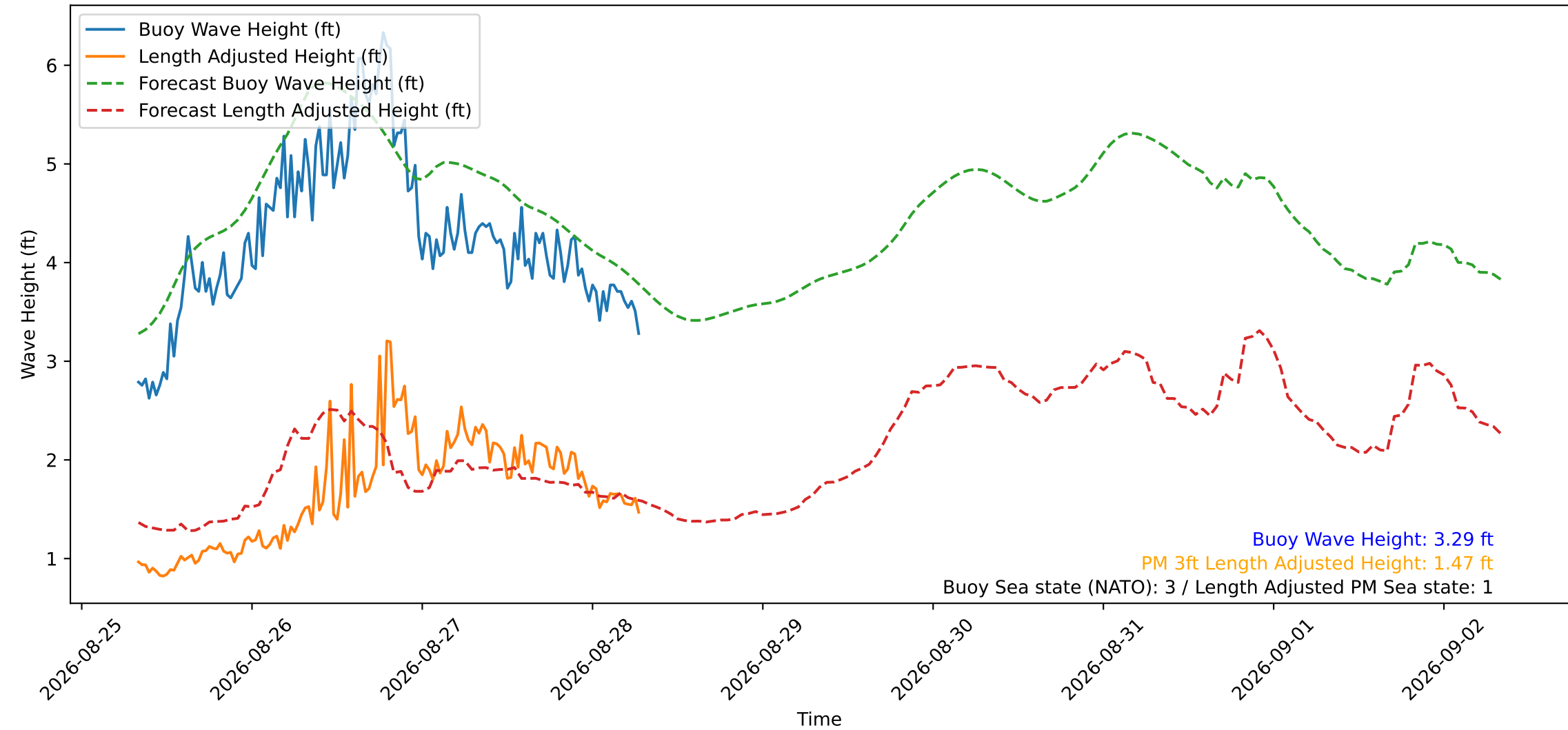
Wave Heights over Time for Green Beach at 2026-08-28 07:31:11
