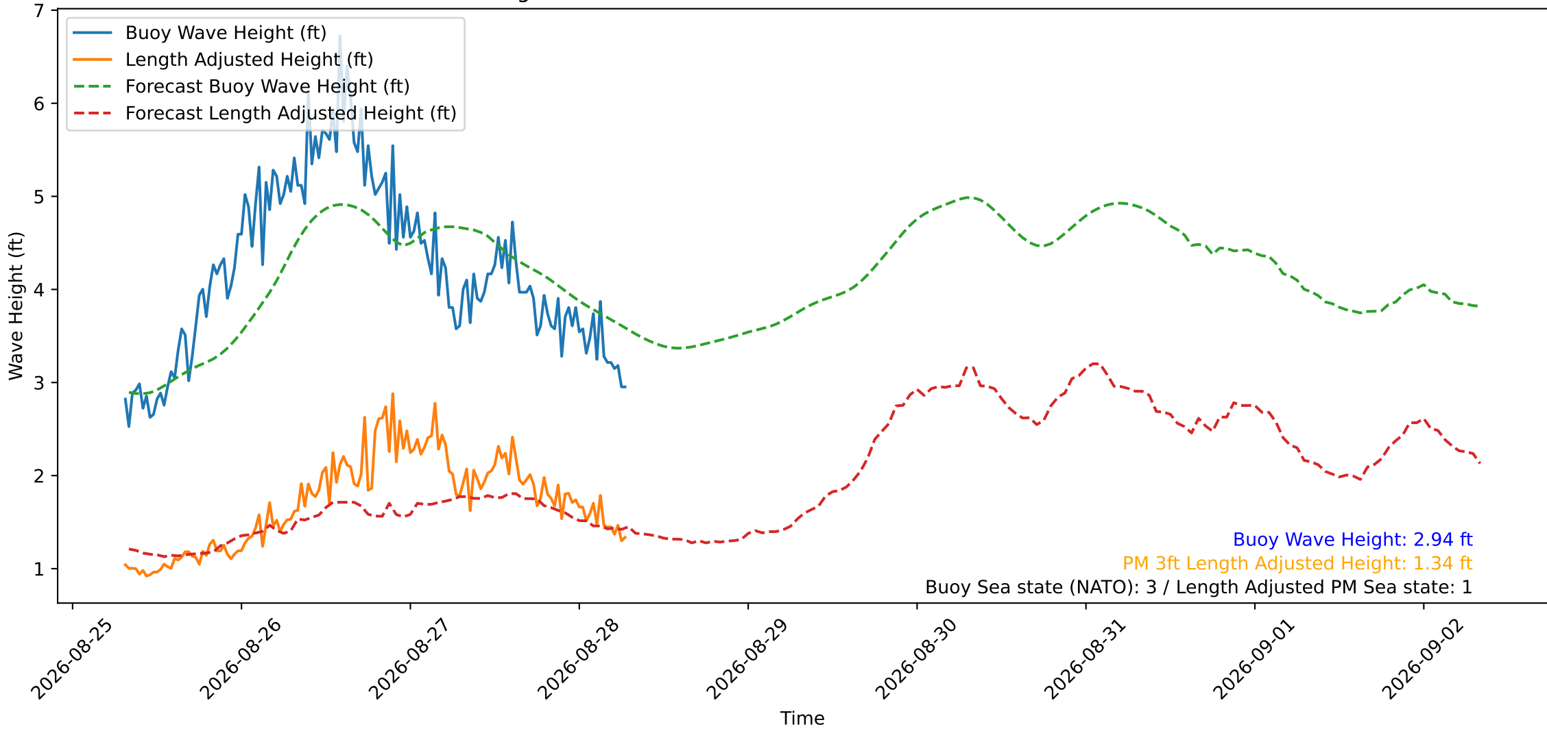
Wave Heights over Time for Oceanside Harbor at 2026-08-28 07:30:29
