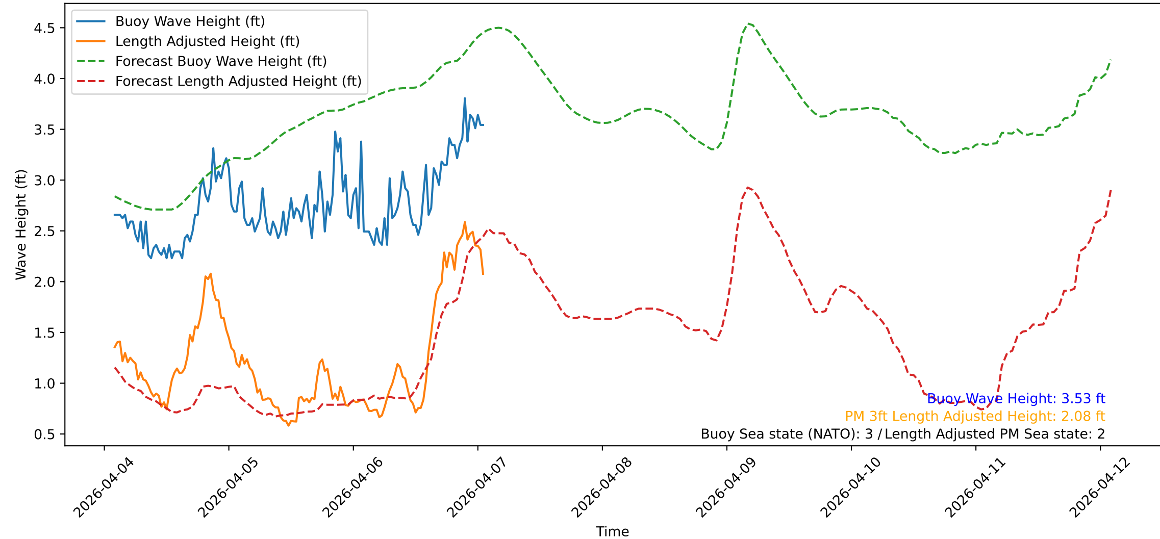
Wave Heights over Time for Green Beach at 2026-04-07 02:01:09
