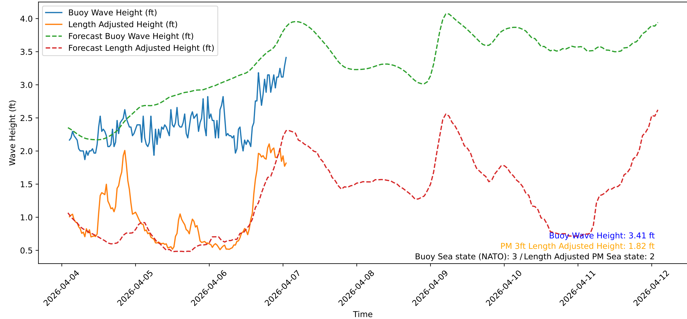
Wave Heights over Time for Red Beach at 2026-04-07 02:00:47
