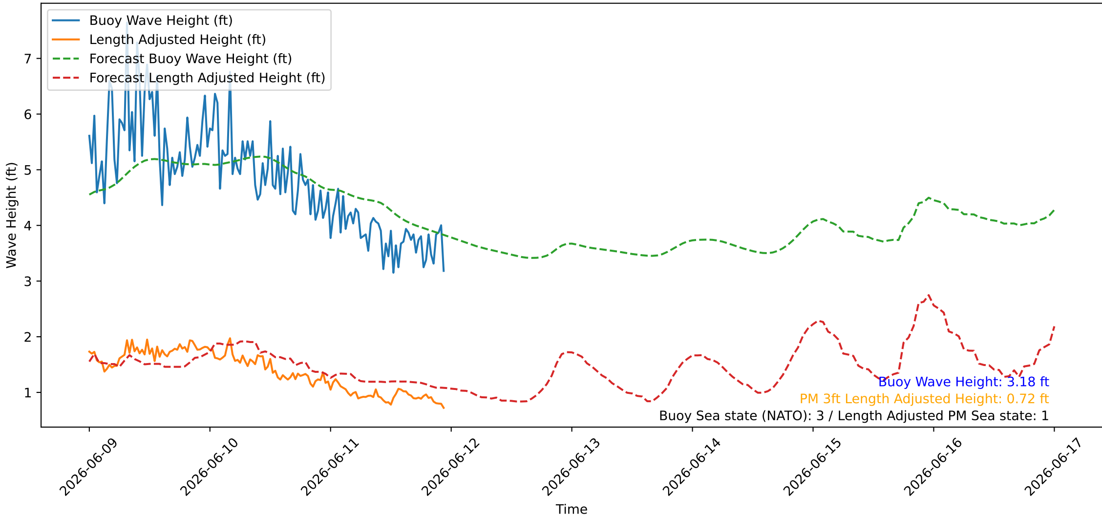
Wave Heights over Time for Red Beach at 2026-06-11 23:30:46
