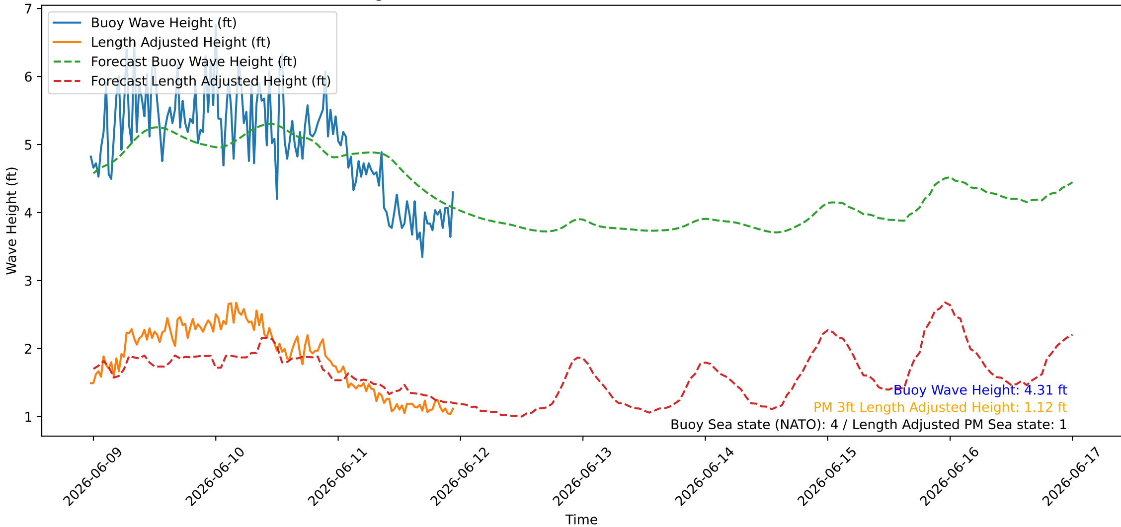
Wave Heights over Time for Oceanside Harbor at 2026-06-11 23:30:26
