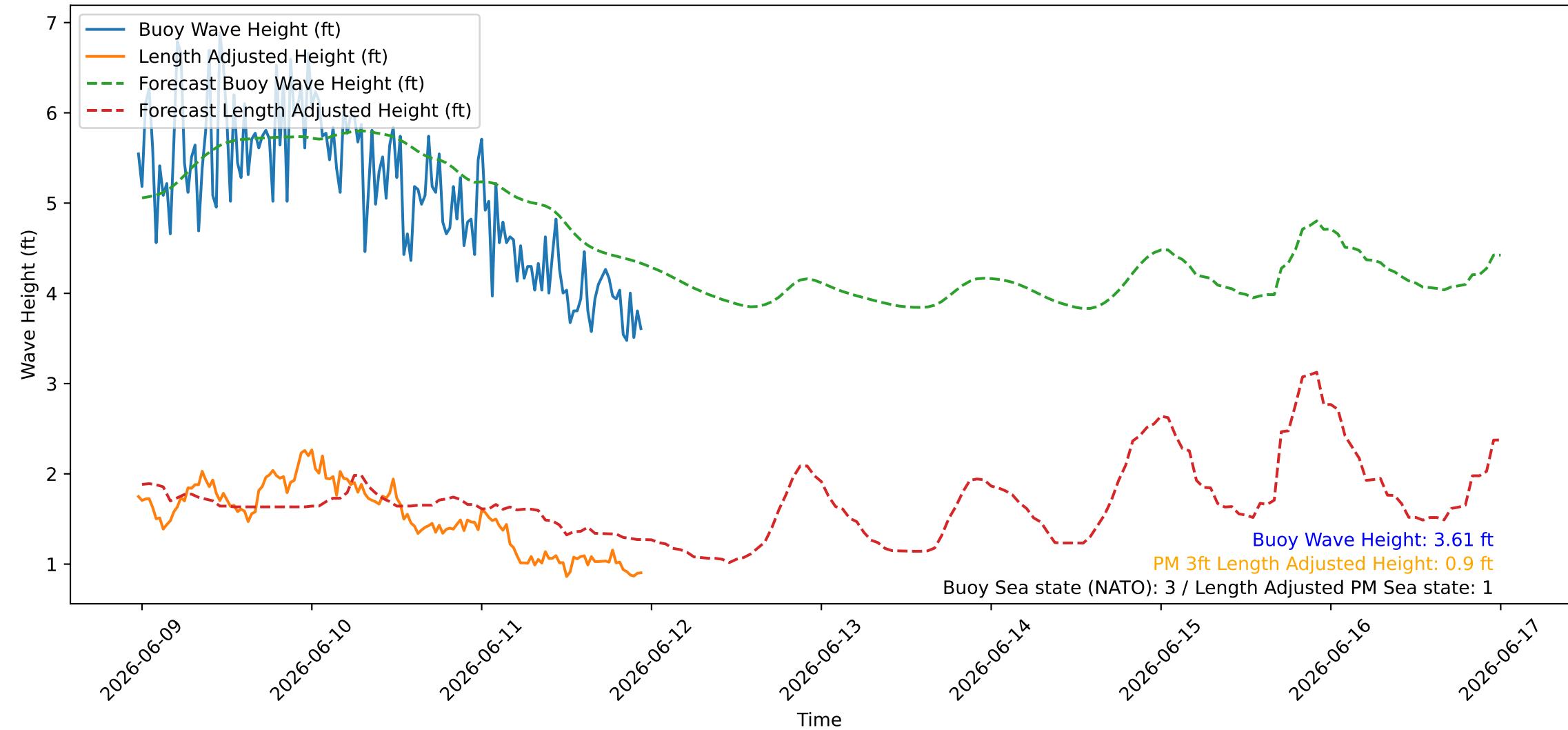
Wave Heights over Time for Green Beach at 2026-06-11 23:31:09
