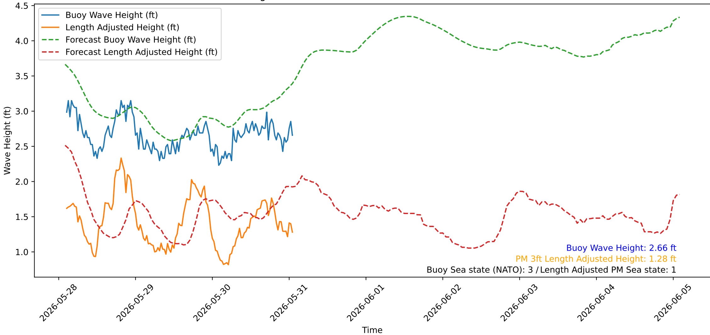
Wave Heights over Time for Red Beach at 2026-05-31 02:00:44
