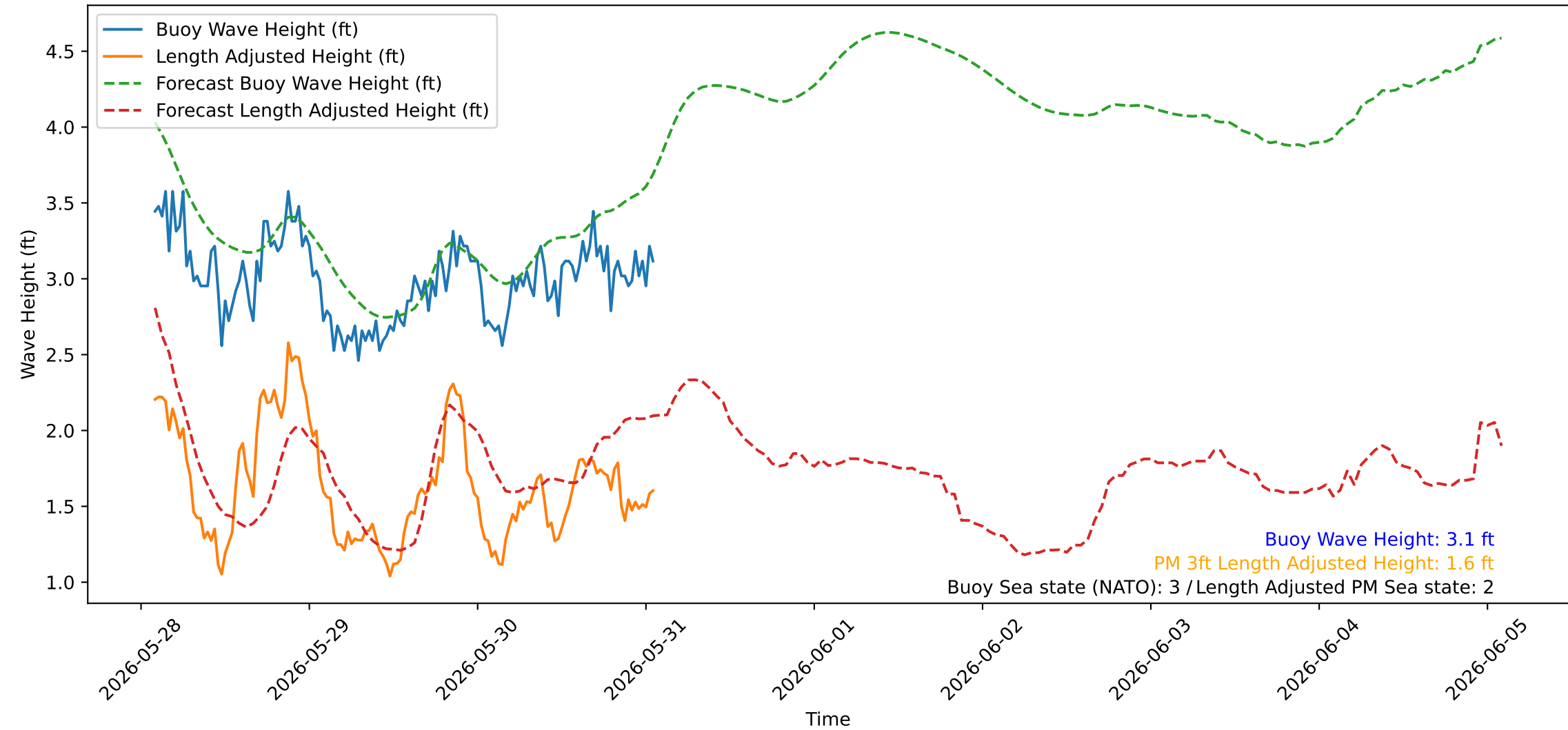
Wave Heights over Time for Green Beach at 2026-05-31 02:01:06
