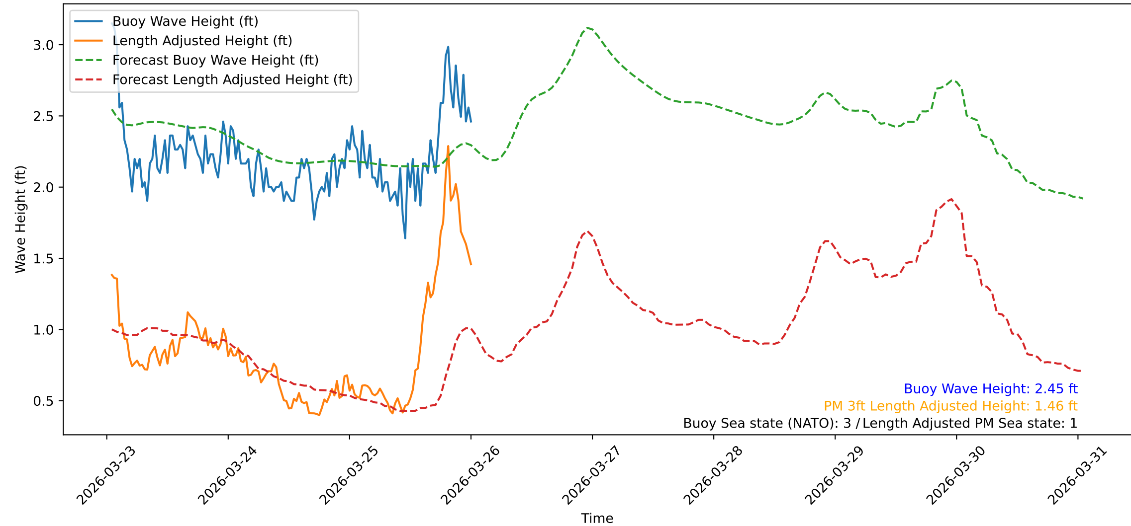
Wave Heights over Time for Green Beach at 2026-03-26 01:01:09
