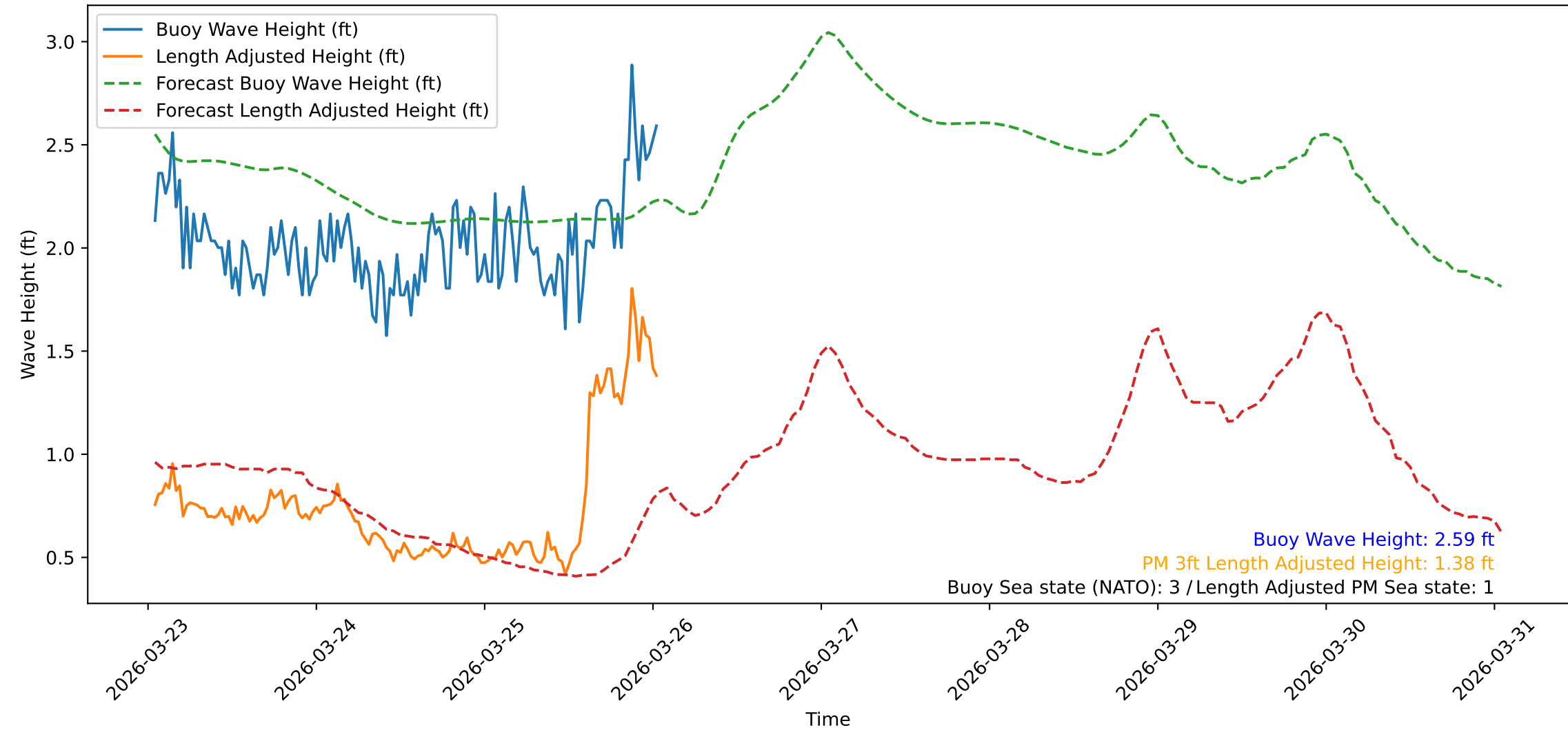
Wave Heights over Time for Oceanside Harbor at 2026-03-26 01:00:31
