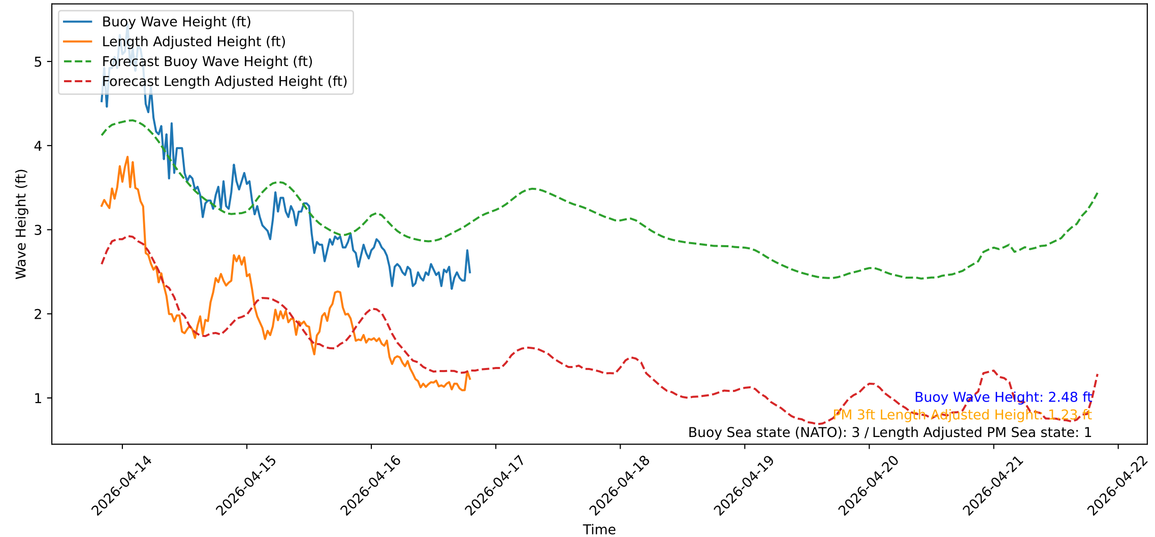
Wave Heights over Time for Oceanside Harbor at 2026-04-16 19:50:31
