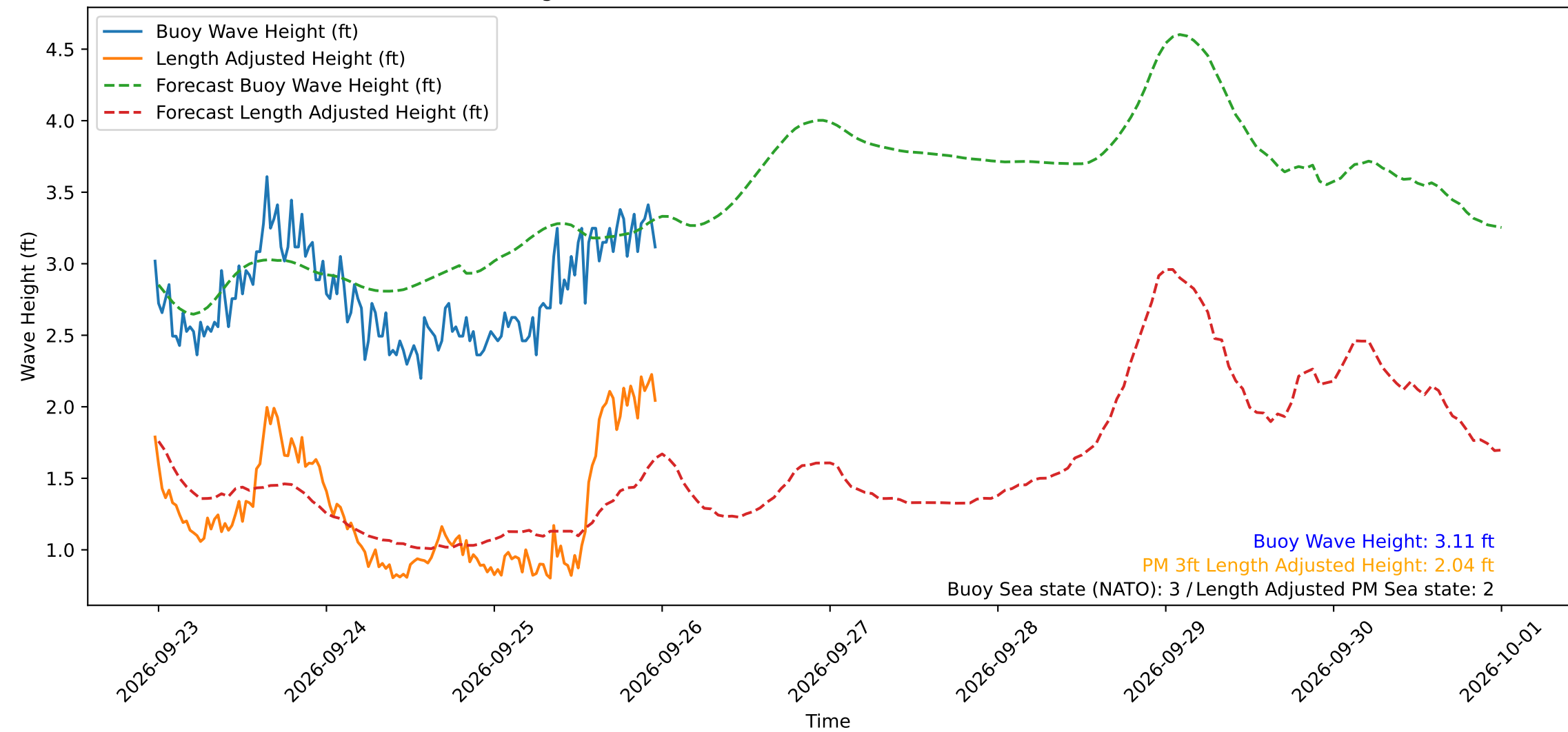
Wave Heights over Time for Oceanside Harbor at 2026-09-25 23:40:30
