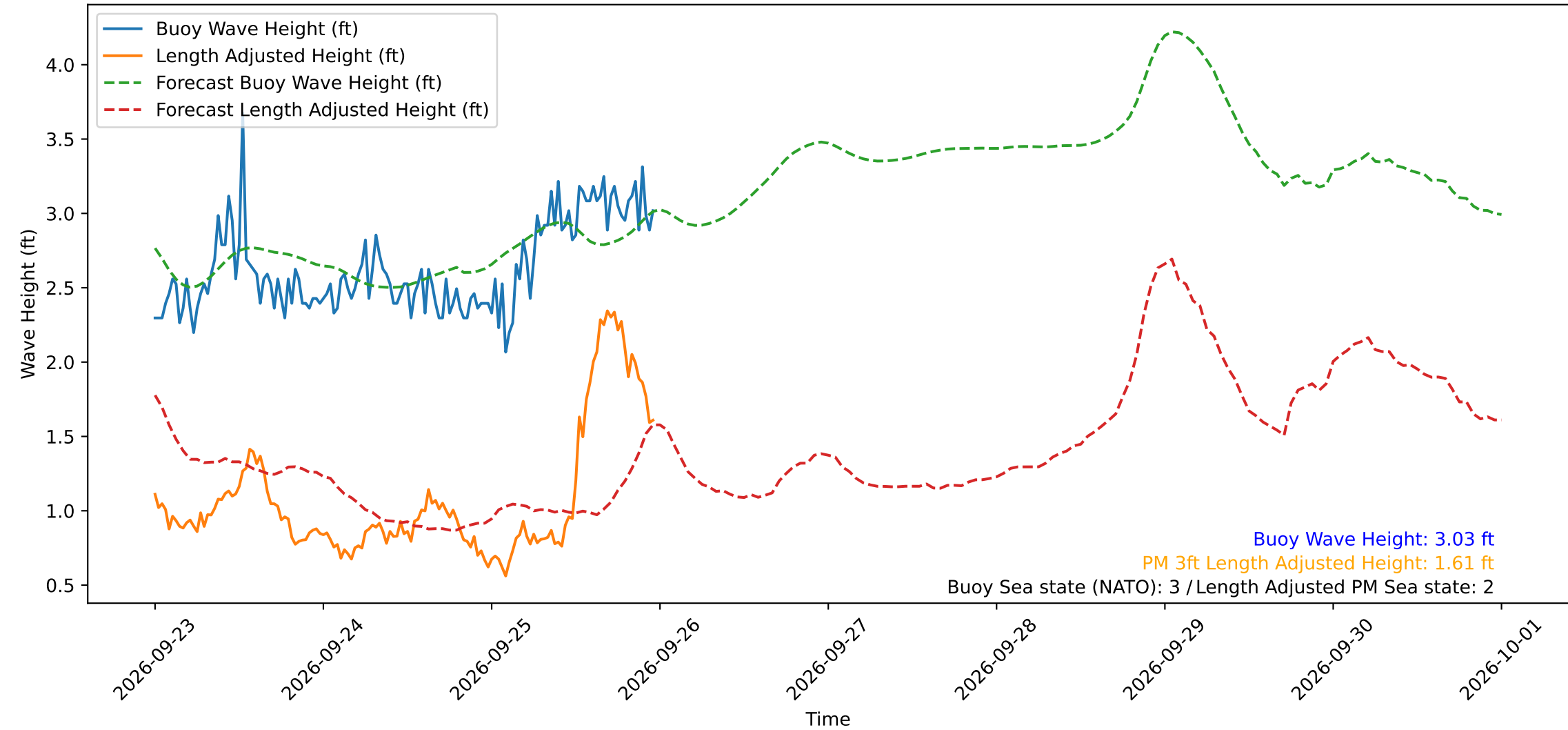
Wave Heights over Time for Red Beach at 2026-09-25 23:40:50
