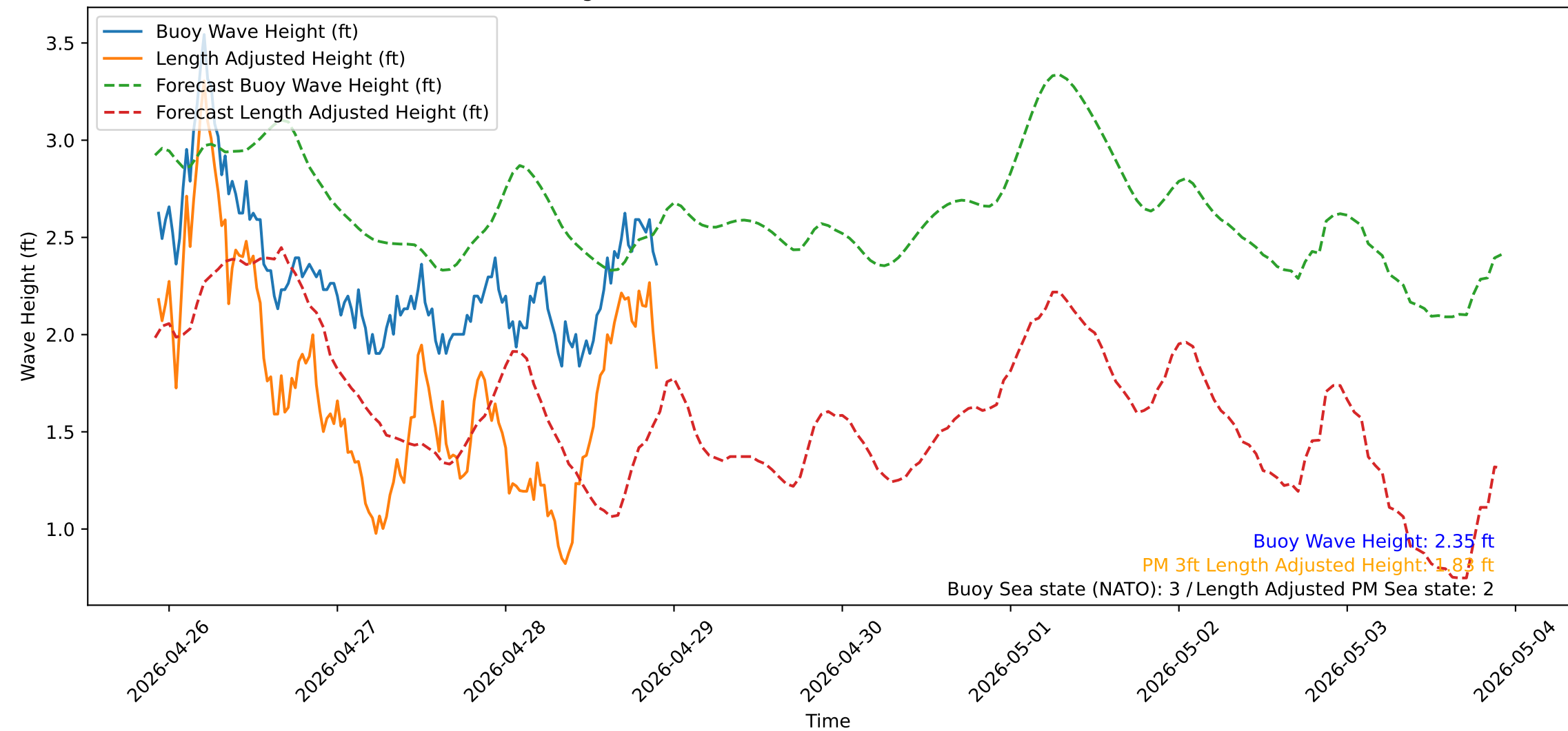
Wave Heights over Time for Red Beach at 2026-04-28 22:20:52
