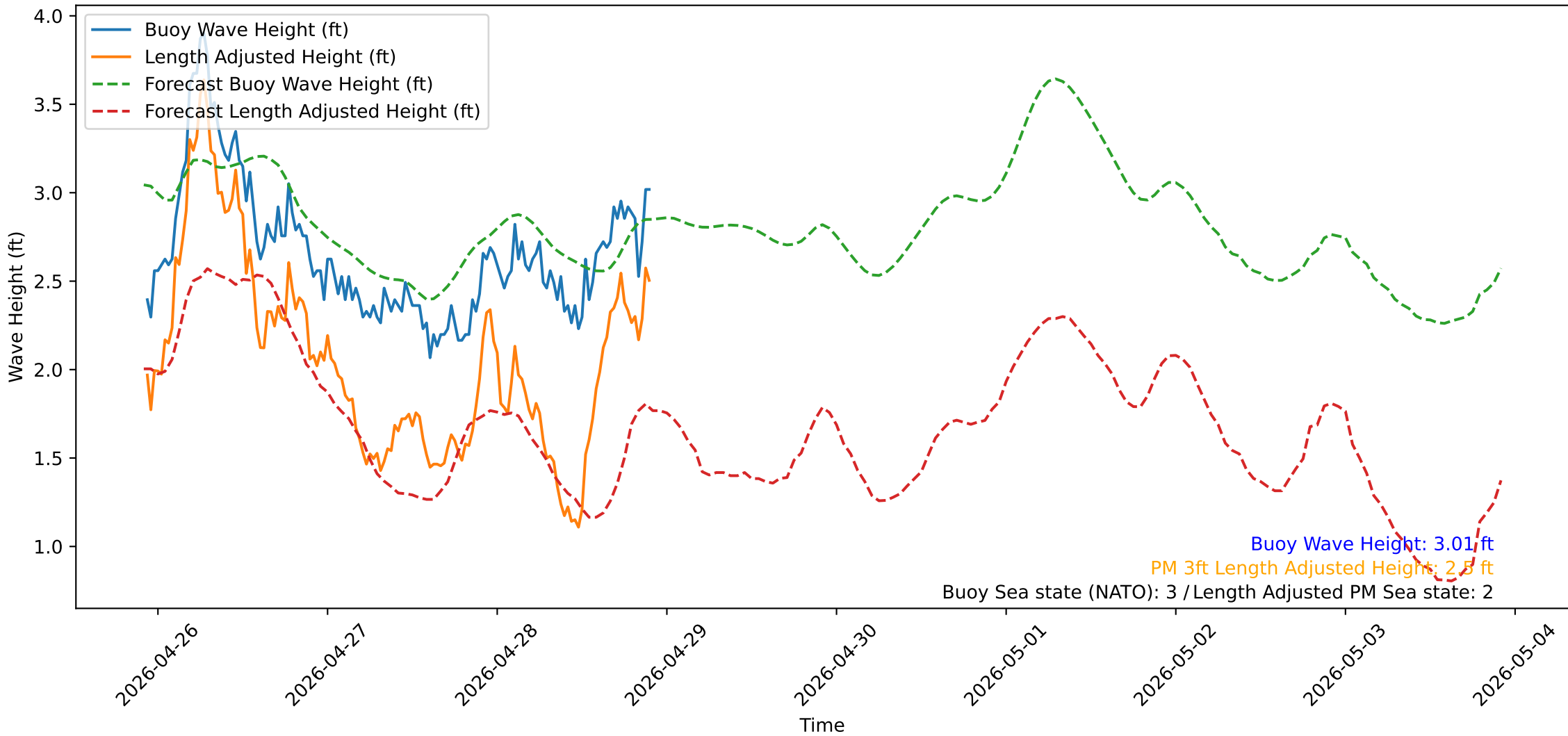
Wave Heights over Time for Oceanside Harbor at 2026-04-28 22:20:31
