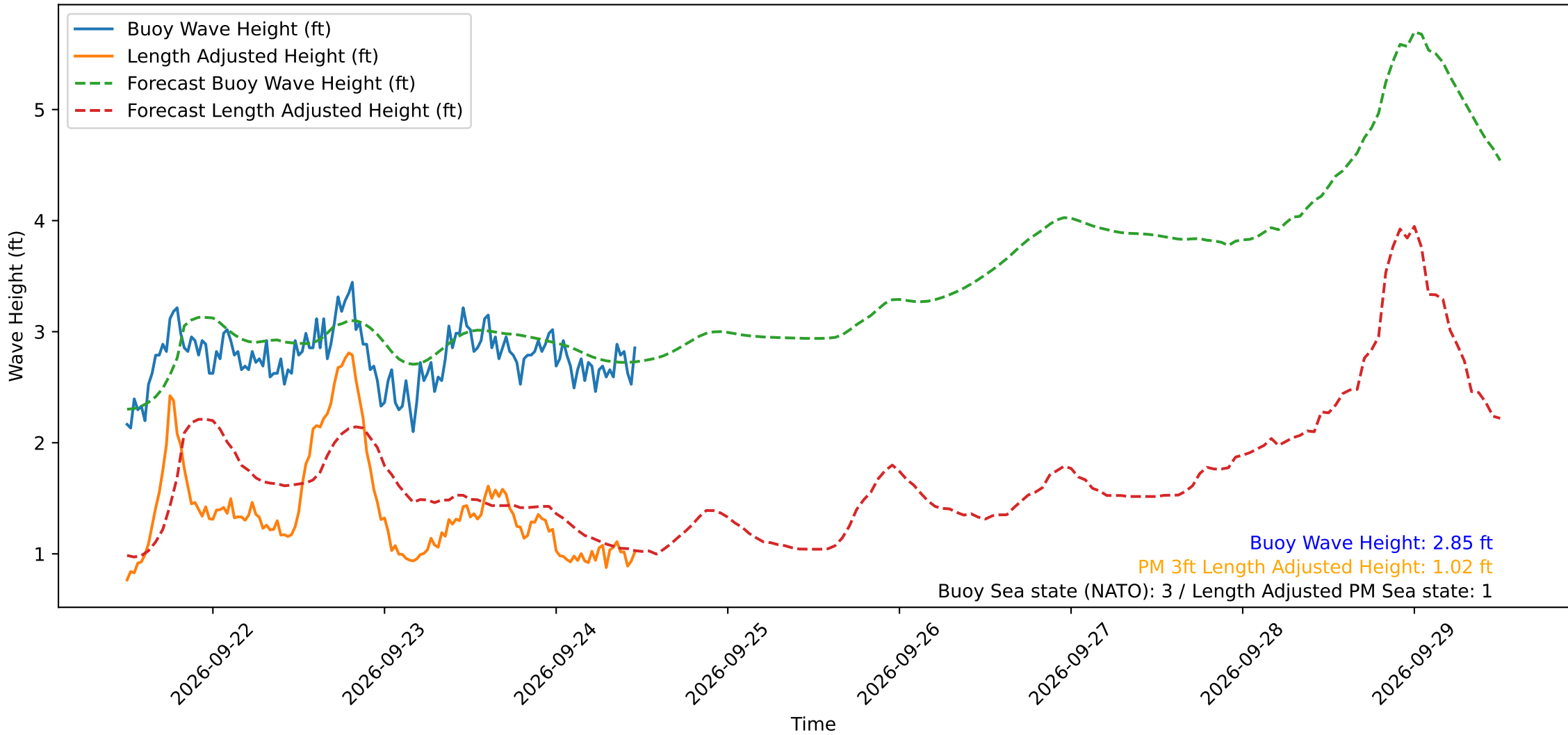
Wave Heights over Time for Green Beach at 2026-09-24 11:51:14
