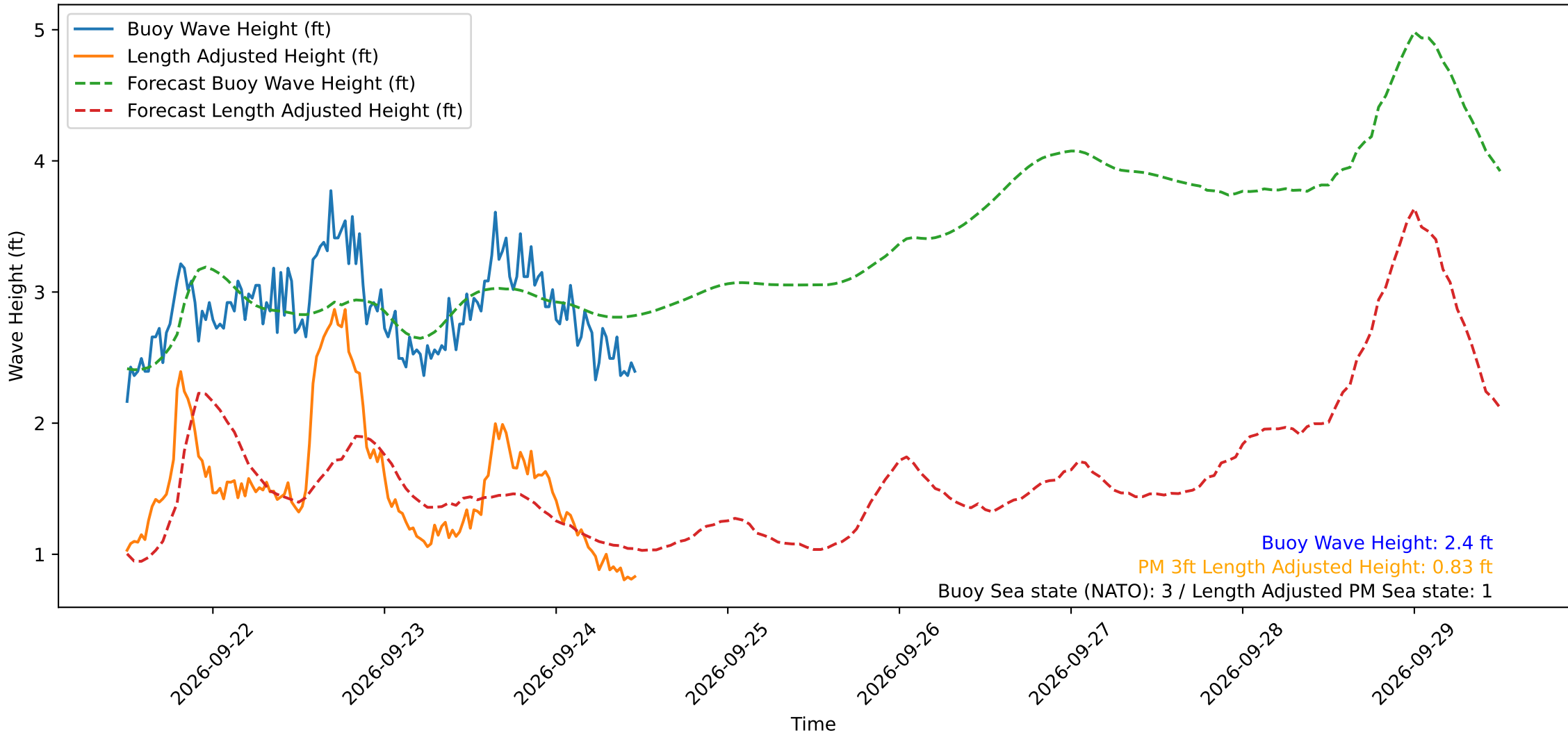
Wave Heights over Time for Oceanside Harbor at 2026-09-24 11:50:30
