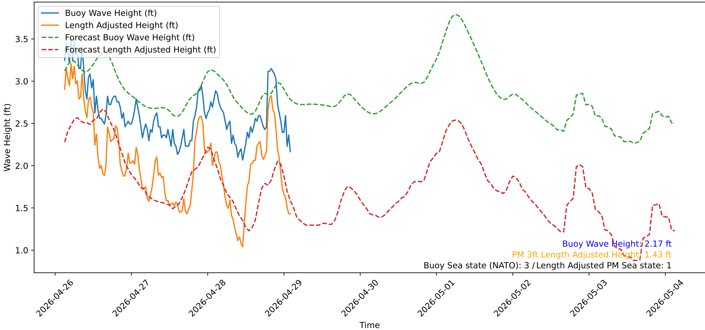
Wave Heights over Time for Green Beach at 2026-04-29 03:01:12
