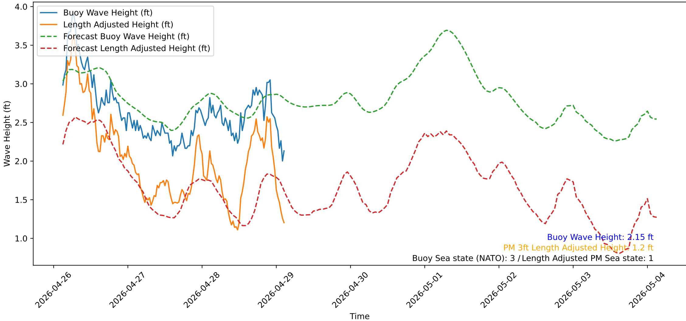
Wave Heights over Time for Oceanside Harbor at 2026-04-29 03:00:31
