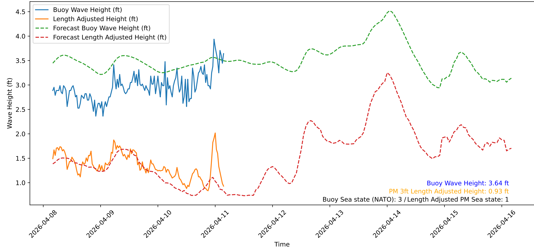
Wave Heights over Time for Green Beach at 2026-04-11 04:11:13
