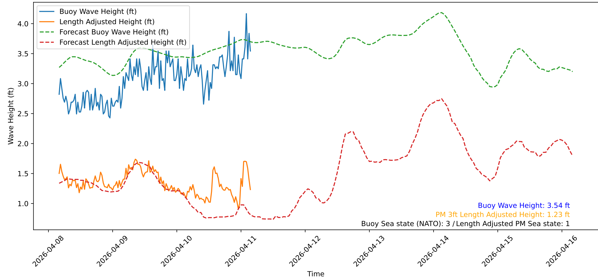
Wave Heights over Time for Oceanside Harbor at 2026-04-11 04:10:31
