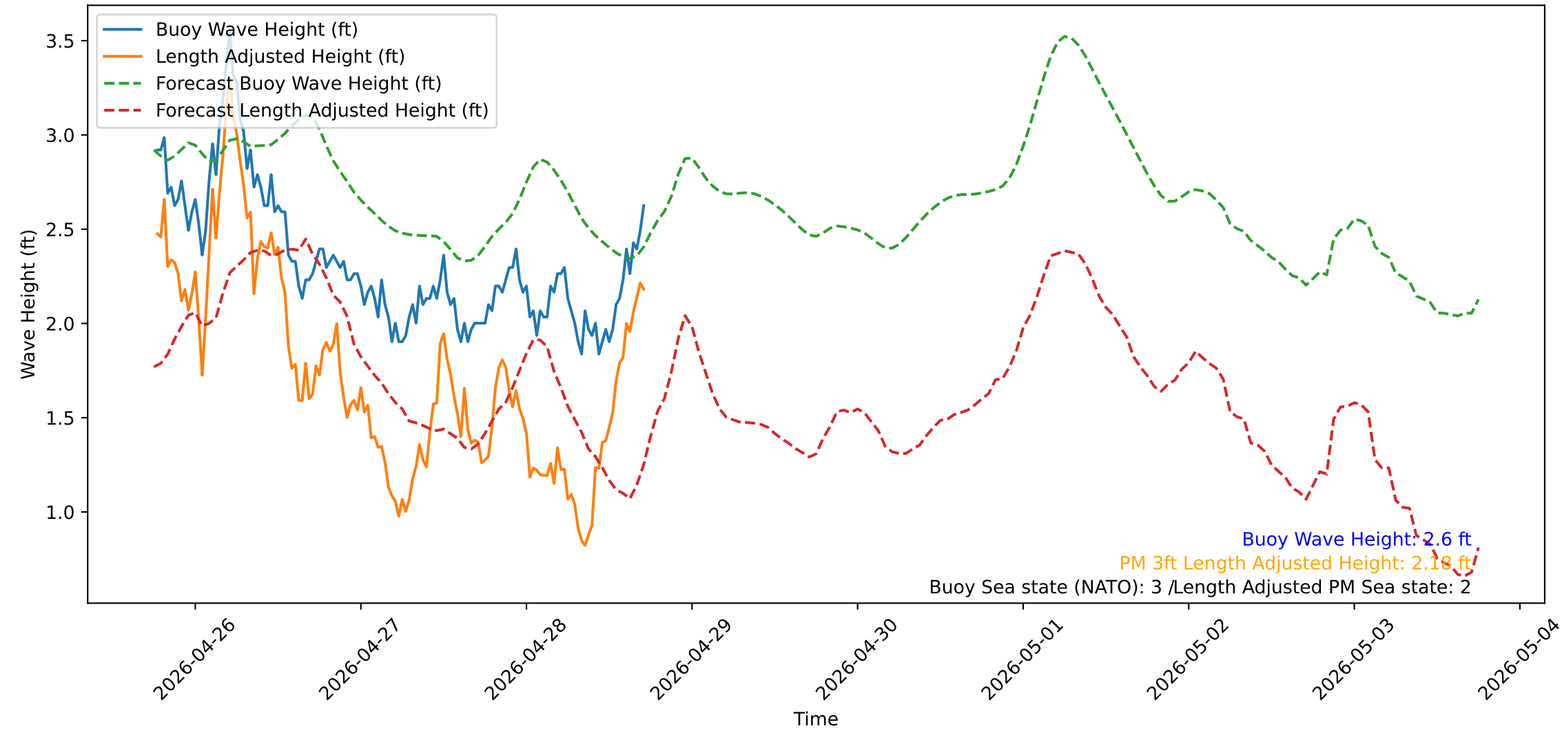
Wave Heights over Time for Red Beach at 2026-04-28 18:00:50
