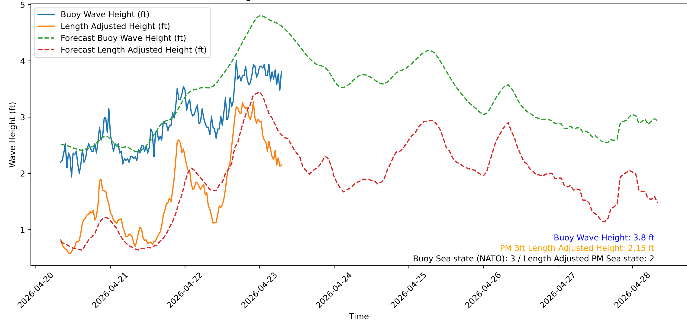
Wave Heights over Time for Green Beach at 2026-04-23 07:51:13
