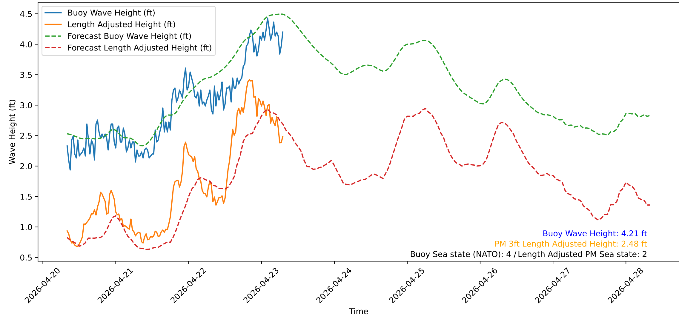
Wave Heights over Time for Oceanside Harbor at 2026-04-23 07:50:31
