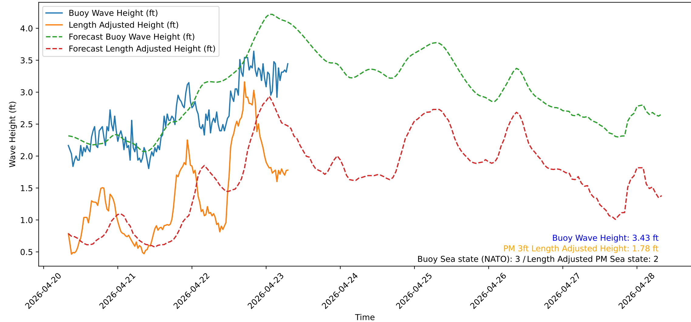
Wave Heights over Time for Red Beach at 2026-04-23 07:50:51
