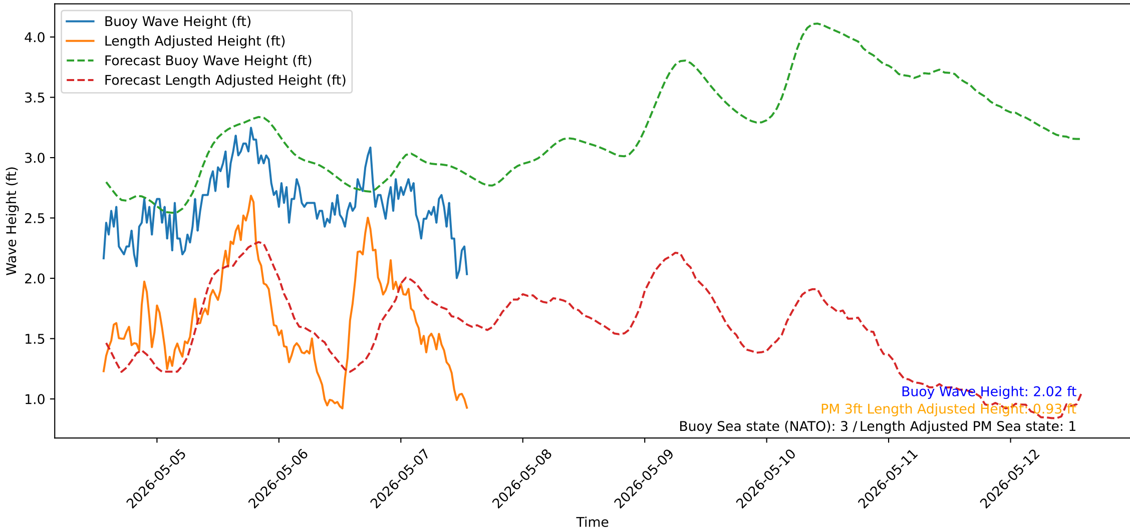
Wave Heights over Time for Oceanside Harbor at 2026-05-07 13:30:31
