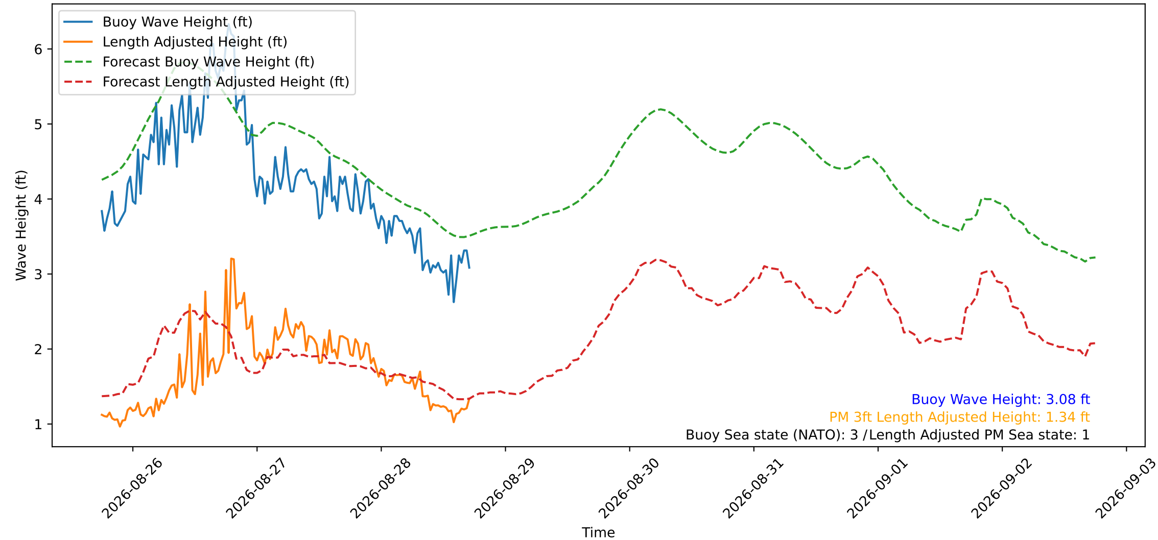
Wave Heights over Time for Green Beach at 2026-08-28 17:51:15
