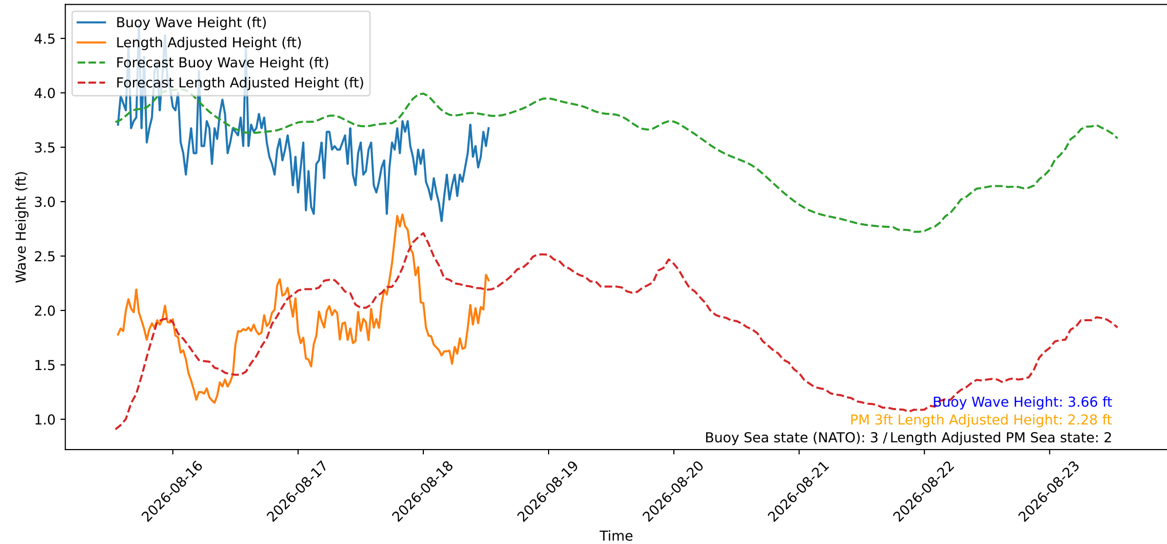
Wave Heights over Time for Oceanside Harbor at 2026-08-18 13:20:26
