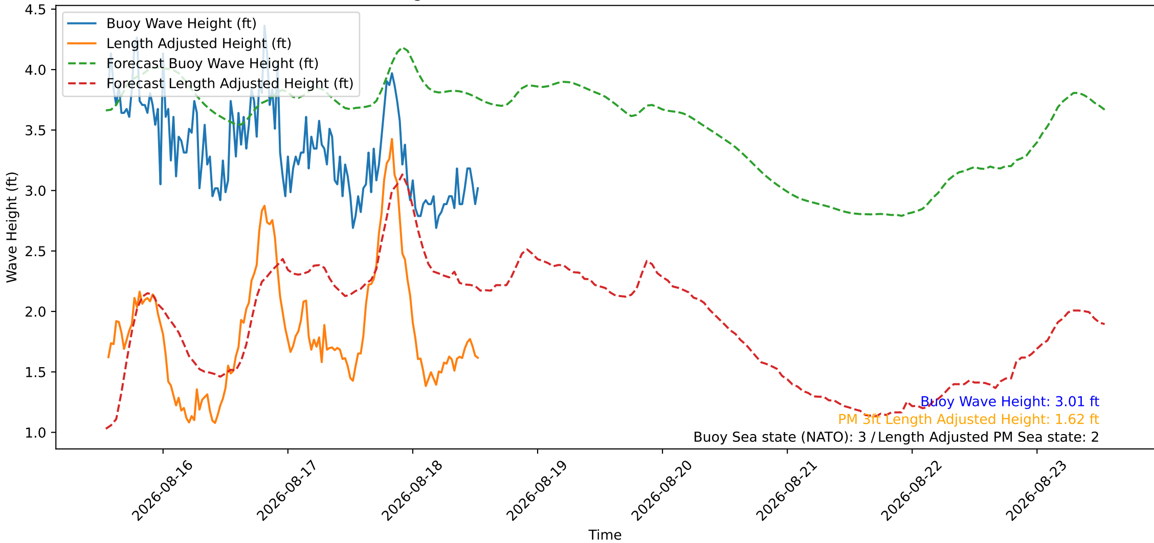
Wave Heights over Time for Green Beach at 2026-08-18 13:21:11
