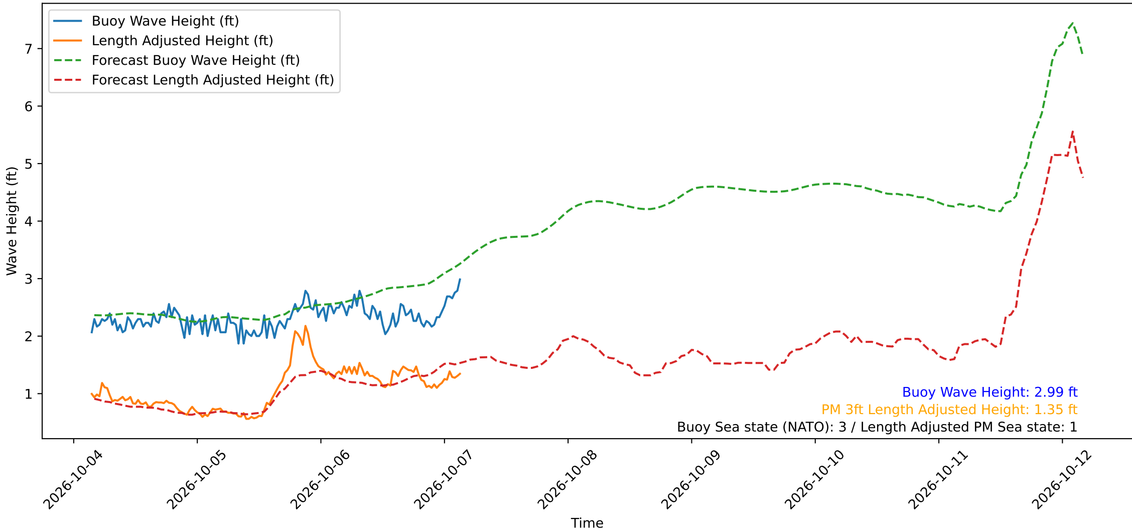
Wave Heights over Time for Oceanside Harbor at 2026-10-07 03:40:29
