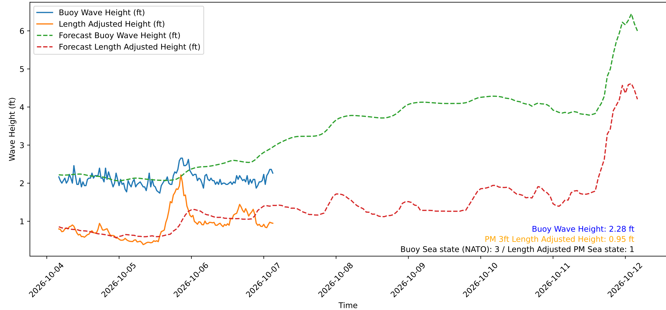
Wave Heights over Time for Red Beach at 2026-10-07 03:40:49
