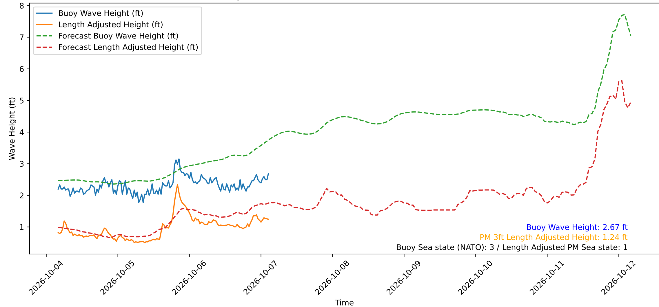
Wave Heights over Time for Green Beach at 2026-10-07 03:41:12
