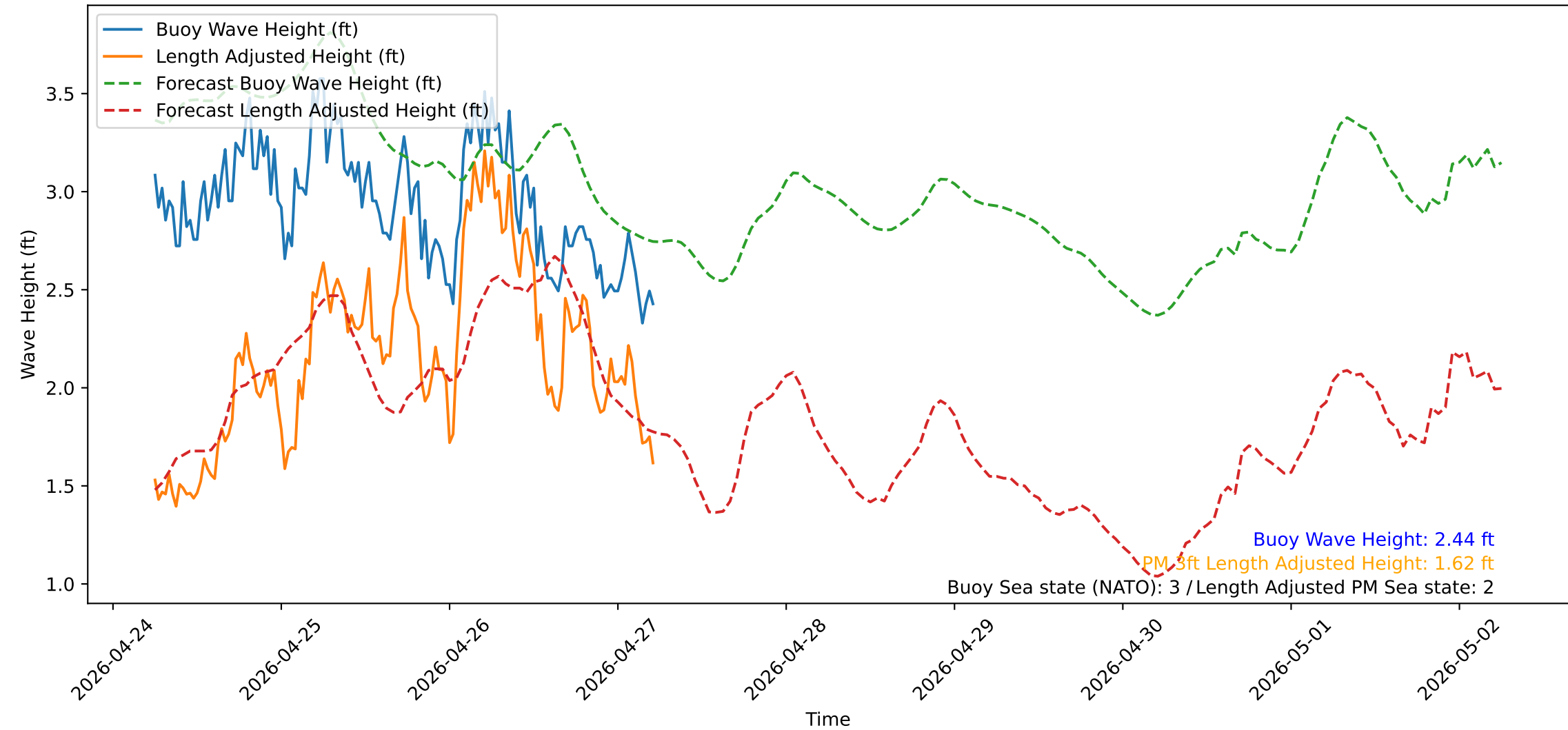
Wave Heights over Time for Green Beach at 2026-04-27 05:51:14
