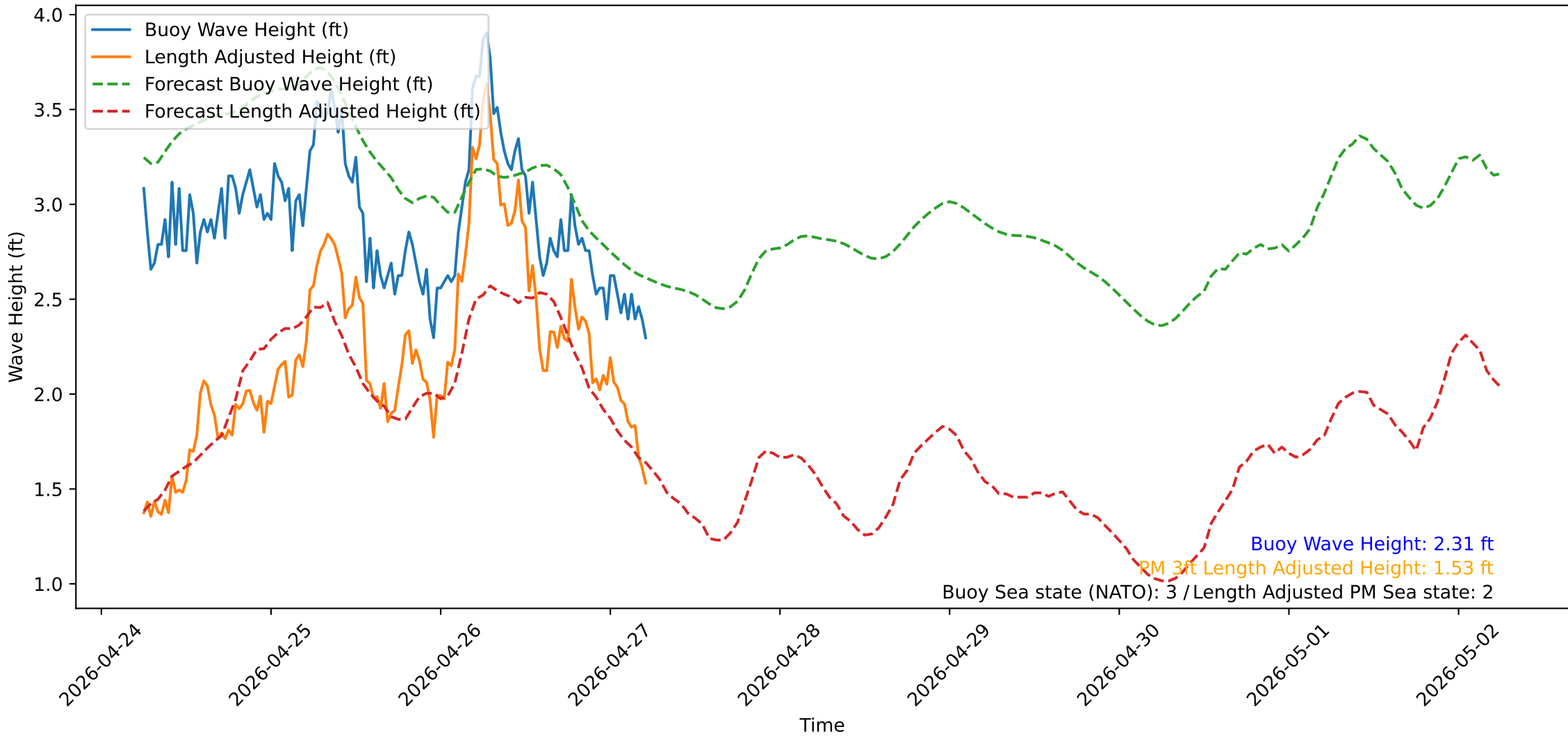
Wave Heights over Time for Oceanside Harbor at 2026-04-27 05:50:31
