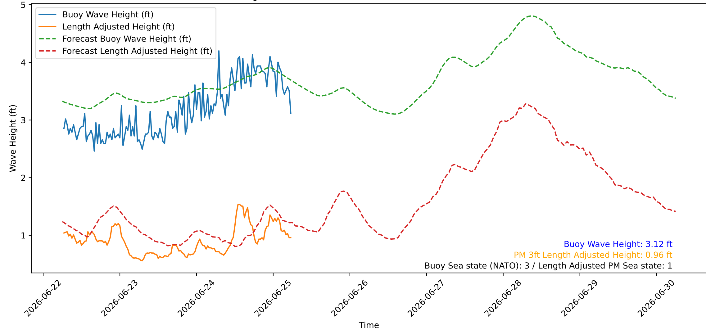
Wave Heights over Time for Green Beach at 2026-06-25 06:21:09
