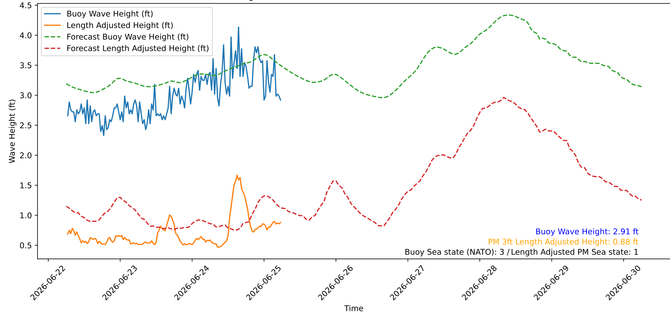
Wave Heights over Time for Red Beach at 2026-06-25 06:20:46
