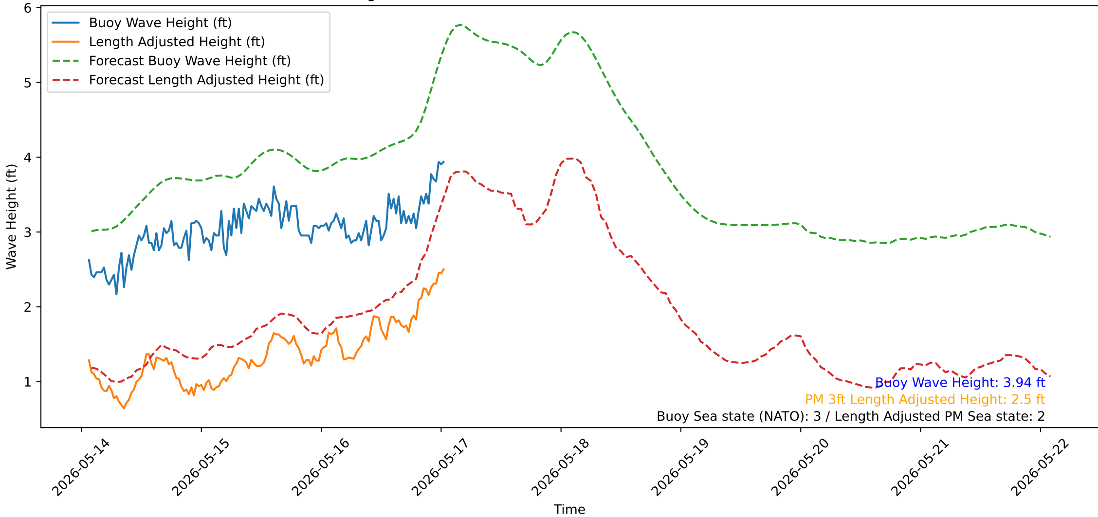
Wave Heights over Time for Oceanside Harbor at 2026-05-17 01:30:31
