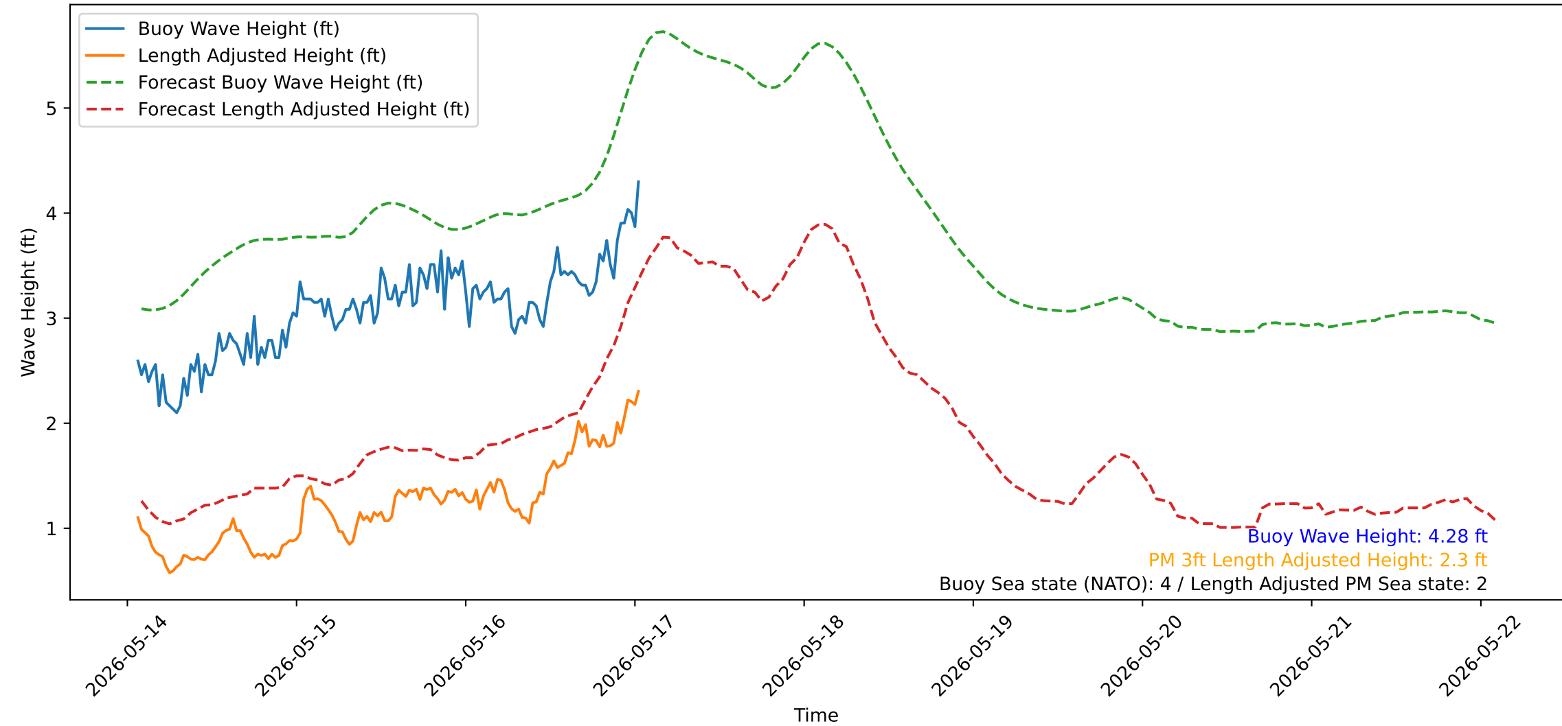
Wave Heights over Time for Green Beach at 2026-05-17 01:31:12
