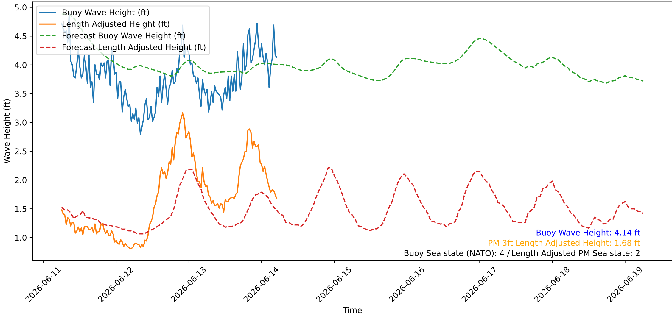
Wave Heights over Time for Oceanside Harbor at 2026-06-14 06:00:26
