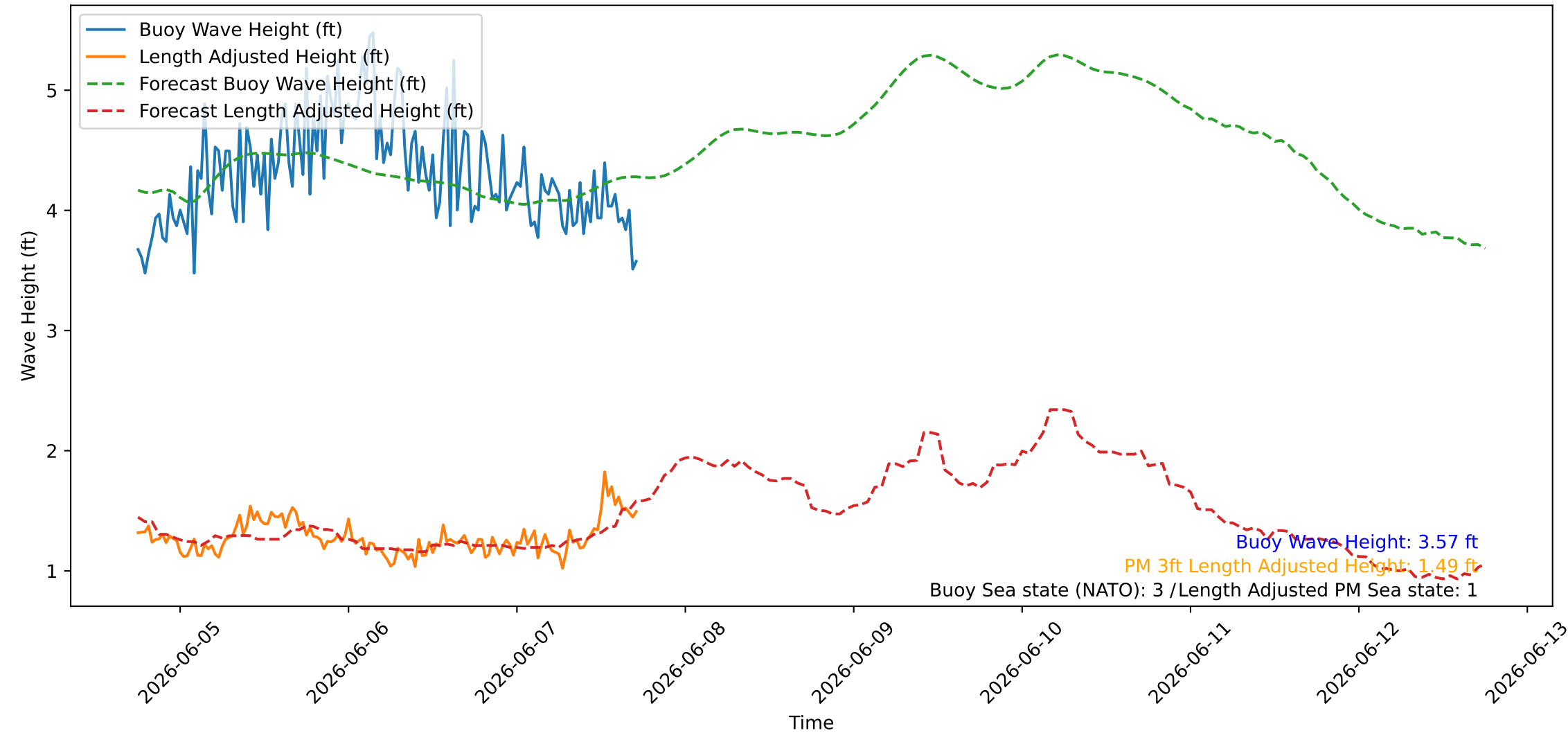
Wave Heights over Time for Oceanside Harbor at 2026-06-07 17:50:25
