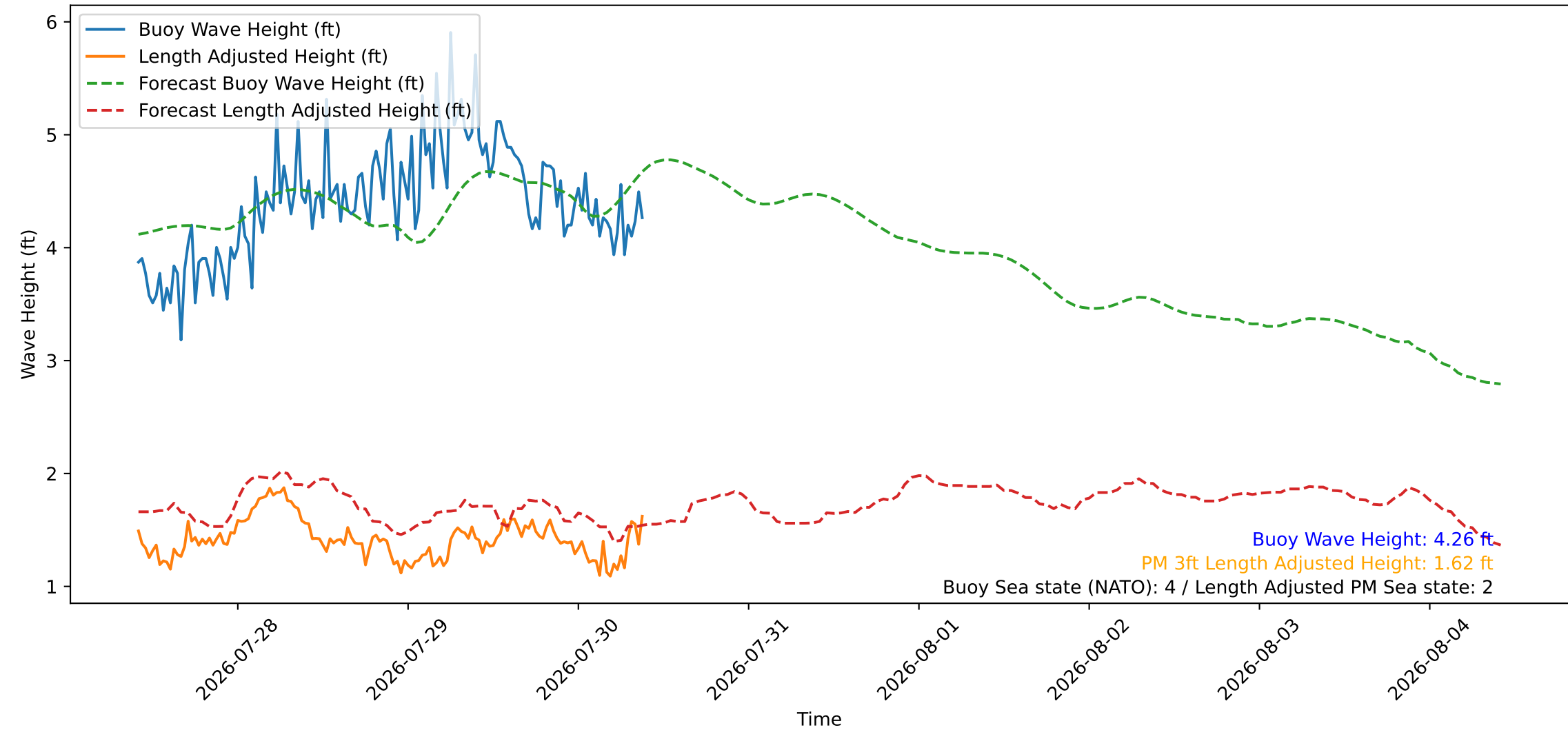
Wave Heights over Time for Oceanside Harbor at 2026-07-30 09:50:27
