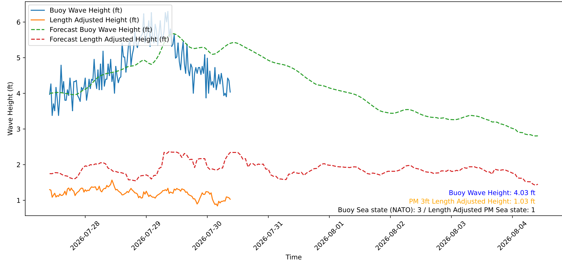
Wave Heights over Time for Green Beach at 2026-07-30 09:51:11
