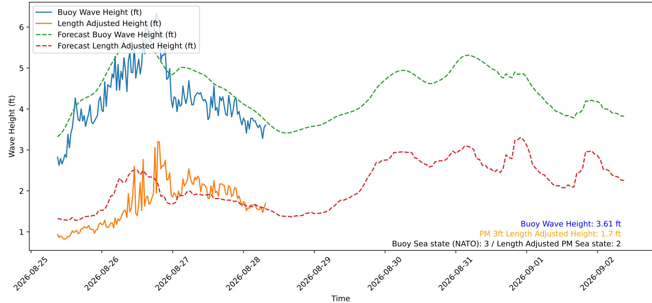
Wave Heights over Time for Green Beach at 2026-08-28 08:31:12
