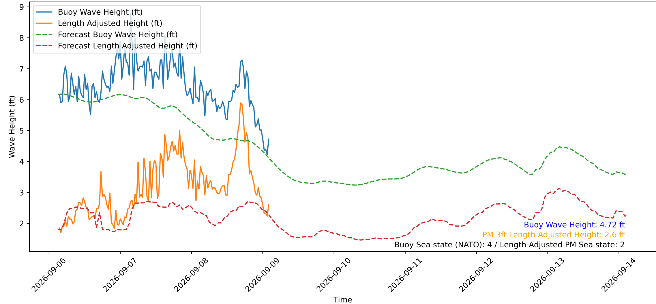
Wave Heights over Time for Green Beach at 2026-09-09 03:01:11
